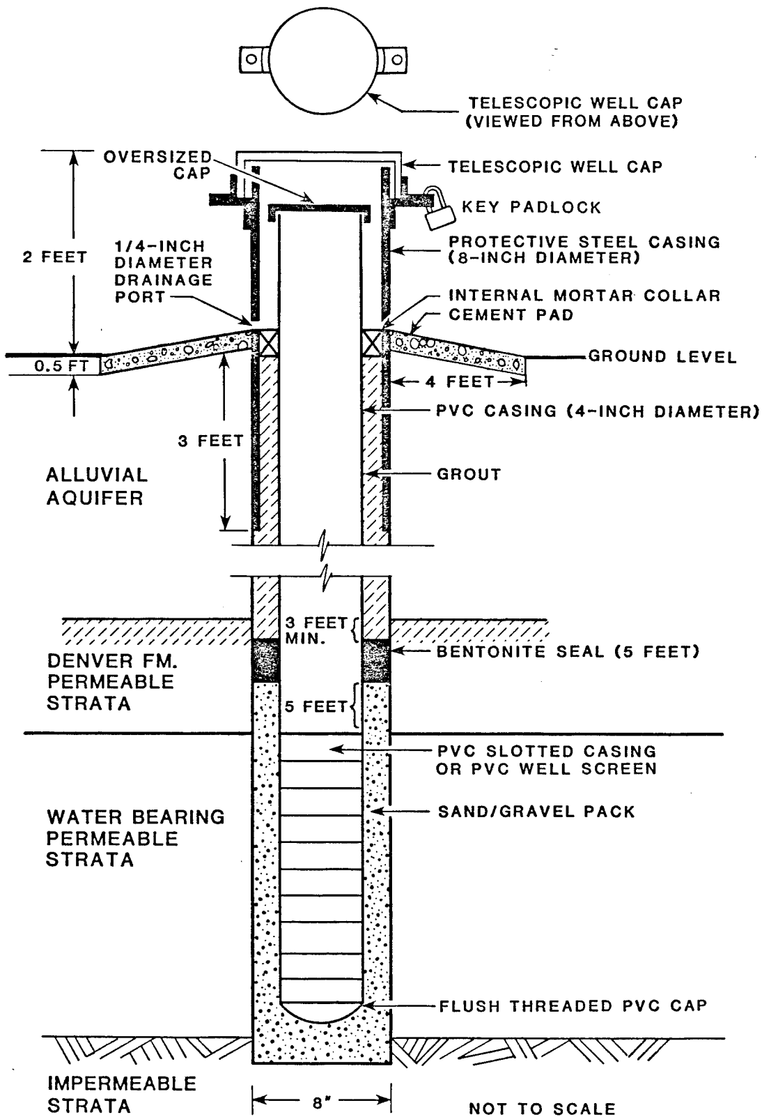
Figure 3.8-2 DEEP (DENVER FORMATION) MONITOR WELL CONSTRUCTION
