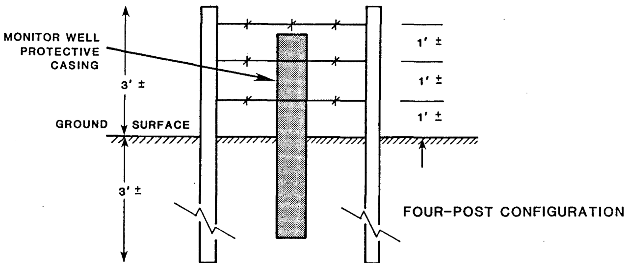
FIGURE 3.8-4 Post Placement Around Wells
