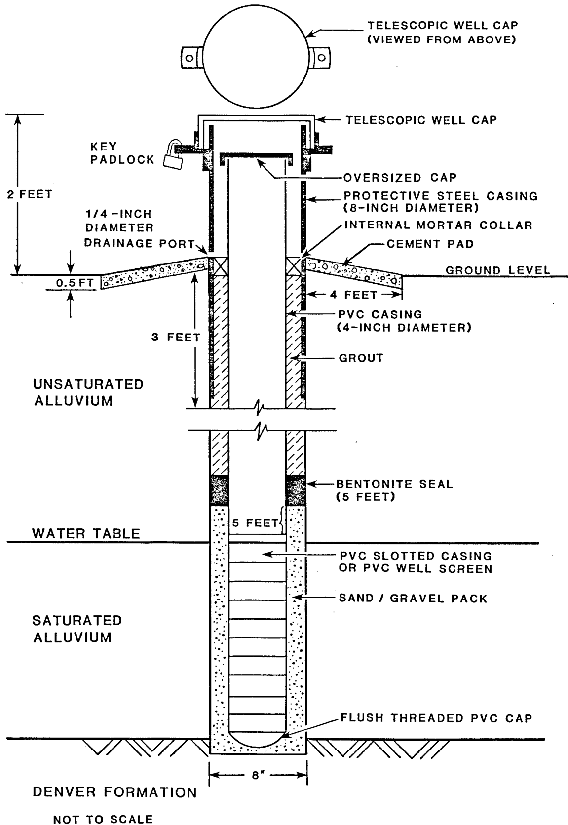
Figure 3.8-1 SHALLOW (ALLUVIAL) MONITOR WELL CONSTRUCTION
