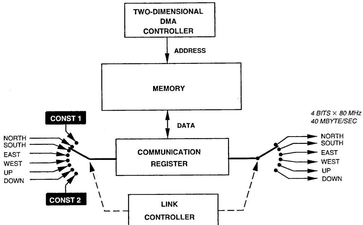
Figure 2-4. CM link.
