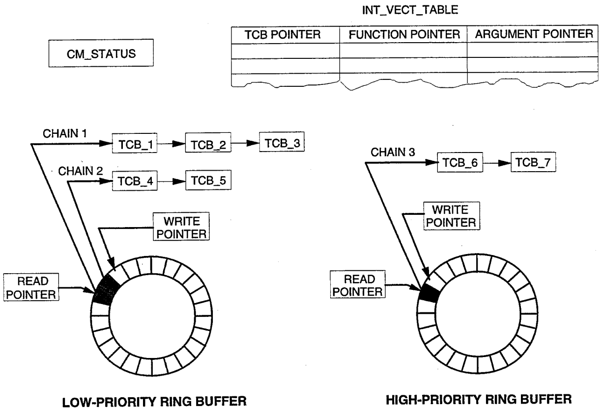
Figure 3-1. CM control system.
