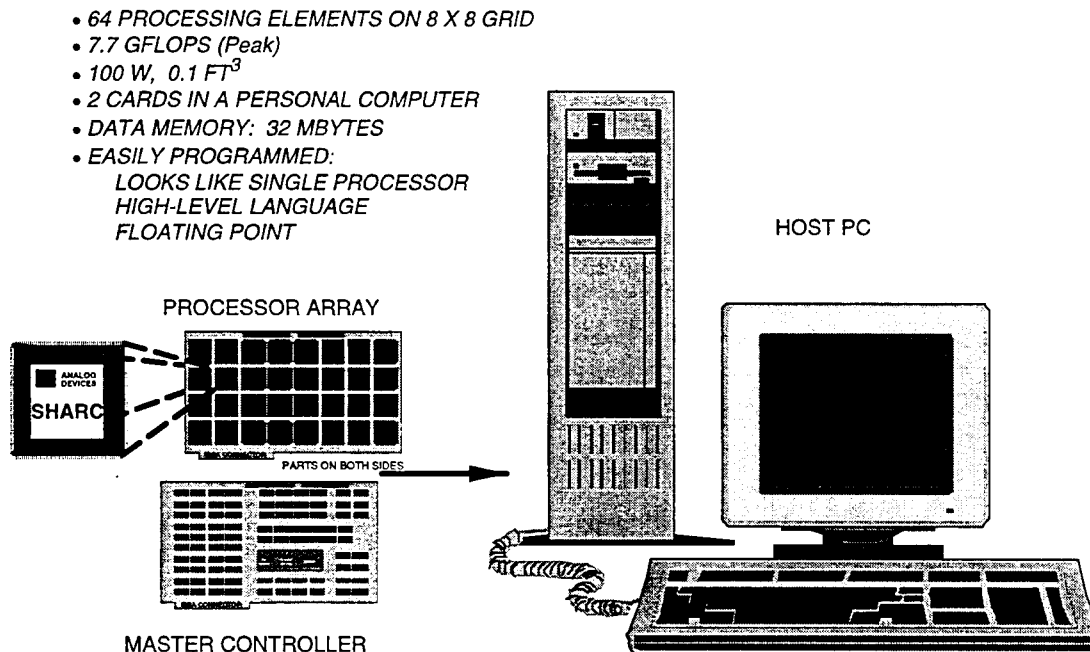
Figure 1-1. MeshSP-1 System.
