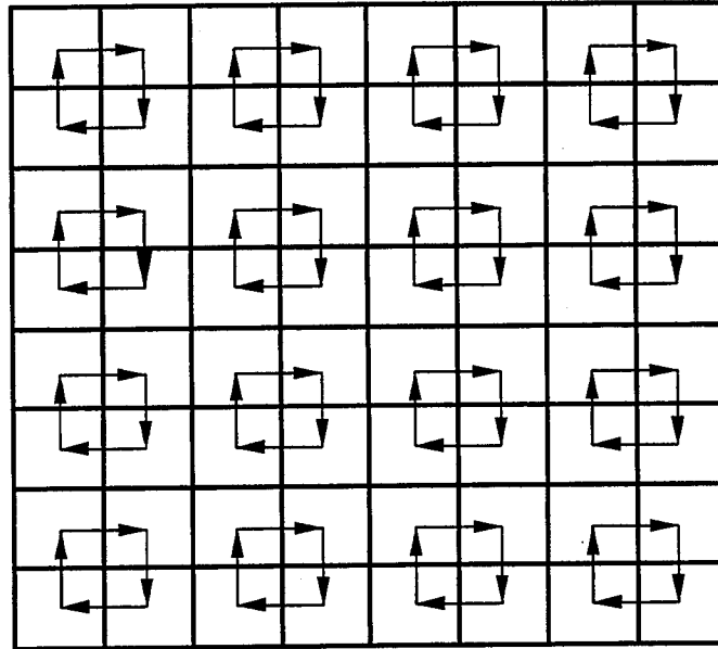
Figure 2-5. A collisionless transfer.
