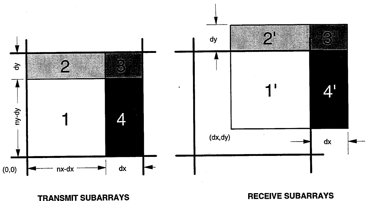
Figure 3-3. Shifting algorithm.
