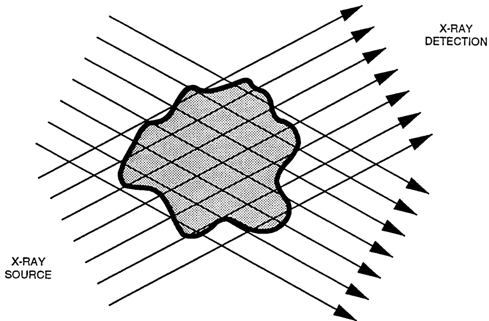
Figure 5-12. CT measurements for two projection angles.
