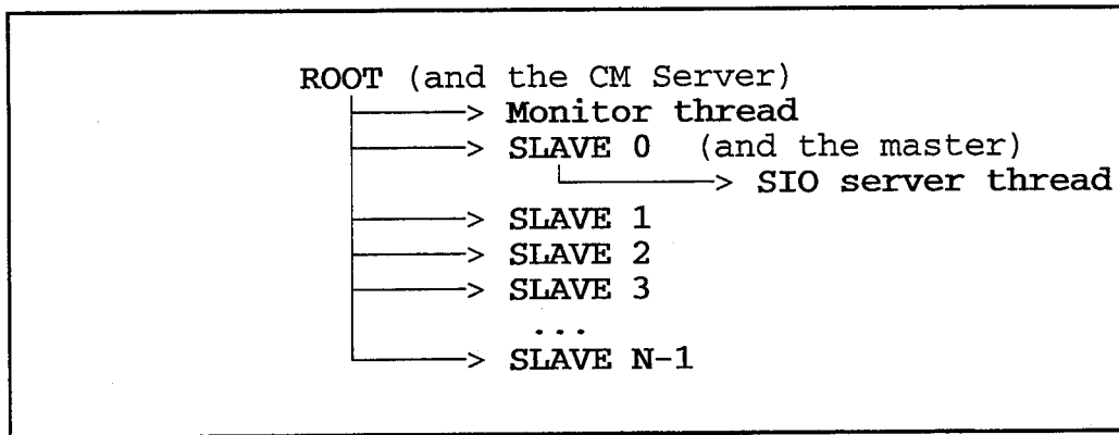
Figure 4-1. Simulator processes and threads.
