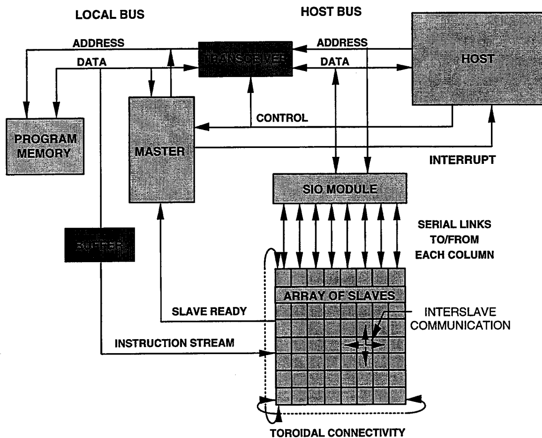
Figure 2-1. MeshSP architecture.
