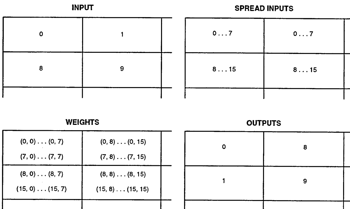
Figure 5-11. Propagation steps.
