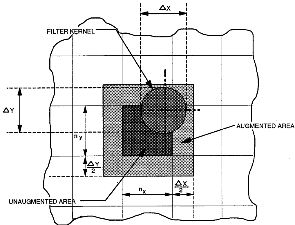
Figure 5-1. Segmented convolution.
