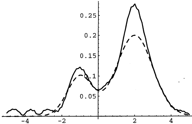
Figure 2: Reconstruction of S(x) = \frac{e^{-(x+1)^2}}{10} + \frac{e^{-(x-2)^2}}{5} .
