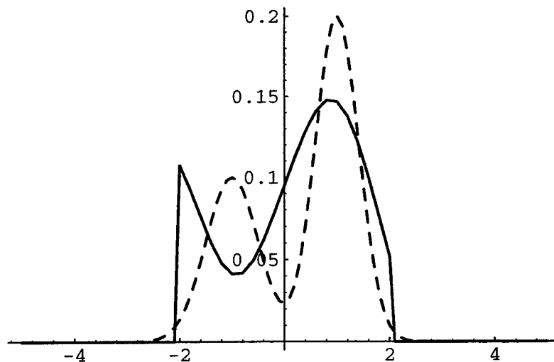
Figure 15: Reconstruction of S(x) for 21 measurements on [-10, 10] , tolerance E = 300 .
