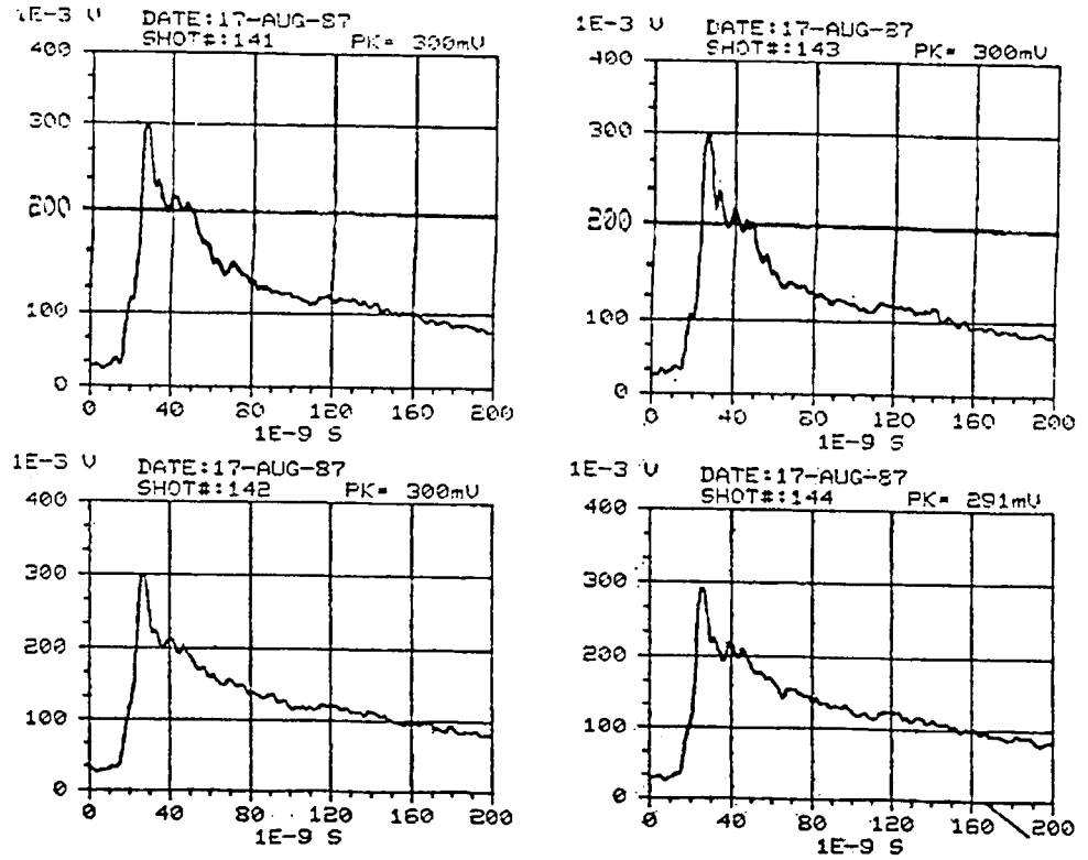
Figure D-25. REPS output waveforms for pulses 141, 142, 143, and 144.
