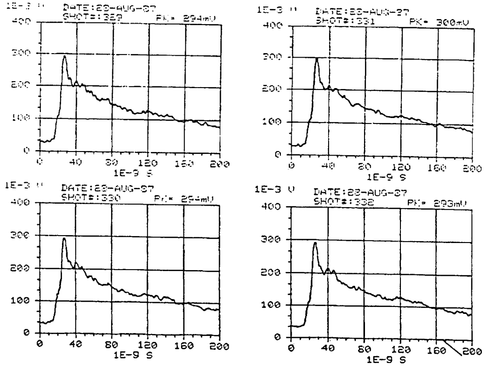
Figure D-61. REPS output waveforms for pulses 329, 330, 331, and 332.
