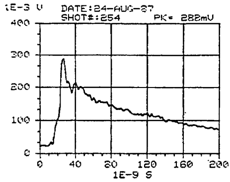
Figure D-47. REPS output waveforms for pulses 254, 255, 256, and 257.
