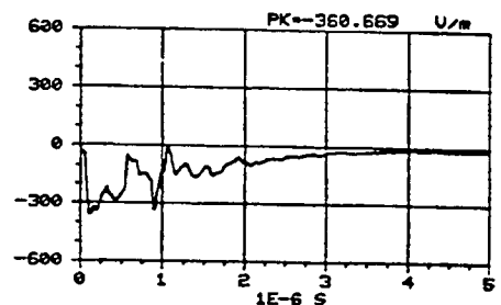
Figure C-190. Z component of the electric field measured at location -25/50/2 using sensor E304-C. REPS pulse 90 generating 6.2 kV/m at 50 m.
