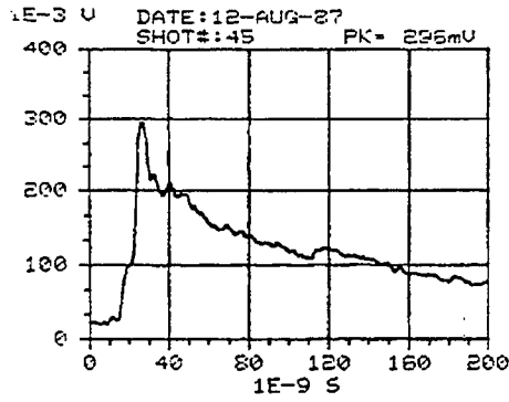
Figure D-7. REPS output waveforms for pulses 45, 46, 47, and 48.
