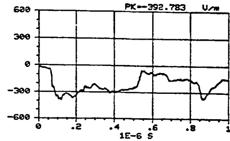
Figure C-189. Z component of the electric field measured at location -25/50/2 using sensor E304-C. REPS pulse 88 generating 6.4 kV/m at 50 m.
