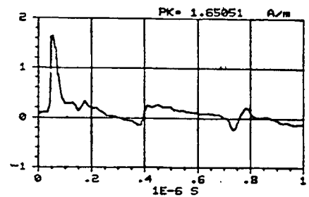
Figure C-230. X component of the magnetic field measured at location 50/50/1 using sensor H104-C. REPS pulse 254 generating 6.1 kV/m at 50 m.
