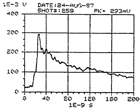
Figure D-48. REPS output waveforms for pulses 259, 260, 261, and 262.
