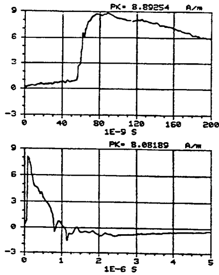
Figure C-23. Y component of the magnetic field measured at location -50/25/1 using sensor H104-C. REPS pulse 237 generating 6.1 kV/m at 50 m.
