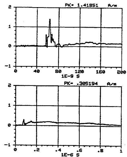
Figure C-148. Z component of the magnetic field measured at location -75/75/1 using sensor H104-C. REPS pulse 151 generating 6.5 kV/m at 50 m.
