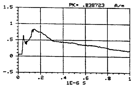
Figure C-101. Z component of the magnetic field measured at location -125/50/1 using sensor H104-C. REPS pulse 212 generating 6.4 kV/m at 50 m.
