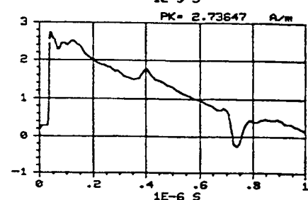
Figure C-232. Y component of the magnetic field measured at location 50/50/1 using sensor H104-C. REPS pulse 256 generating 6.3 kV/m at 50 m.
