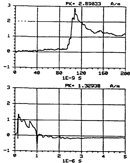
Figure C-120. Y component of the magnetic field measured at location 0/75/1 using sensor H104-C. REPS pulse 133 generating 6.2 kV/m at 50 m.
