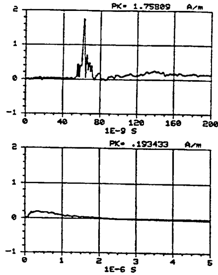
Figure C-149. Z component of the magnetic field measured at location -75/75/1 using sensor H104-C. REPS pulse 152 generating 6.5 kV/m at 50 m.
