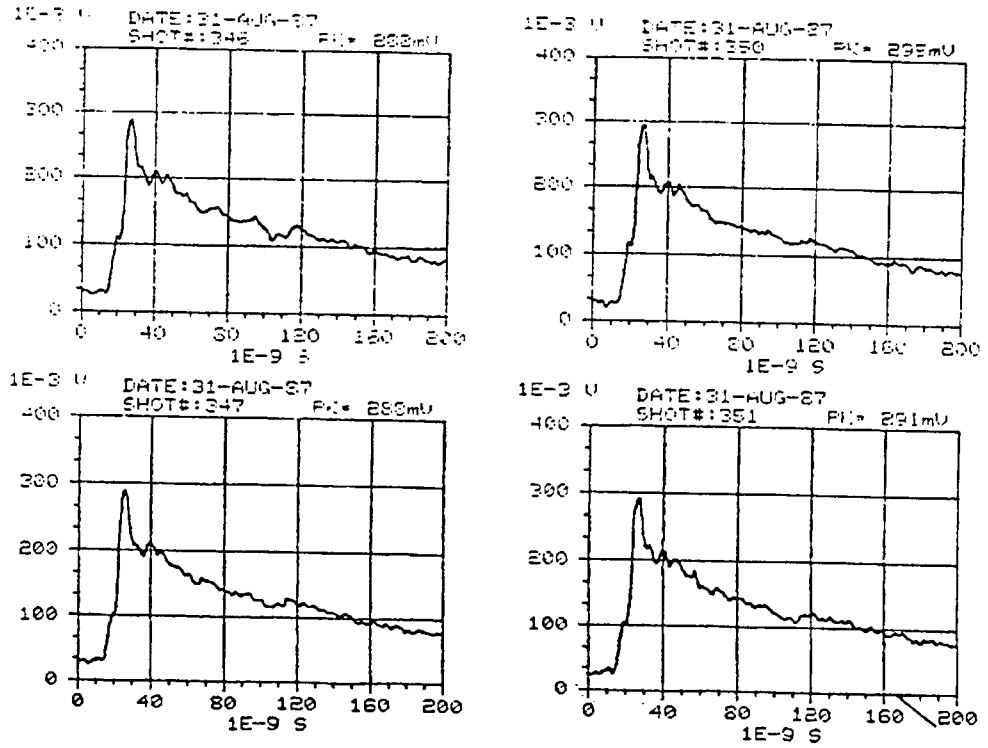
Figure D-65. REPS output waveforms for pulses 346, 347, 350, and 351.
