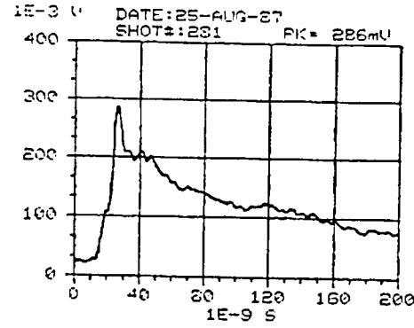
Figure D-53. REPS output waveforms for pulses 281, 283, 284, and 287.
