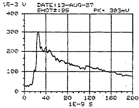
Figure D-15. REPS output waveforms for pulses 95, 96, 97, and 98.
