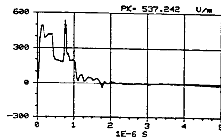
Figure C-229. Z component of the electric field measured at location 50/50/1 using sensor E304-C. REPS pulse 261 generating 6 kV/m at 50 m.
