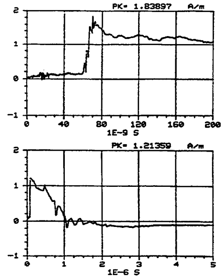
Figure C-138. Y component of the magnetic field measured at location -50/75/1 using sensor H104-C. REPS pulse 113 generating 6.5 kV/m at 50 m.
