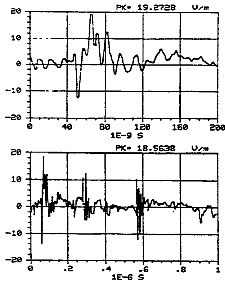
Figure C-115. -Y component of the electric field measured at location 0/75/1 using sensor E201-C. REPS pulse 140 generating 6.3 kV/m at 50 m.
