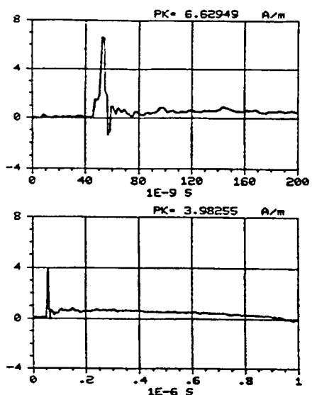
Figure C-56. Z component of the magnetic field measured at location 0/50/1 using sensor H104-C. REPS pulse 16 generating 6.6 kV/m at 50 m.
