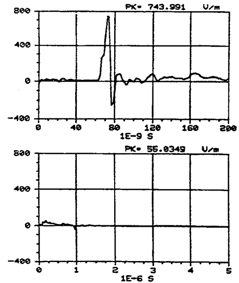
Figure C-114. X component of the electric field measured at location 0/75/1 using sensor E201-C. REPS pulse 142 generating 6.4 kV/m at 50 m.
