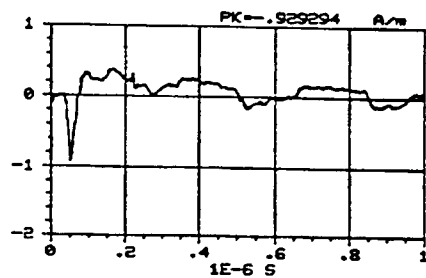
Figure C-191. X component of the magnetic field measured at location -25/50/2 using sensor H104-C. REPS pulse 81 generating 6.3 kV/m at 50 m.
