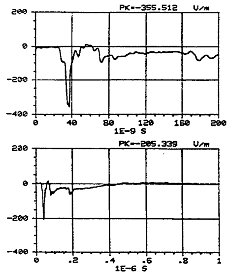
Figure C-84. -Y component of the electric field measured at location -100/50/1 using sensor E201-C. REPS pulse 190 generating 6.3 kV/m at 50 m.
