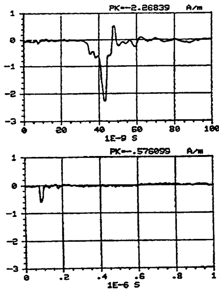
Figure C-283. Z component of the magnetic field measured at location 0/-75/1 using sensor H104-C. REPS pulse 391 generating 6.1 kV/m at 50 m.
