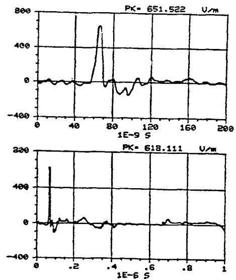
Figure C-168. Z component of the electric field measured at location 0/25/2 using sensor E201-C. REPS pulse 43 generating 6.3 kV/m at 50 m.
