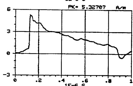
Figure C-262. Y component of the magnetic field measured at location 35/35/1 using sensor H104-C. REPS pulse 276 generating 6.3 kV/m at 50 m.
