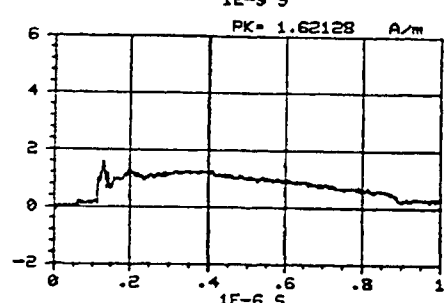
Figure C-264. Z component of the magnetic field measured at location 35/35/1 using sensor H104-C. REPS pulse 374 generating 6.2 kV/m at 50 m.
