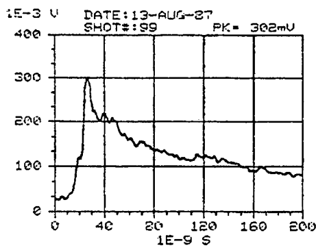
Figure D-16. REPS output waveforms for pulses 99, 101, 103, and 104.
