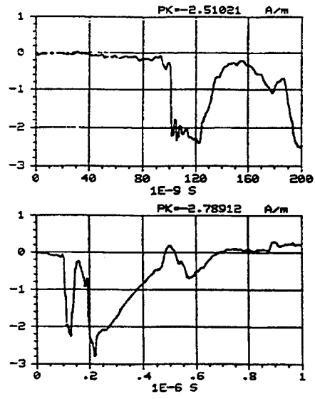
Figure C-42. X component of the magnetic field measured at location -100/25/1 using sensor H104-C. REPS pulse 196 generating 6.5 kV/m at 50 m.
