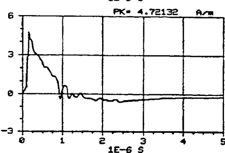
Figure C-263. Y component of the magnetic field measured at location 35/35/1 using sensor H104-C. REPS pulse 377 generating 6.2 kV/m at 50 m.
