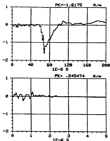
Figure C-62. X component of the magnetic field measured at location -25/50/1 using sensor H104-C. REPS pulse 75 generating 6.3 kV/m at 50 m.
