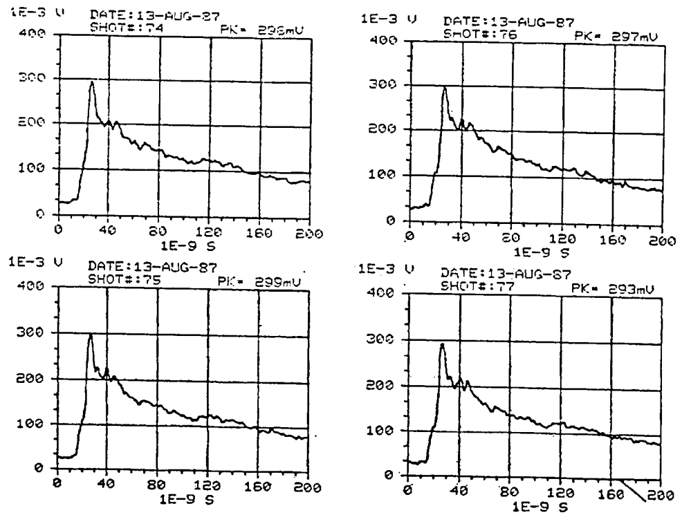
Figure D-10. REPS output waveforms for pulses 74, 75, 76, and 77.
