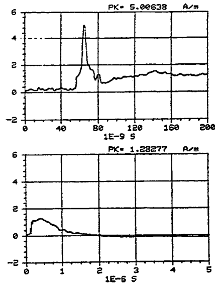
Figure C-265. Z component of the magnetic field measured at location 35/35/1 using sensor H104-C. REPS pulse 375 generating 6 kV/m at 50 m.
