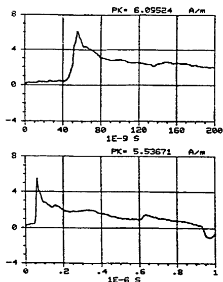
Figure C-54. Y component of the magnetic field measured at location 0/50/1 using sensor H104-C. REPS pulse 13 generating 6.3 kV/m at 50 m.
