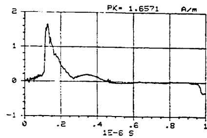
Figure C-245. Z component of the magnetic field measured at location 25/0/1 using sensor H104-C. REPS pulse 396 generating 6.2 kV/m at 50 m.
