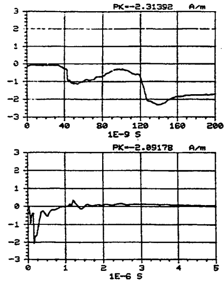
Figure C-98. X component of the magnetic field measured at location -125/50/1 using sensor H104-C. REPS pulse 210 generating 6.4 kV/m at 50 m.
