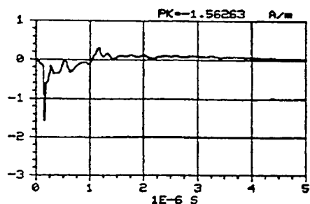
Figure C-261. -X component of the magnetic field measured at location 35/35/1 using sensor H104-C. REPS pulse 373 generating 6.2 kV/m at 50 m.
