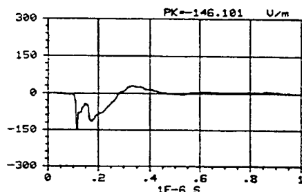
Figure C-104. -Y component of the electric field measured at location -150/50/1 using sensor E201-C. REPS pulse 343 generating 6.2 kV/m at 50 m.
