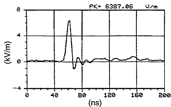
Figure 13. Sample hardcopy of typical waveform collected by IVAN.
