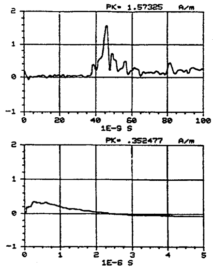
Figure C-92. Z component of the magnetic field measured at location -100/50/1 using sensor H104-C. REPS pulse 184 generating 6.1 kV/m at 50 m.
