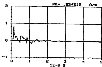
Figure C-231. X component of the magnetic field measured at location 50/50/1 using sensor H104-C. REPS pulse 255 generating 6 kV/m at 50 m.
