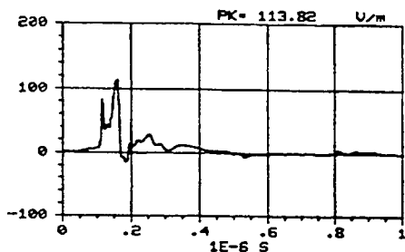
Figure C-103. X component of the electric field measured at location -150/50/1 using sensor E201-C. REPS pulse 340 generating 6.4 kV/m at 50 m.
