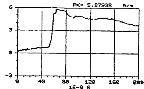
Figure C-261. -X component of the magnetic field measured at location 35/35/1 using sensor H104-C. REPS pulse 373 generating 6.2 kV/m at 50 m.
