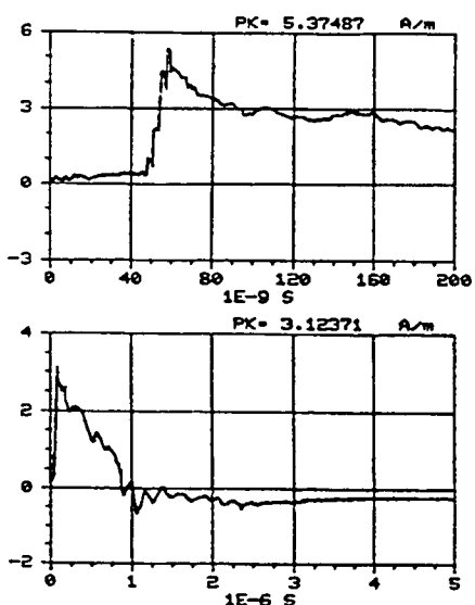
Figure C-64. Y component of the magnetic field measured at location -25/50/1 using sensor H104-C. REPS pulse 74 generating 6.3 kV/m at 50 m.
