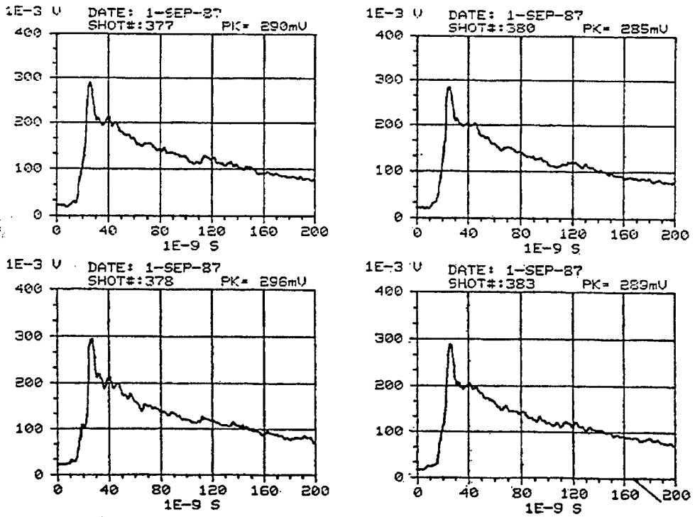
Figure D-72. REPS output waveforms for pulses 377, 378, 380, and 383.
