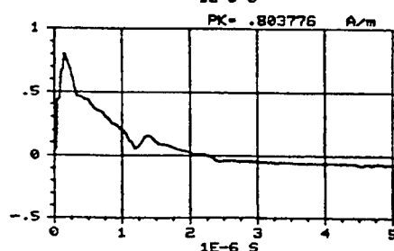
Figure C-102. Z component of the magnetic field measured at location -125/50/1 using sensor H104-C. REPS pulse 213 generating 6.2 kV/m at 50 m.
