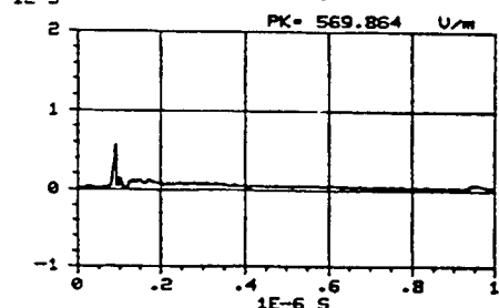
Figure C-248. -Y component of the electric field measured at location 18/33/1 using sensor E304-C. REPS pulse 360 generating 6.2 kV/m at 50 m.
