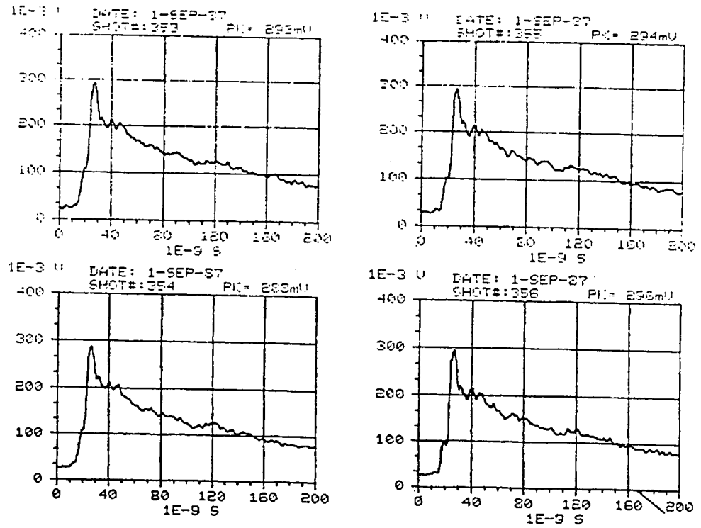
Figure D-66. REPS output waveforms for pulses 353, 354, 355, and 356.
