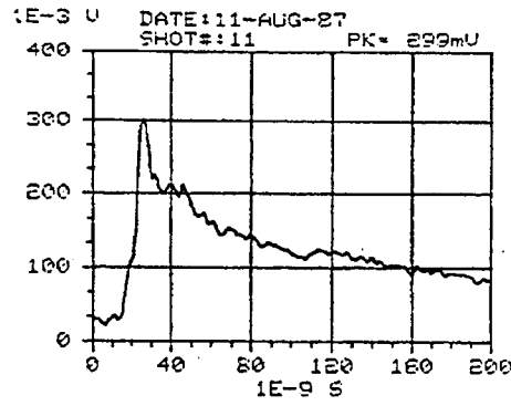
Figure D-3. REPS output waveforms for pulses 11, 13, 14, and 15.
