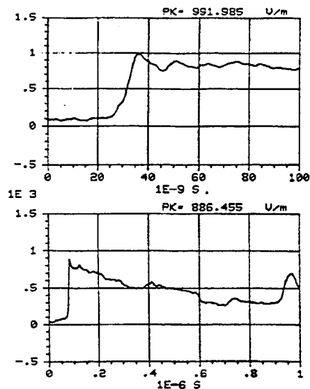
Figure C-249. Z component of the electric field measured at location 18/33/1 using sensor E304-C. REPS pulse 358 generating 6.1 kV/m at 50 m.
