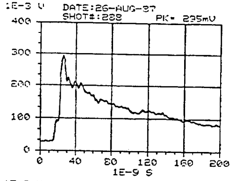
Figure D-54. REPS output waveforms for pulses 288, 289, 292, and 293.
