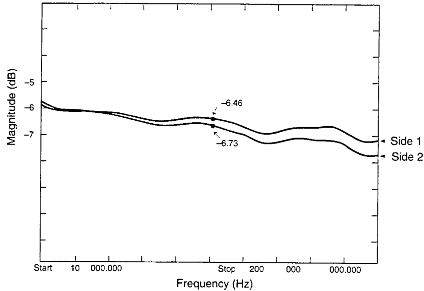
Figure A-3. Frequency response of balun and cable loss.
