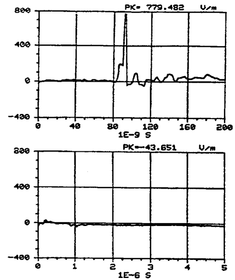
Figure C-122. X component of the electric field measured at location -25/75/1 using sensor E201-C. REPS pulse 124 generating 6.6 kV/m at 50 m.
