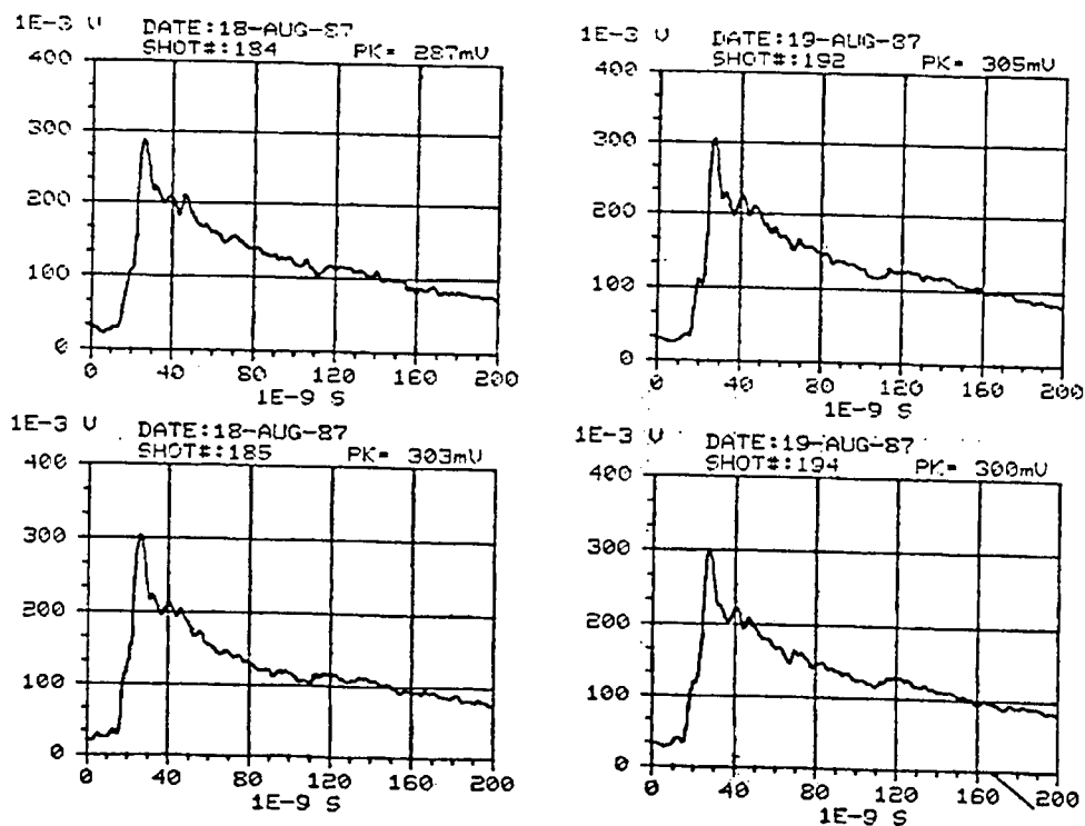
Figure D-34. REPS output waveforms for pulses 184, 185, 192, and 194.
