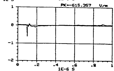
Figure C-216. -X component of the electric field measured at location 25/50/1 using sensor E201-C. REPS pulse 339 generating 6.3 kV/m at 50 m.
