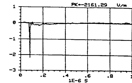
Figure C-247. -X component of the electric field measured at location 18/33/1 using sensor E304-C. REPS pulse 357 generating 6.2 kV/m at 50 m.
