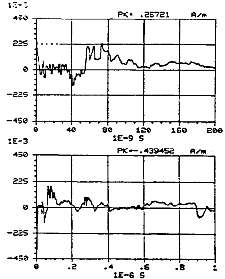
Figure C-118. X component of the magnetic field measured at location 0/75/1 using sensor H104-C. REPS pulse 135 generating 6.2 kV/m at 50 m.
