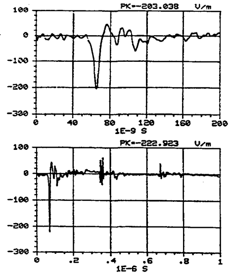
Figure C-2. -Y component of the electric field measured at location 0/25/1 using sensor E201-C. REPS pulse 39 generating 6.1 kV/m at 50 m.
