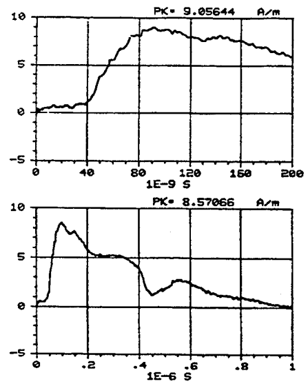
Figure C-44. Y component of the magnetic field measured at location -100/25/1 using sensor H104-C. REPS pulse 200 generating 6.4 kV/m at 50 m.
