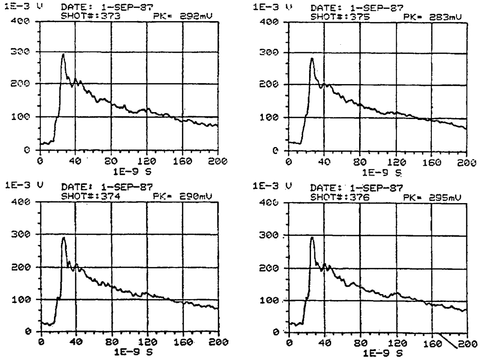
Figure D-71. REPS output waveforms for pulses 373, 374, 375, and 376.
