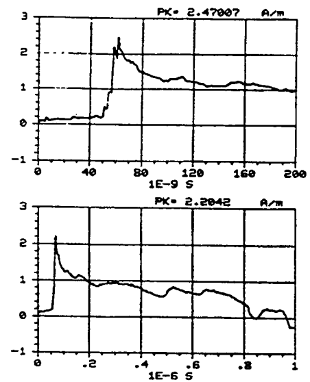
Figure C-128. Y component of the magnetic field measured at location -25/75/1 using sensor H104-C. REPS pulse 126 generating 6.3 kV/m at 50 m.
