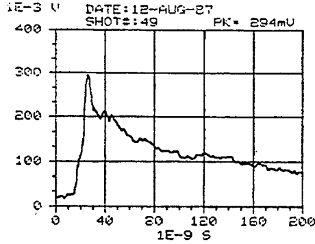
Figure D-8. REPS output waveforms for pulses 49, 52, 53, and 54.
