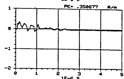
Figure C-192. X component of the magnetic field measured at location -25/50/2 using sensor H104-C. REPS pulse 82 generating 6.5 kV/m at 50 m.
