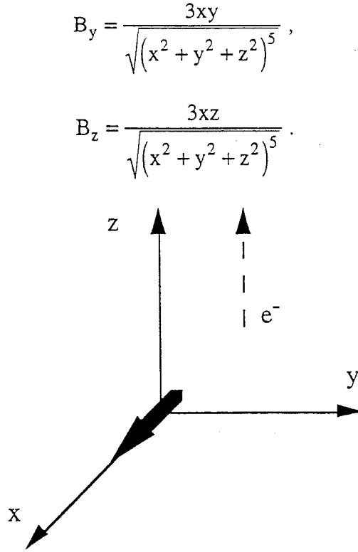
Figure 5.6 Geometry of the calculated magnetic dipole fields.
