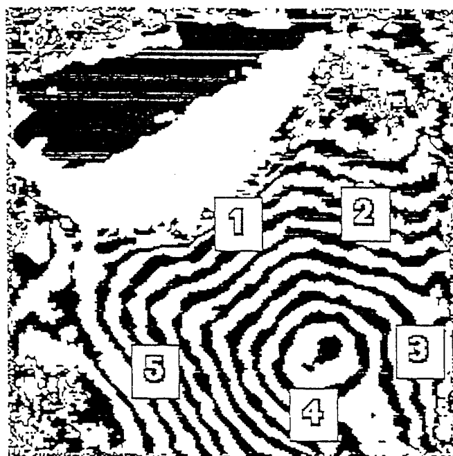
Fig. 2a. Phase image of Co/Cu multilayer acquired in absolute mode of STEM holography ( 1.4\mu\text{m} \times 1.4\mu\text{m} ).
