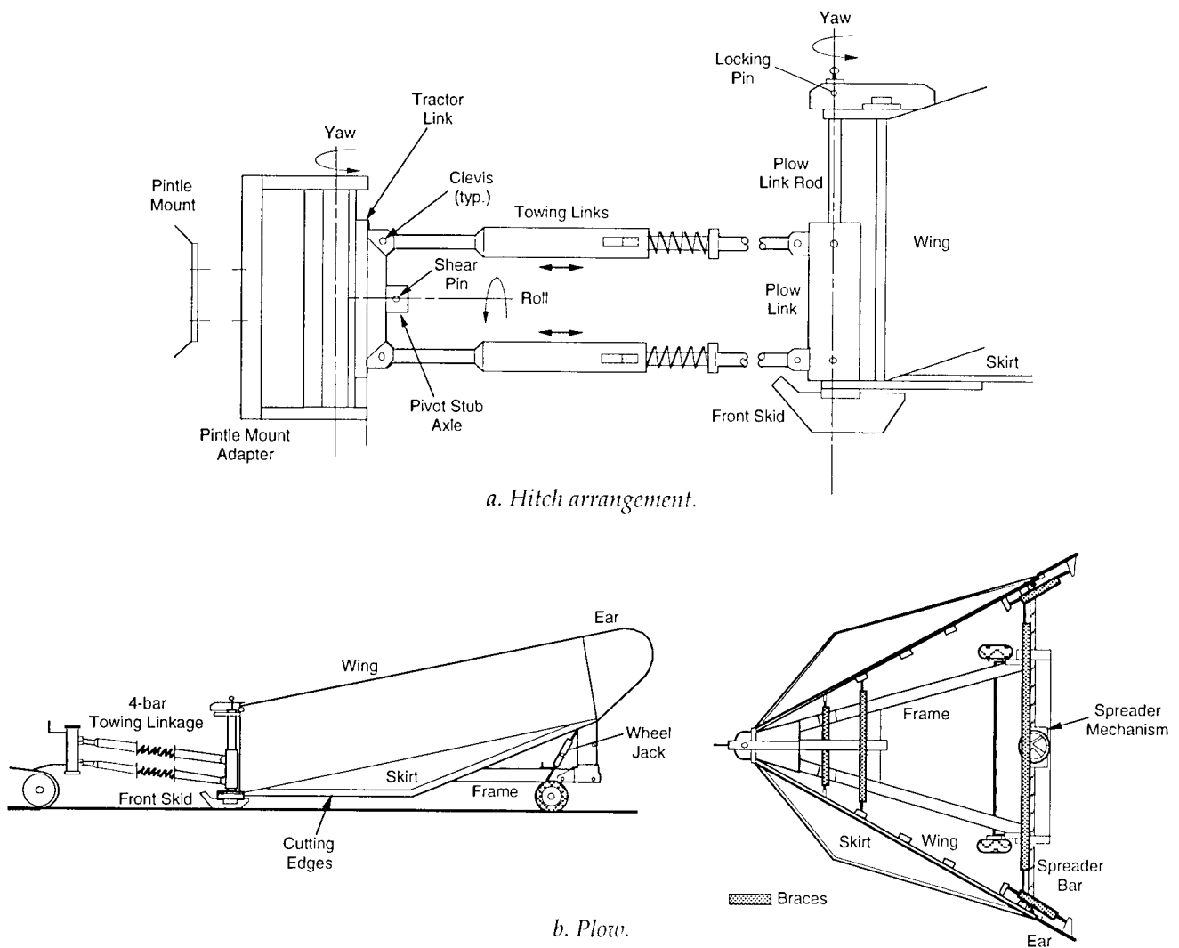
Figure 2. Schematic of plow and hitch.
