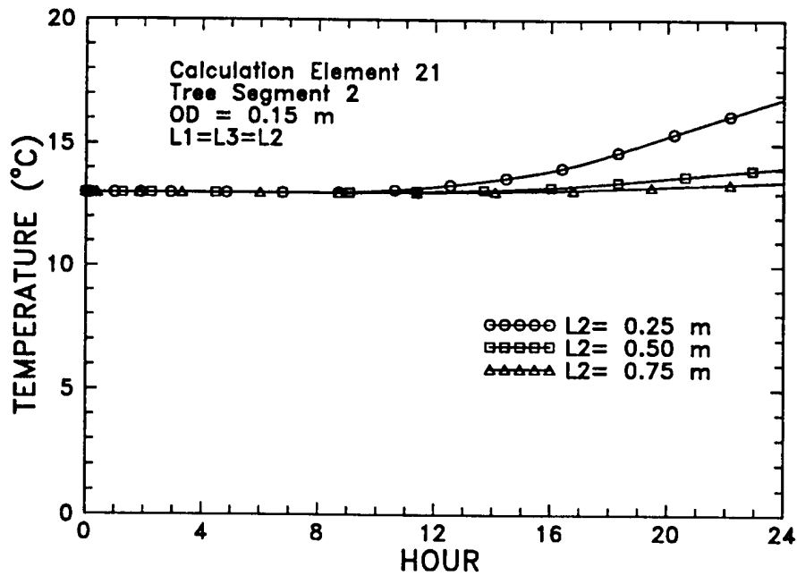
Figure 26. Temperature of Element 21 (OD = 0.15 m) as a Function of Time for Three Different Segment Lengths
