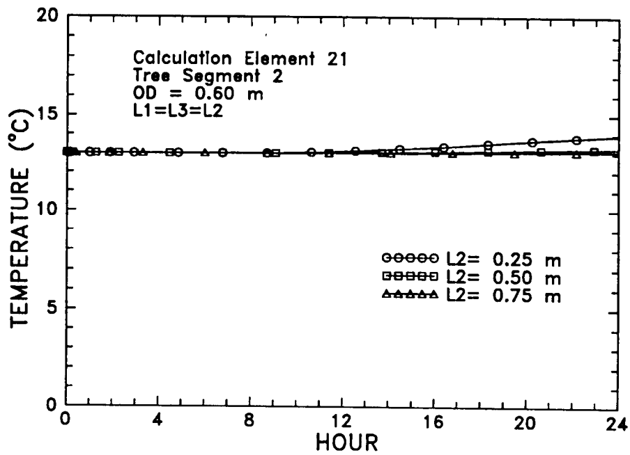
Figure 30. Temperature of Element 21 (OD = 0.6 m) as a Function of Time for Three Different Segment Lengths
