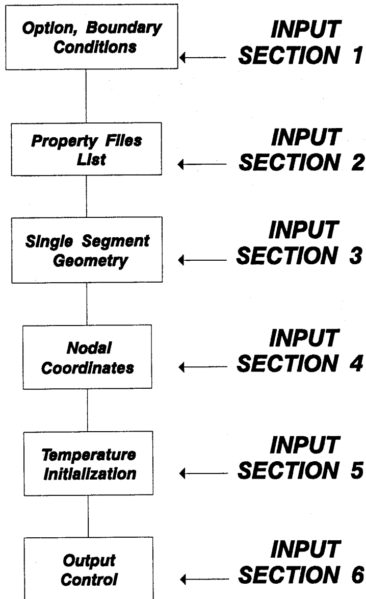
Figure 5. Input Requirements When Specifying the Single Tree Segment Option
