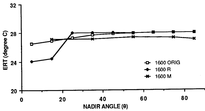
Figure 7. ORIG and ROUGH (R) model predictions and average measurements (M) for Day 235.
