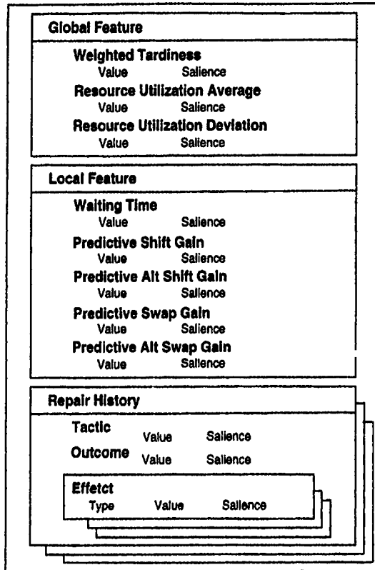
Figure 4: Case Representation
