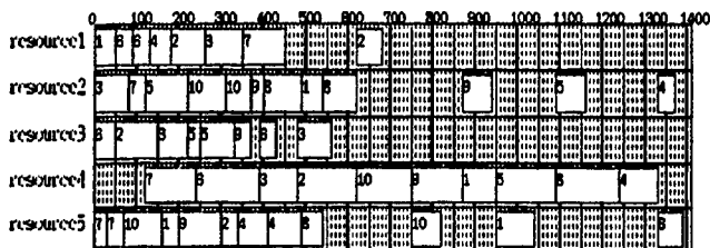
Figure 8: Schedule Result after Repair on A_4^6
