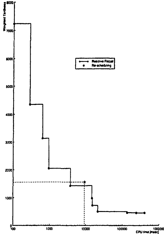
Figure 13 Repair Responsiveness of CABINS in Problem 1
