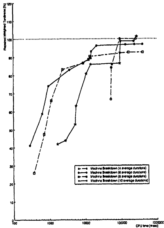
Figure 14: Repair Ratio
