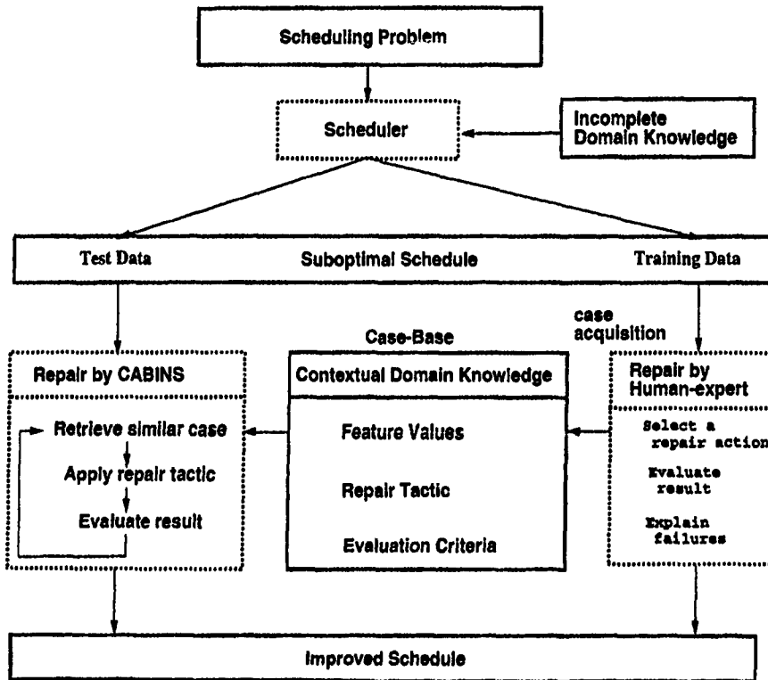
Figure 3. CABINS Architecture
