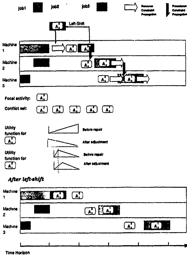
Figure 6 Example of repair tactic application: left-shift
