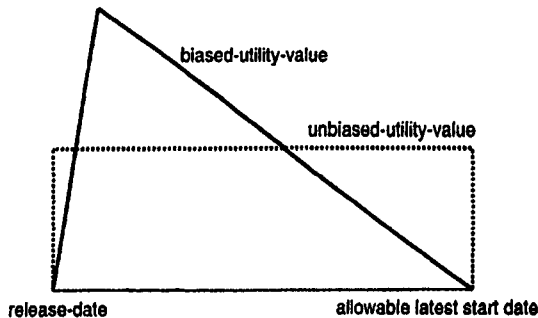
Figure 2: Utility-Functions
