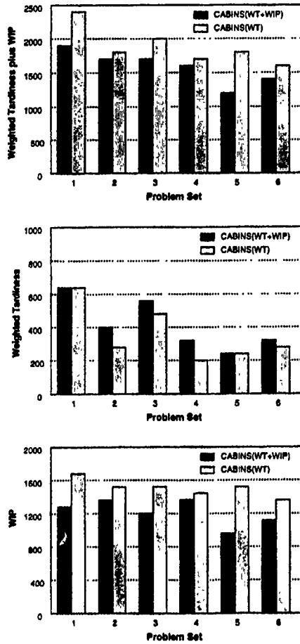
Figure 9: Scheduling Results with Different Case Bases
