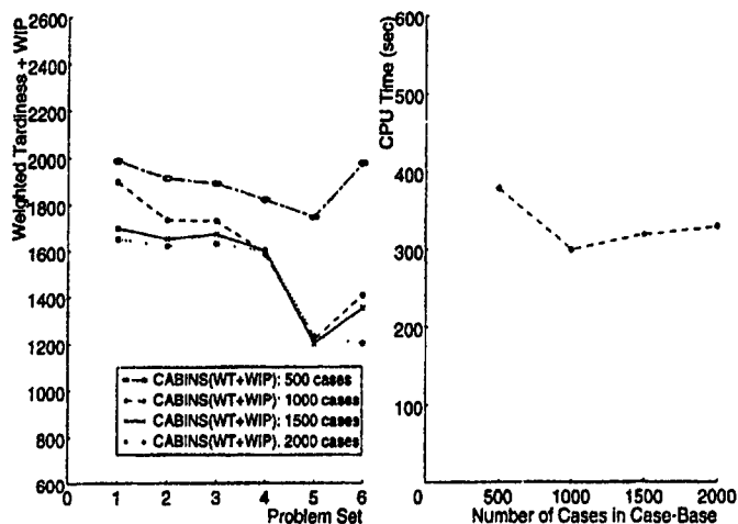
Figure 15: Effect of case-base sizes in quality and efficiency
