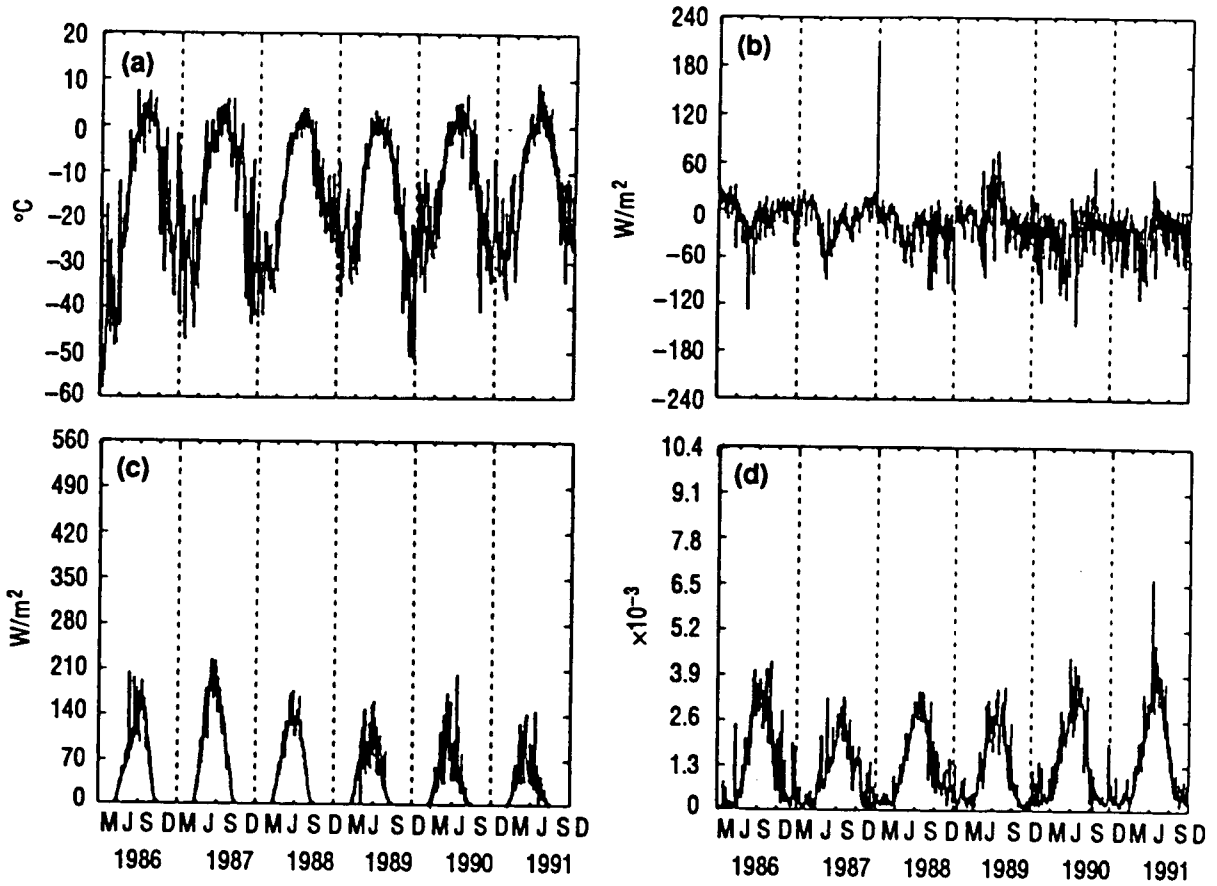
Fig. 8 — Areal-averaged input fields from NOGAPS at 6-hour intervals. All data are for the central Arctic region. (a) Air temperature, (b) longwave radiation, (c) solar radiation, and (d) specific humidity.
