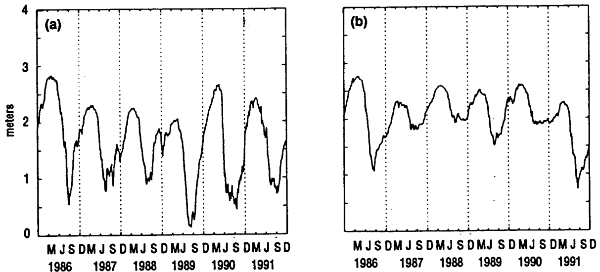
Fig. 10 — Model output areal-averaged ice thickness (meters) for (a) Beaufort and (b) central Arctic
