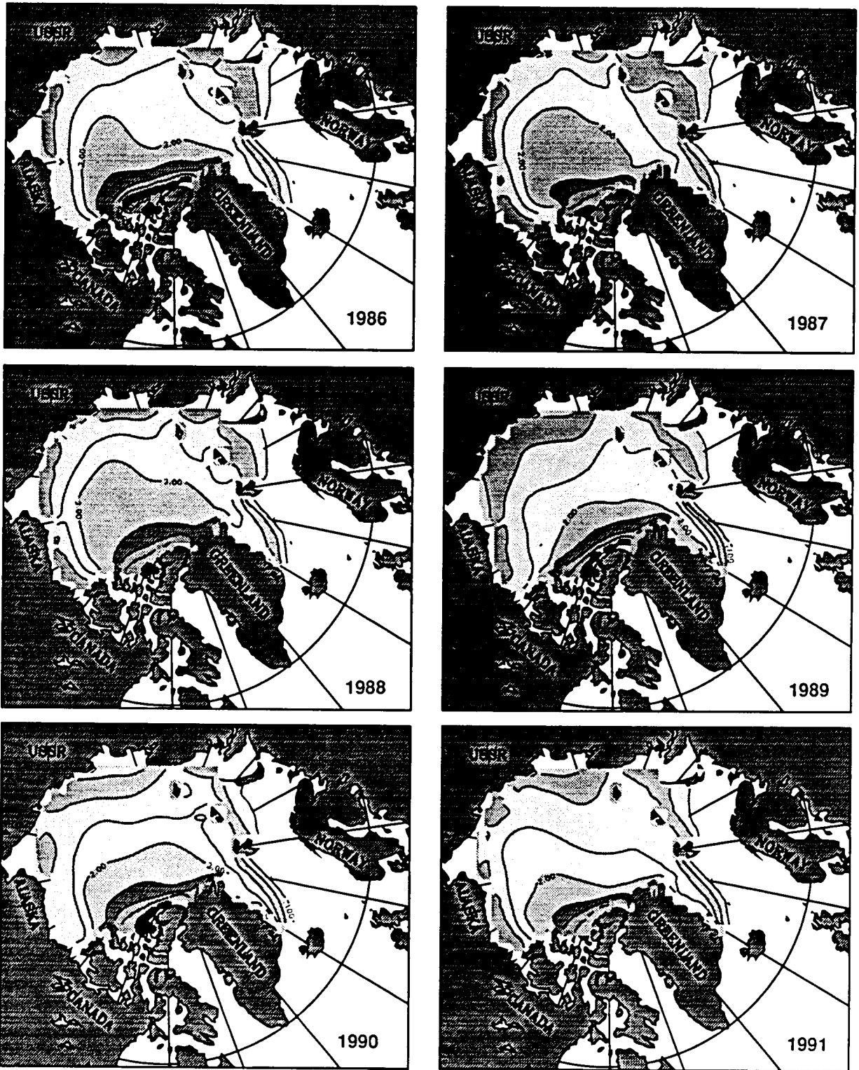
Fig. 6 — Annual mean model derived ice thickness. Ice edge is denoted by the 0.1-m contour. Contour interval is 0.5 m for other contours.
