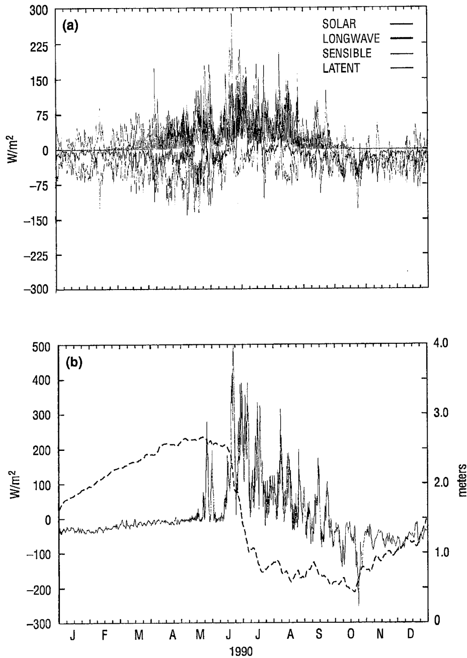
Fig. 13 — (a) Surface forcing terms from Eqs. 5–8 for 1990, Beaufort region, (b) solid line is the sum of the four forcing terms shown in (a); dotted line is the areal-averaged ice thickness in meters for the Beaufort region
