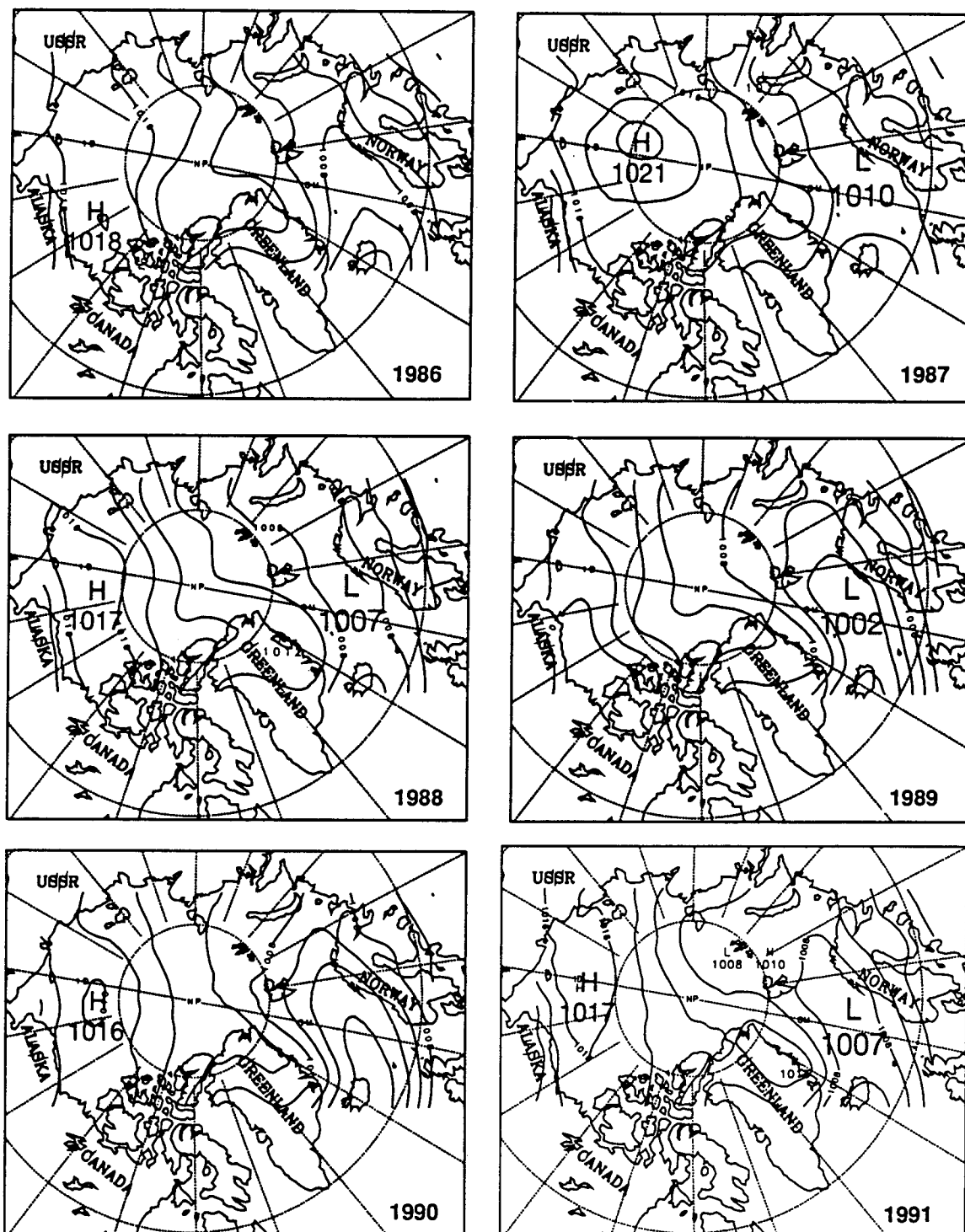
Fig. 2 — Annual mean air pressures from NOGAPS. Contour interval is 2 mb.
