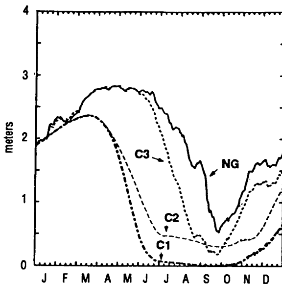
Fig. 17 — Ice thickness for the three climatological test cases and model runs with NOGAPS 1986 data for the Beaufort region.
