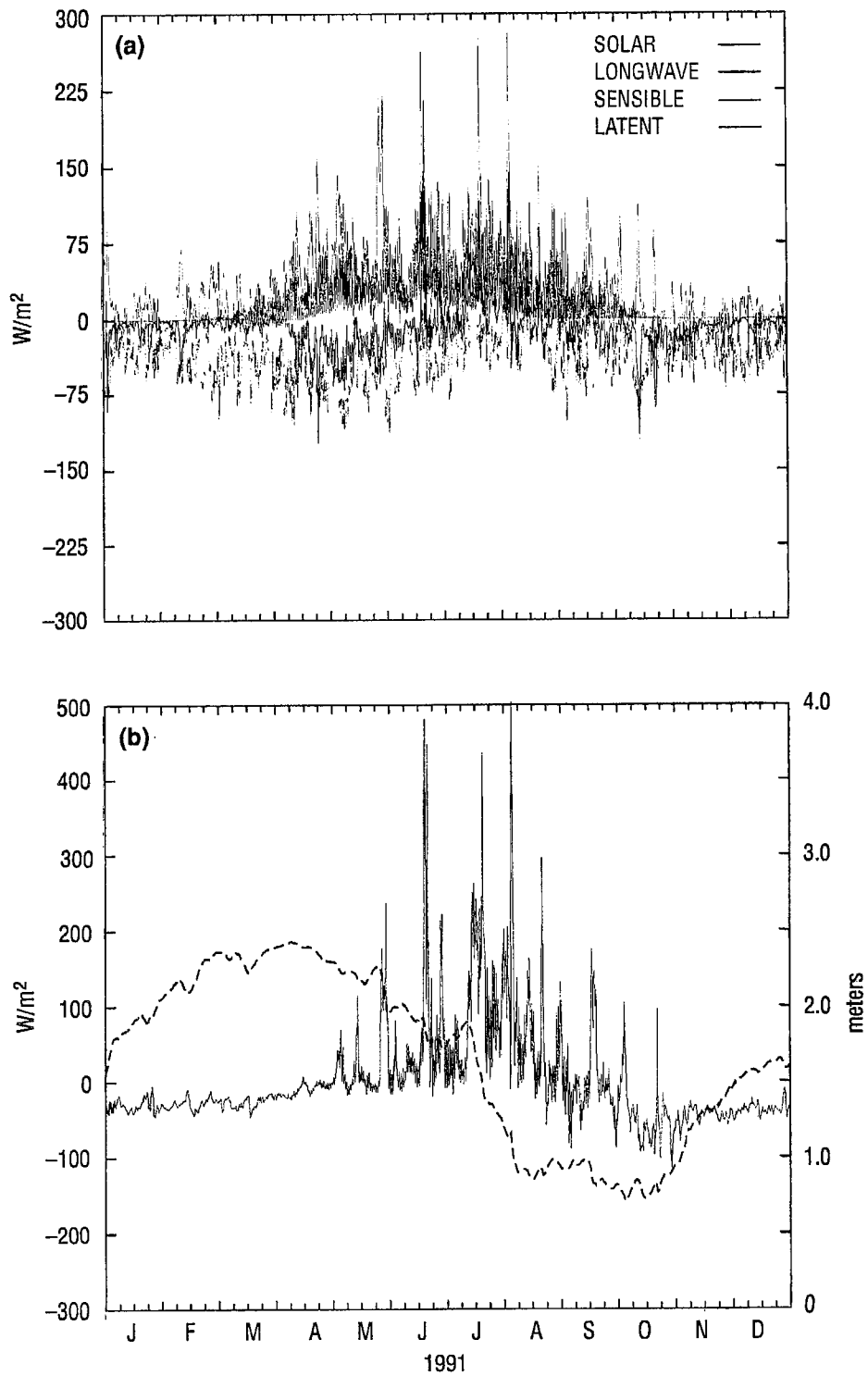
Fig. 14 — (a) Surface forcing terms from Eqs. 5–8 for 1991, Beaufort region, (b) solid line is the sum of the four forcing terms shown in (a); dotted line is the areal-averaged ice thickness in meters for the Beaufort region
