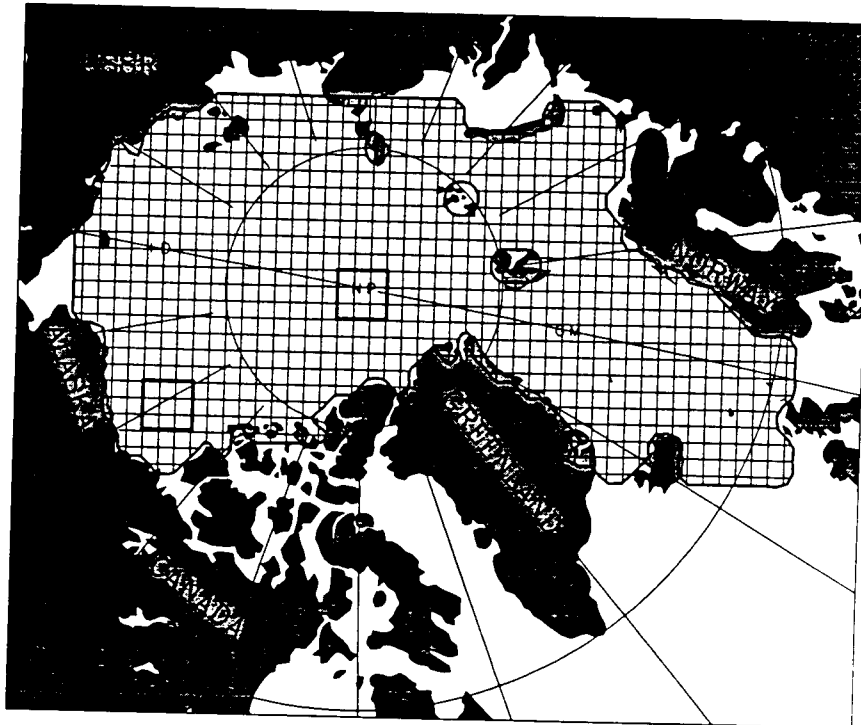
Fig. 1 — The 47 \times 25 horizontal model grid. Boxes depict Beaufort Sea and central Arctic regions used in later discussions.
