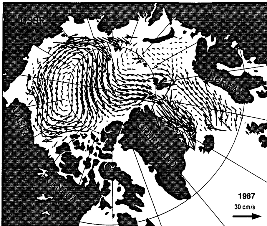
Fig. 5 — Annual mean model-derived ocean currents at level 1. Maximum vector is 30 cm/s.
