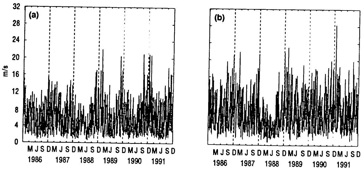
Fig. 9 — Areal-averaged wind speeds from NOGAPS at 6-hour intervals for (a) Beaufort region and (b) central Arctic region
