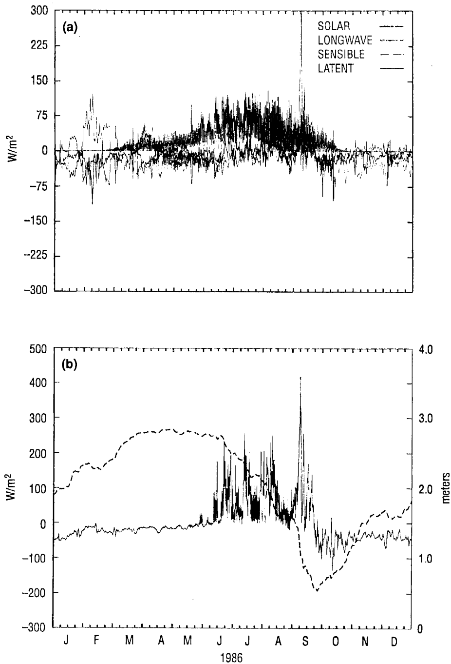
Fig. 12 — (a) Surface forcing terms from Eqs. 5–8 for 1986, Beaufort region, (b) solid line is the sum of the four forcing terms shown in (a); dotted line is the areal-averaged ice thickness in meters for the Beaufort region
