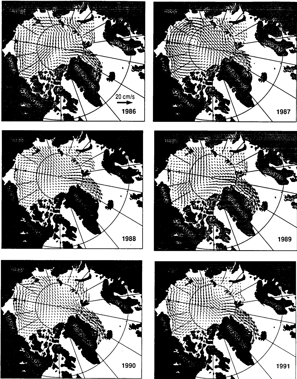
Fig. 4 — Annual mean model-derived ice drift. Maximum vector is 20 cm/s.
