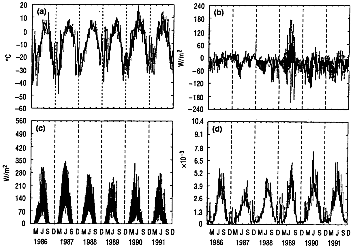
Fig. 7 — Areal-averaged input fields from NOGAPS at 6-hour intervals. All data are for the Beaufort region. (a) Air temperature, (b) longwave radiation, (c) solar radiation, and (d) specific humidity.
