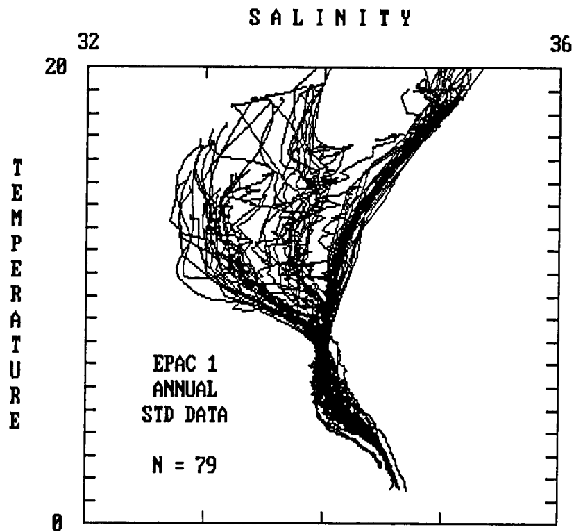
Figure 10. Plot of temperature versus salinity over the full depth spectrum.
