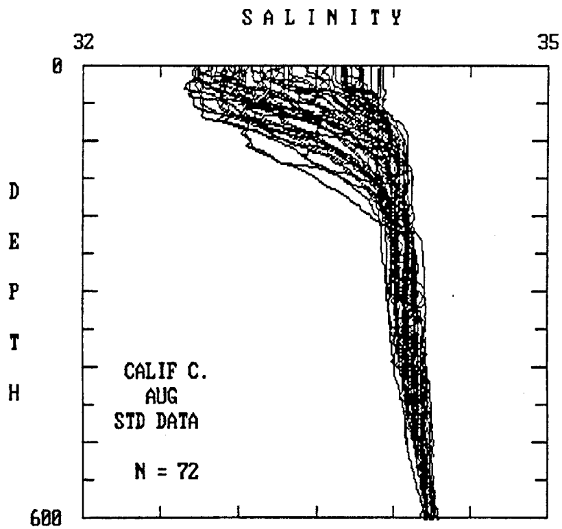
Figure 8. Plot of salinity versus depth.
