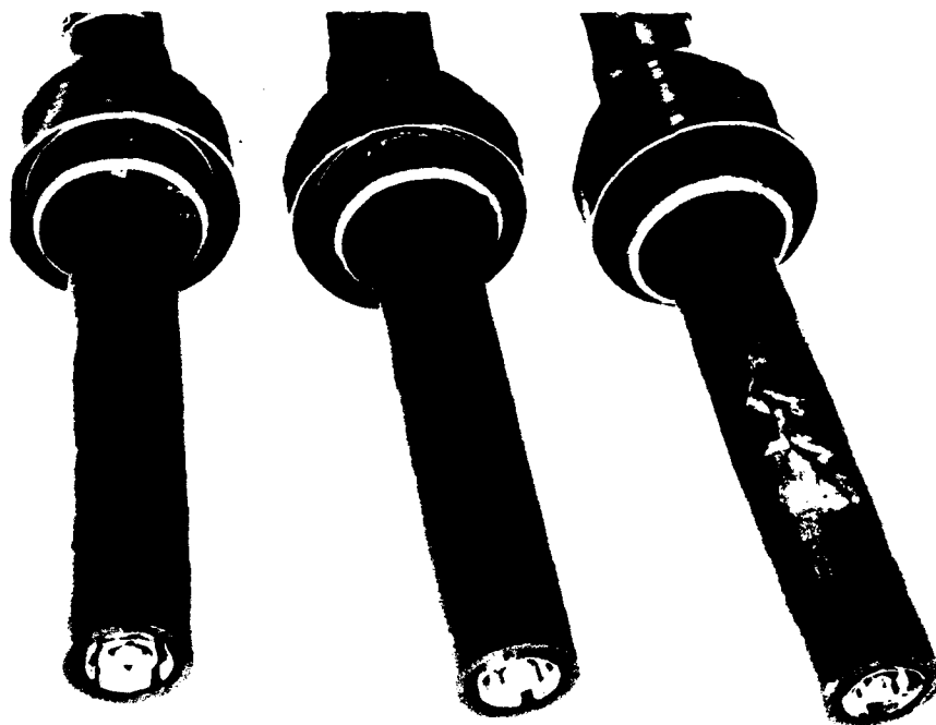
FIGURE 242.—Deterioration of cable housing with breakdown of insulation in the terminal.
