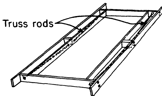
FIGURE 207.—Frame devised to fit X-ray field table unit with pressed wood cover removed.
