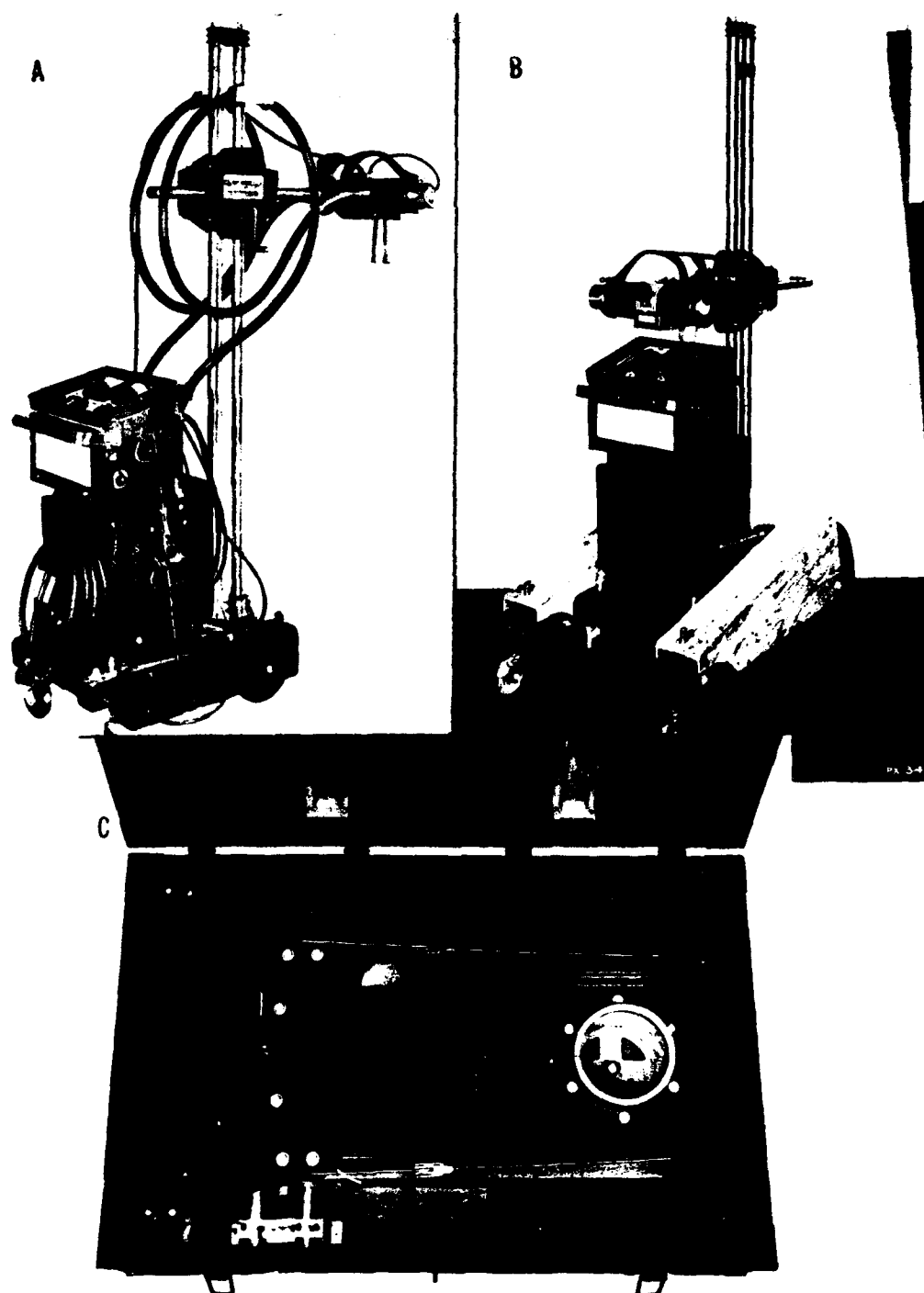
FIGURE 19.—Picker portable basic field X-ray unit. A. Early model, with small wheels. B. Later model, with larger wheels. C. Later model packed for transportation (see fig. 18).
