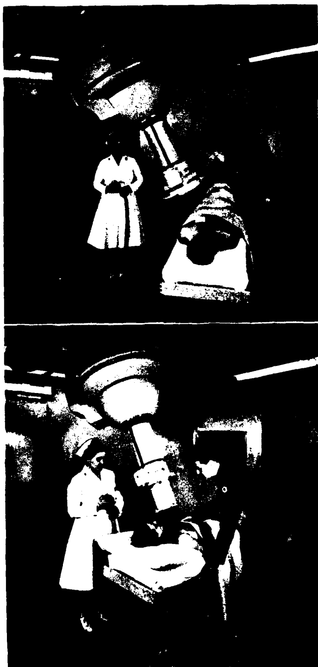
FIGURE 57. —One-million volt X-ray therapy machine, resonant transformer generator. A. Light-beam localizer focused on anterior left chest portal. Movement of machine in all directions is controlled by switch in nurse's hand. B. Double diaphragm system added to nozzle of machine for sharp collimation of X-ray beam.
