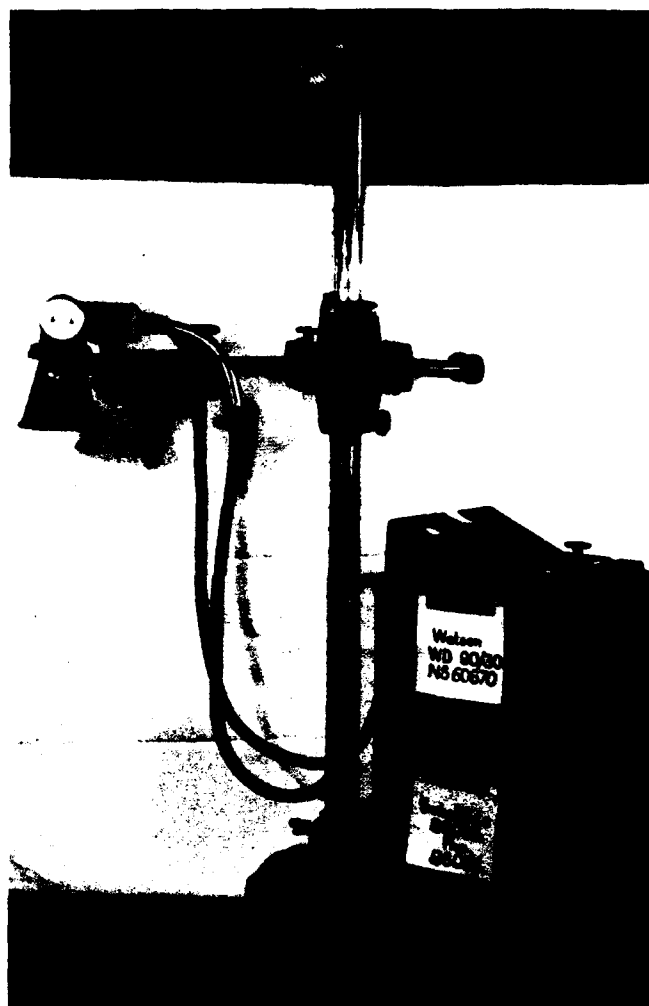
FIGURE 129.—British 90-kv., 30-ma., mobile (not portable) unit, of which 300 were purchased, was sturdy and dependable for work on a smooth, level floor.
