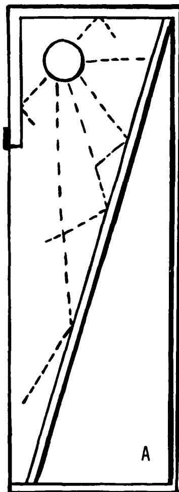
FIGURE 142.—Improvised plywood illuminator made without glass. Reflector surface of plywood is covered with white enamel (2). A. Details of construction. B. Illuminator in use.
