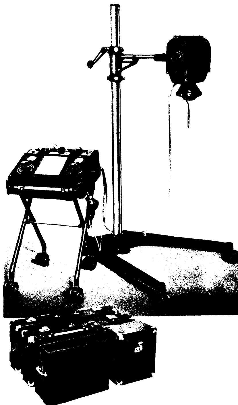
FIGURE 131.—Watson portable X-ray apparatus, type MX-2. Top, ready for use. Bottom, packed in carrying cases, which contain everything except folding stand for control unit.
