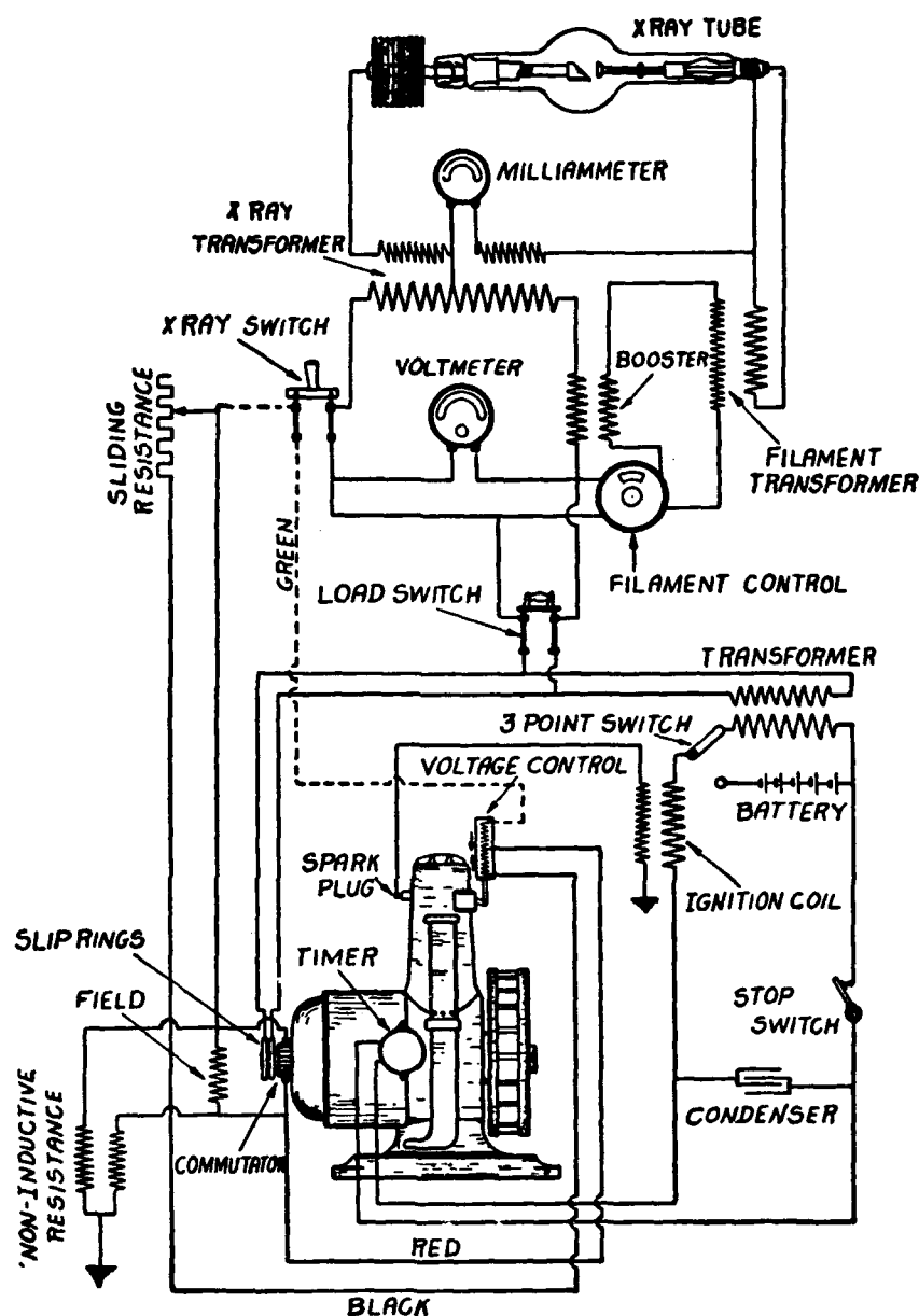
FIGURE 14.—Diagram of wiring for World War I portable X-ray unit. Dotted lines show connections for machines with special control (2).
