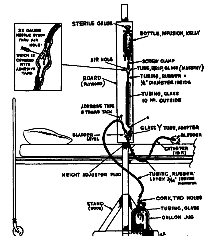
FIGURE 2.—Automatically controlled or tidal system.
