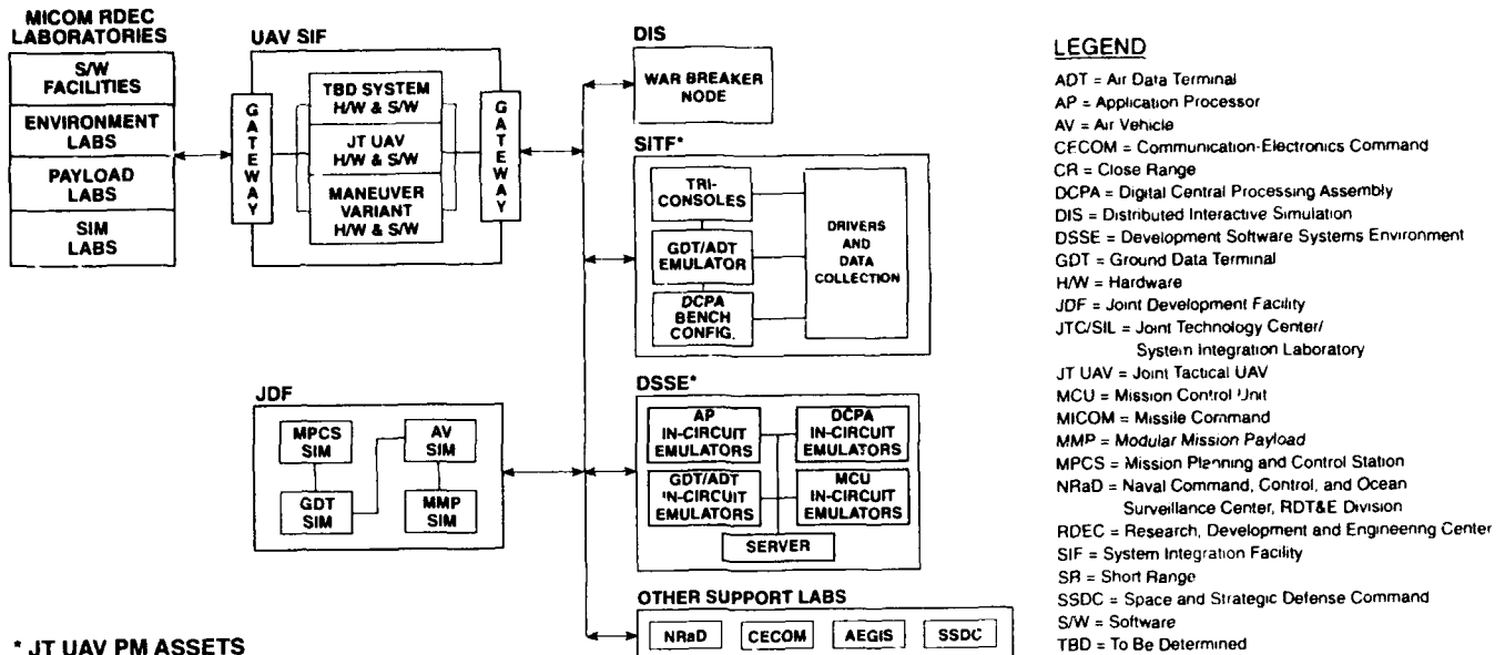
Figure 4-6 UAV JTC/SIL
