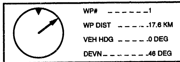
Driver's Steer-To-Display
