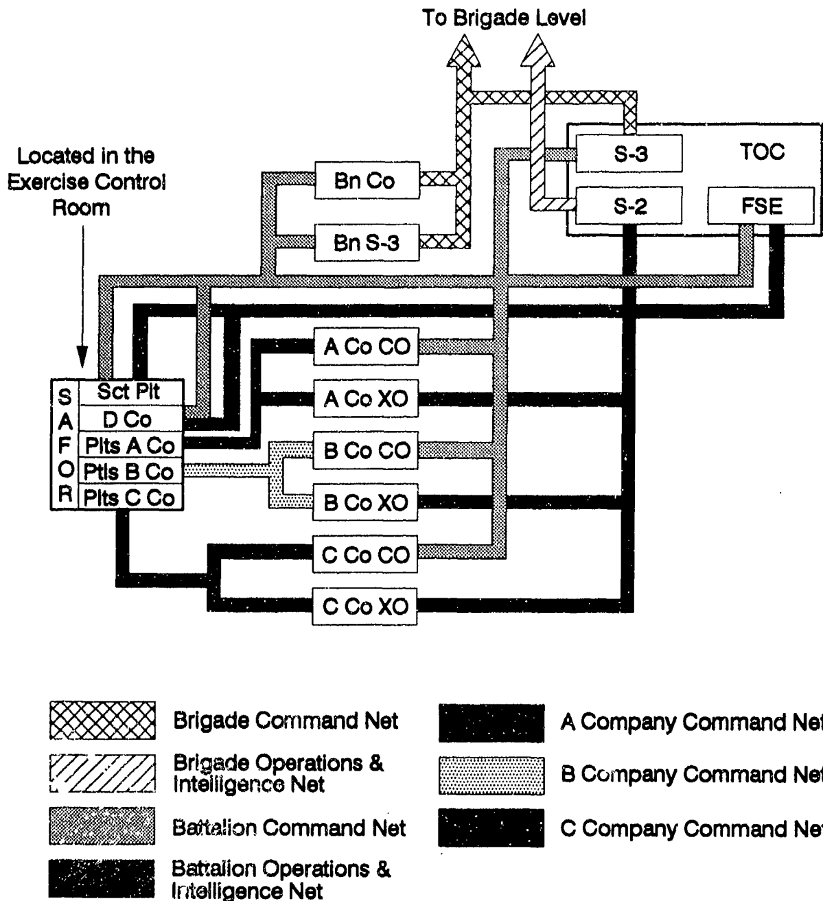
Figure 13. Diagram of the tactical voice radio networks used in the battalion-level evaluation.
