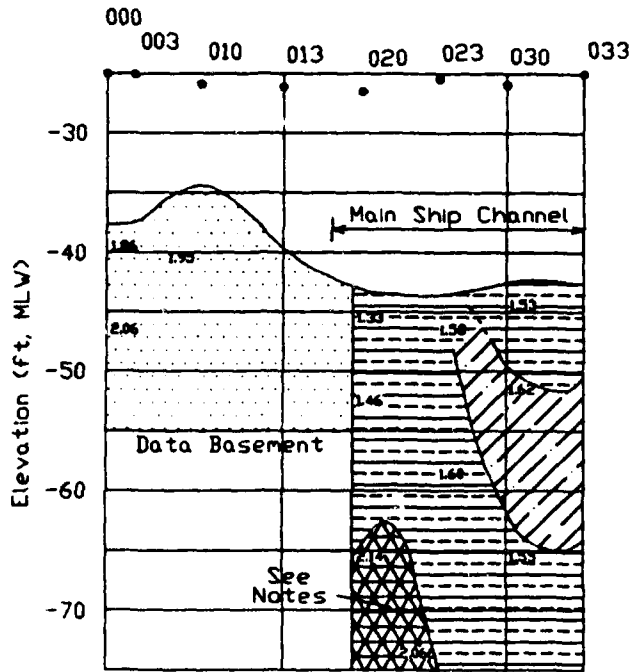
Inner Confluence Area WES Survey Line 5
