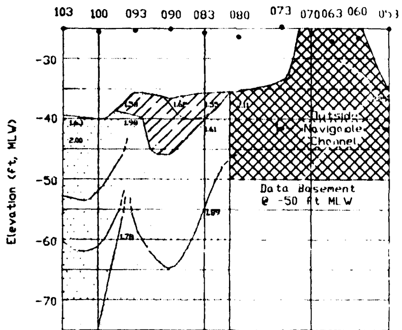
Chelsea River WES Survey Line 8
