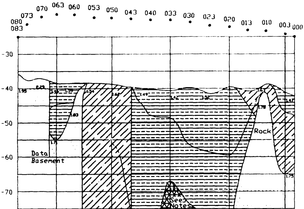
Reserved Channel WES Survey Line 5
