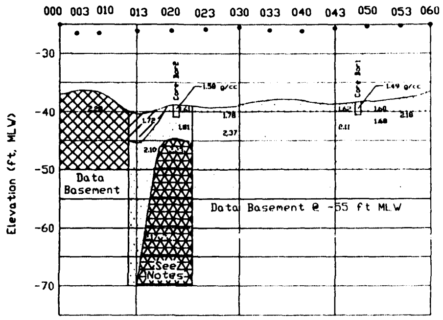
Chelsea River WES Survey Line 7
