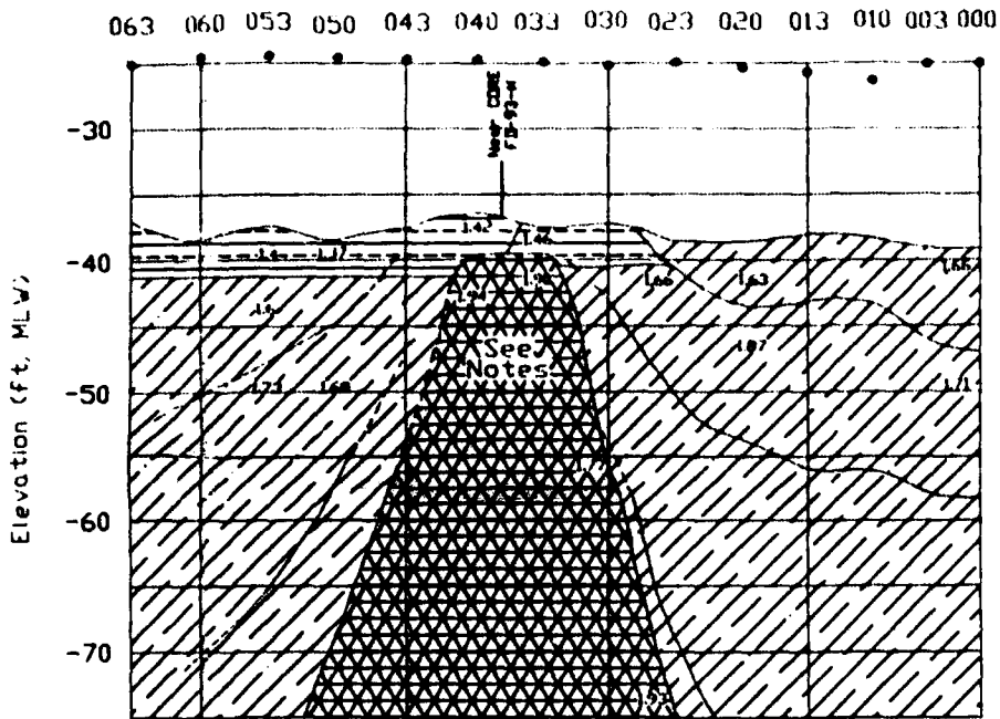
Mystic River WES Survey Line 6
