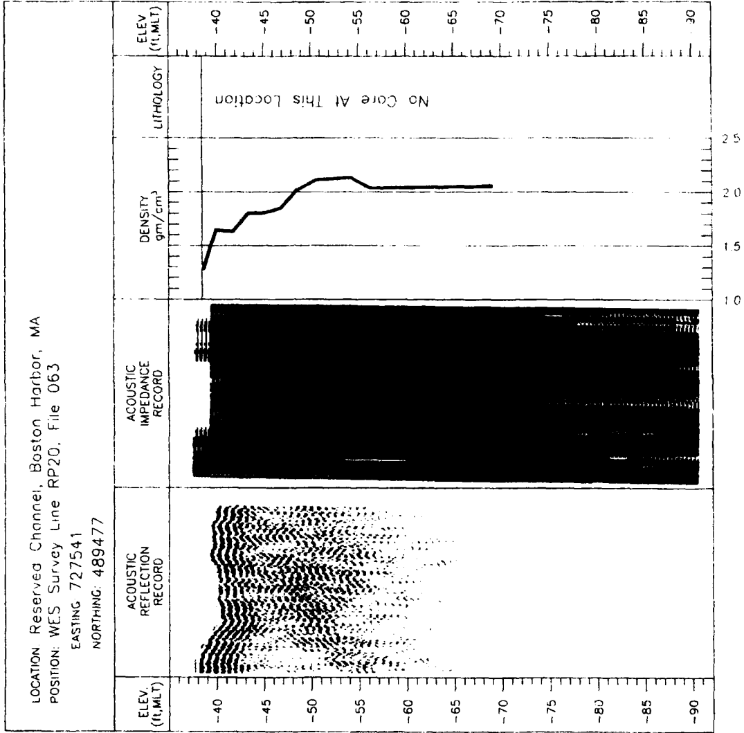
Figure 39. Check calibration, Reserved Channel
