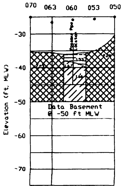
Inner Confluence Area WES Survey Line 16
