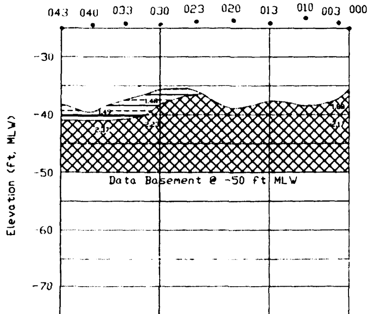
Chelsea River WES Survey Line 10
