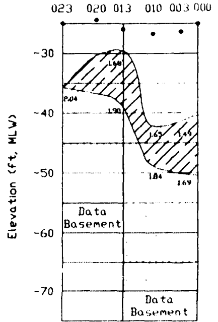
Chelsea River WES Survey Line 13
