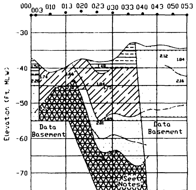
Inner Confluence Area WES Survey Line 8
