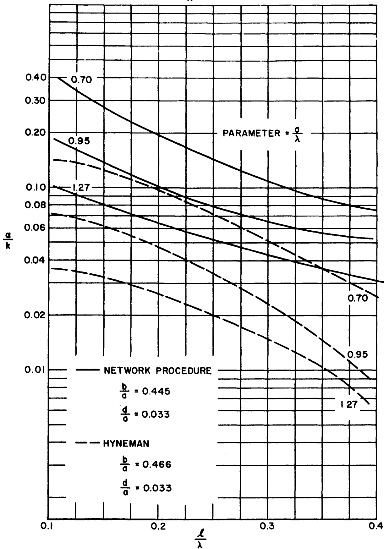
Fig.5. THEORETICAL ATTENUATION vs. SLOTT SPACING IN WAVELENGTHS
