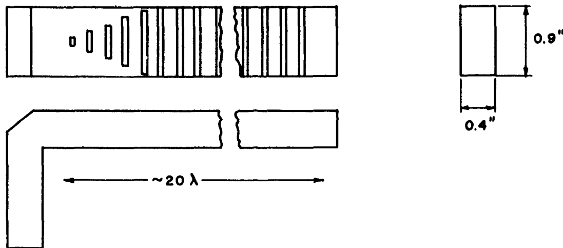
Fig. 8 Antenna constructed for the measurements.
