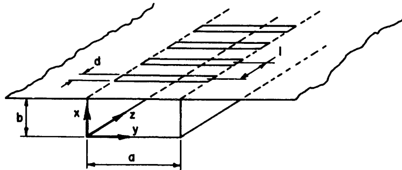
Figure 1. Transversely-slotted waveguide
