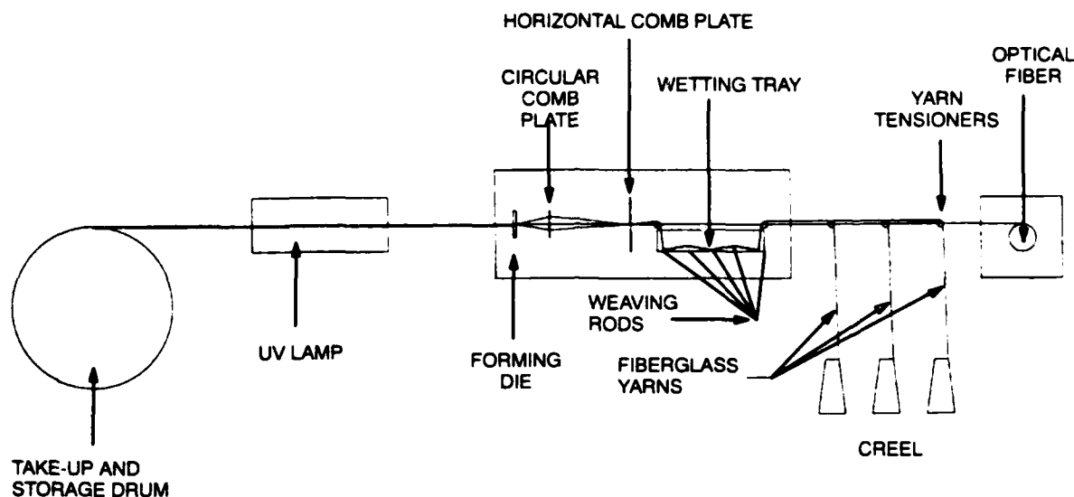
Figure 2. Research and test plant.
