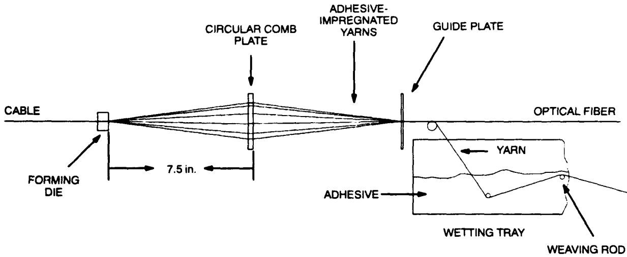
Figure 4. Comb plate and forming die positions.
