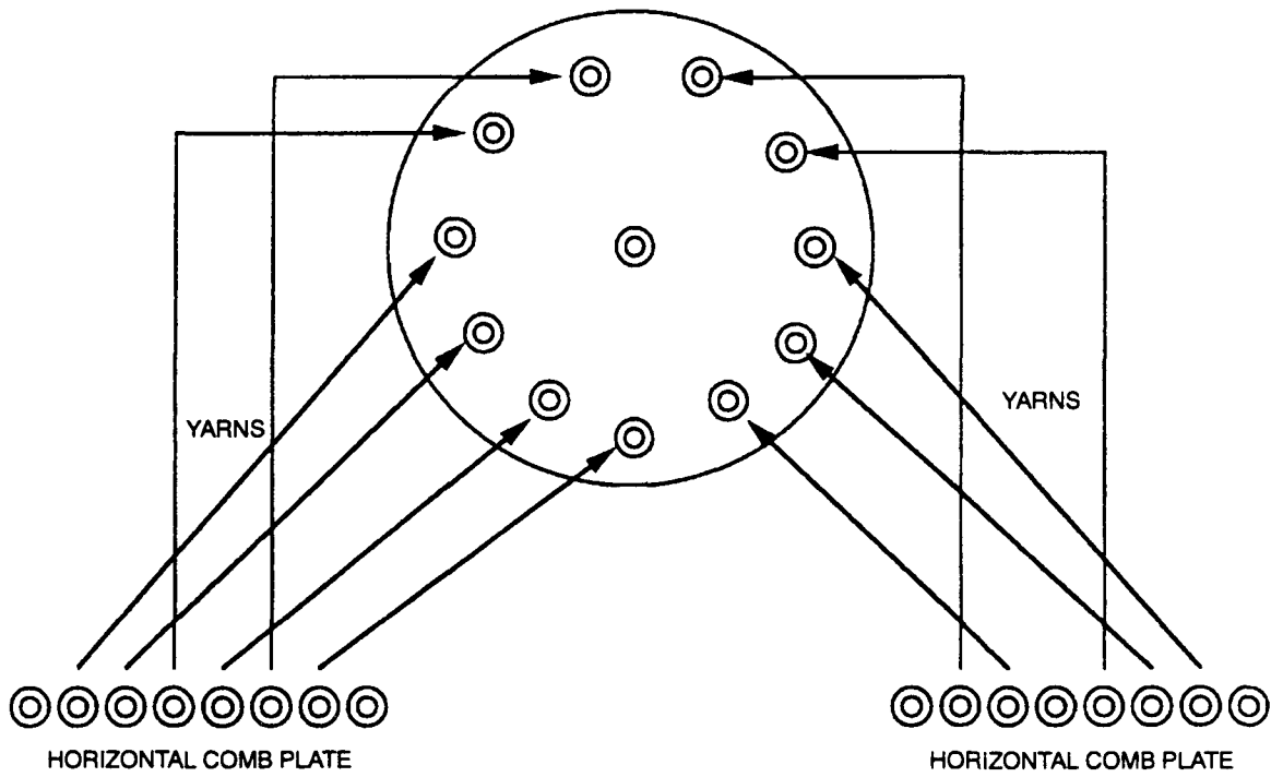
STRINGING PATHS FOR THE SECOND WETTING BOX
