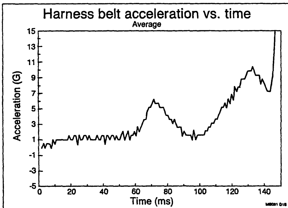
Figure 12b. Harness belt acceleration obtained by double differentiation of output of simulation 1.
