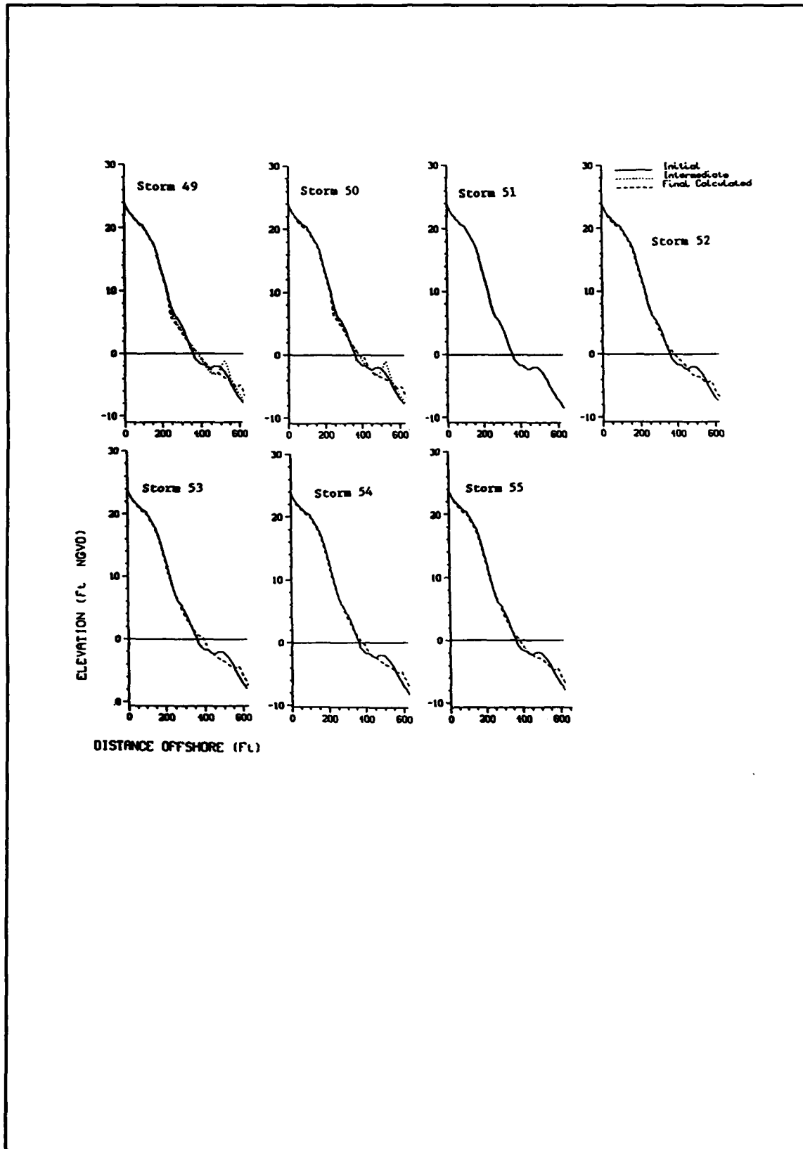
Figure D5. Response of R-21, existing conditions, training storms 49-55
