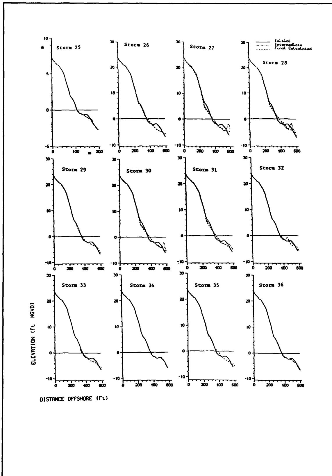
Figure D3. Response of R-21, existing conditions, training storms 25-36
