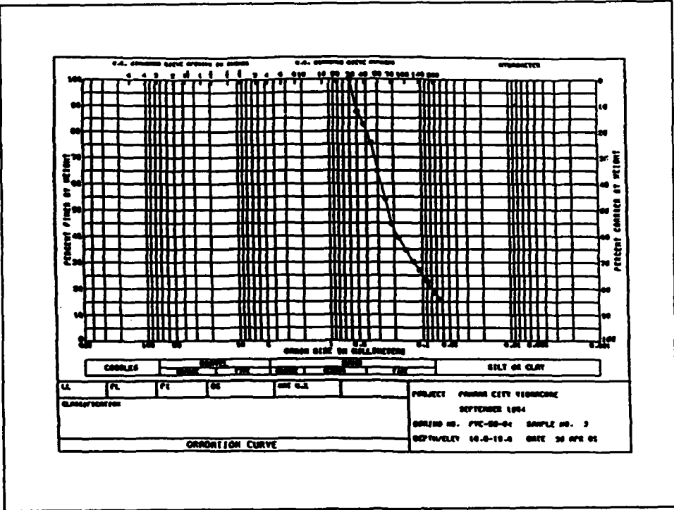
Figure A4. Sand gradation curve of an offshore sample
