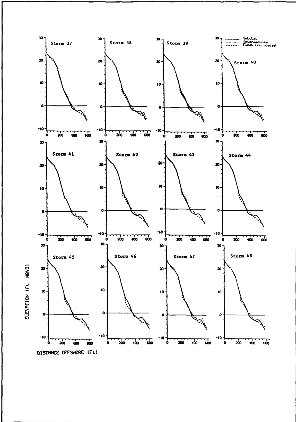
Figure D4. Response of R-21, existing conditions, training storms 37-48
