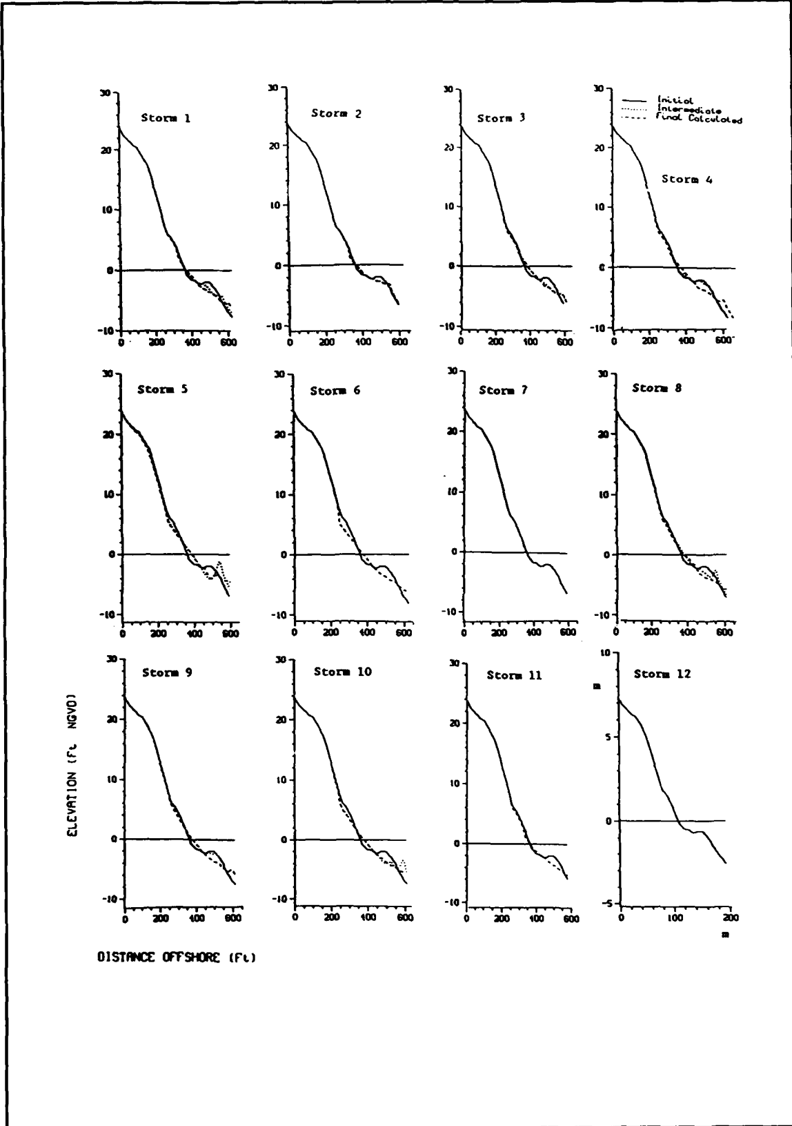
Figure D1. Response of R-21, existing conditions, training storms 1-12
