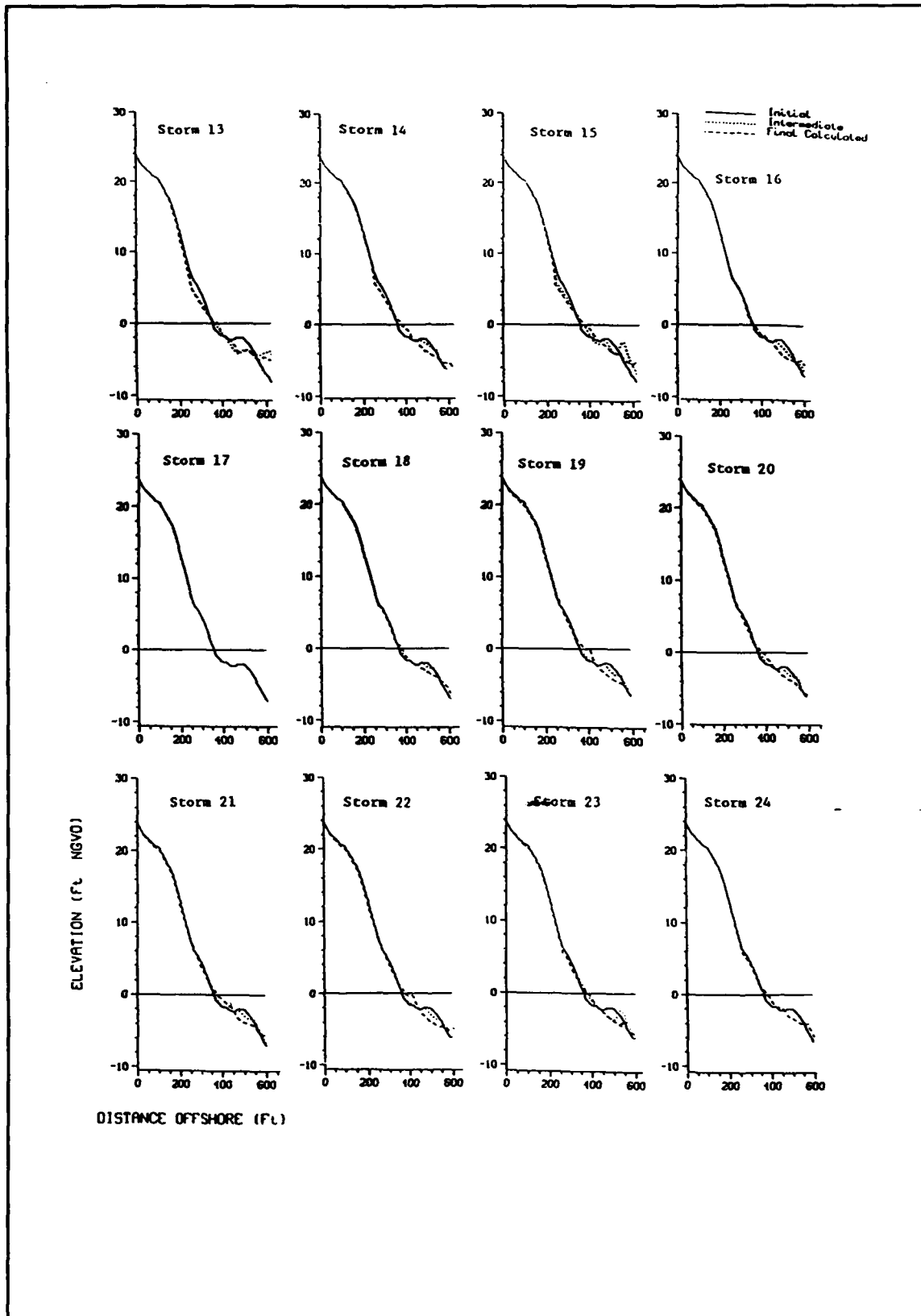
Figure D2. Response of R-21, existing conditions, training storms 13-24
