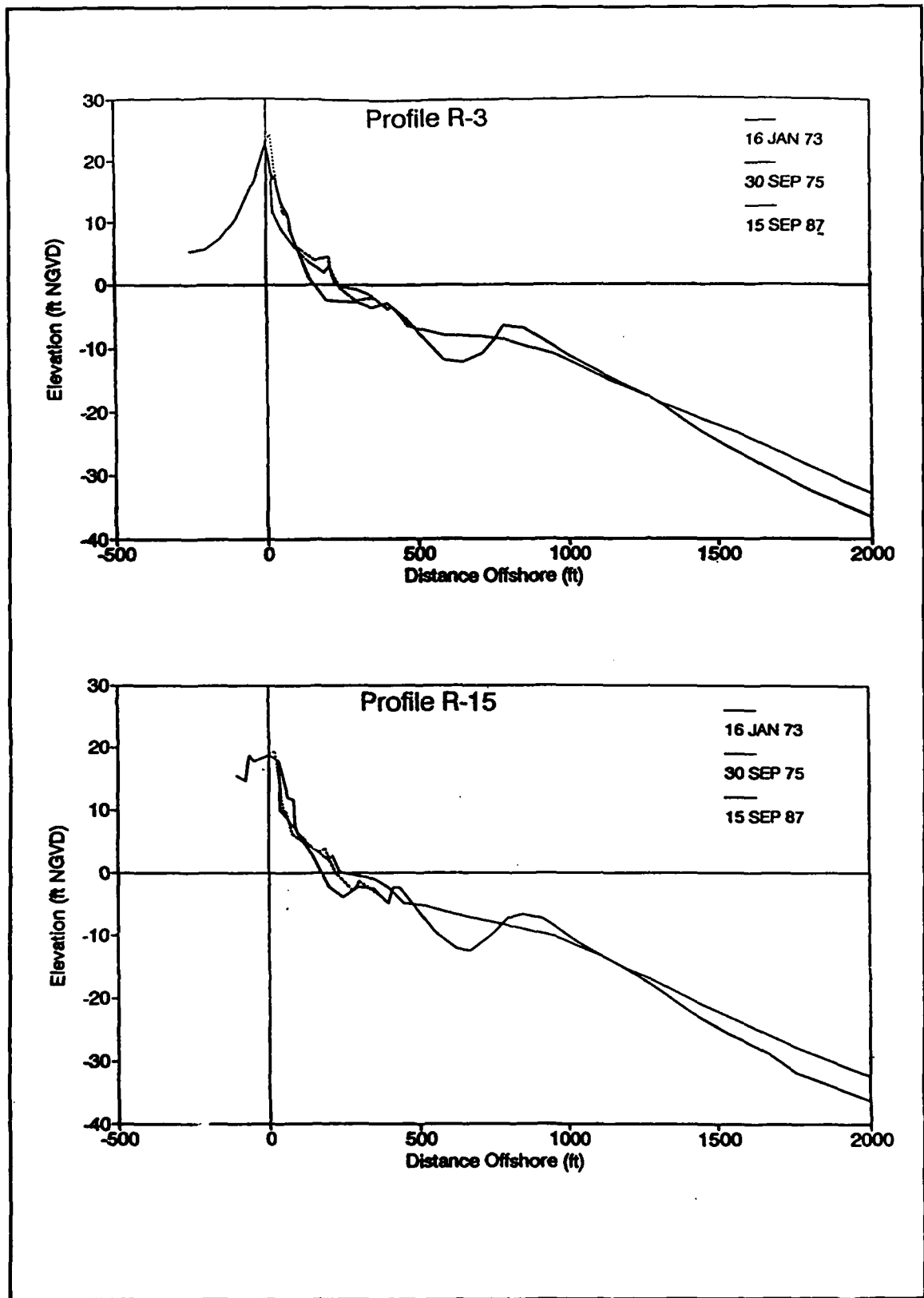
Figure B1. R-3 and R-15 profile surveys
