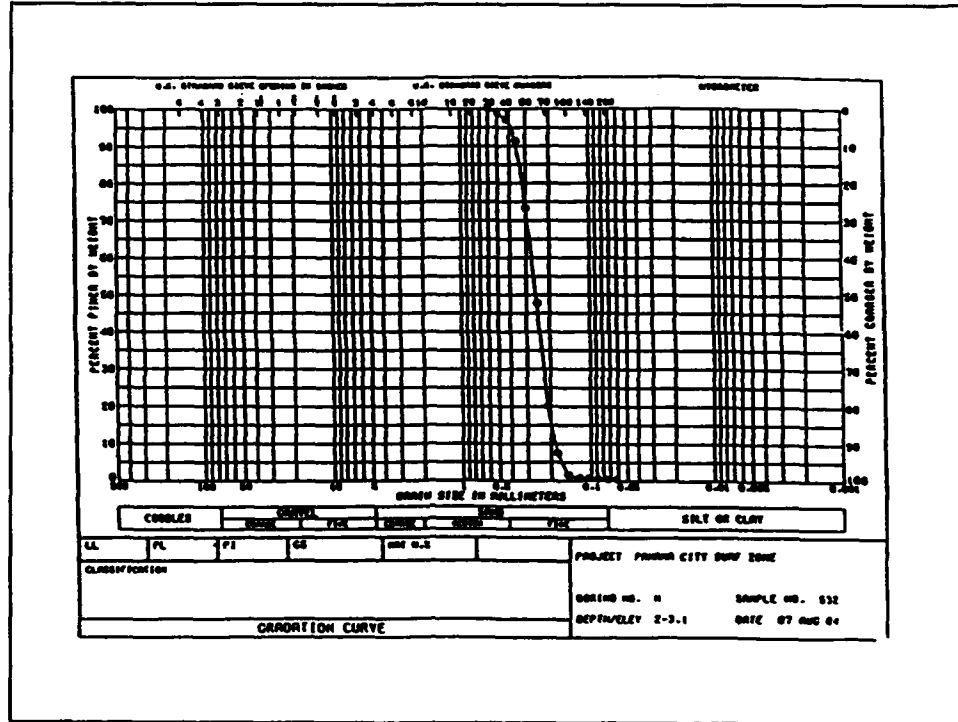
Figure A2. Sand gradation curve of a surf zone sample
