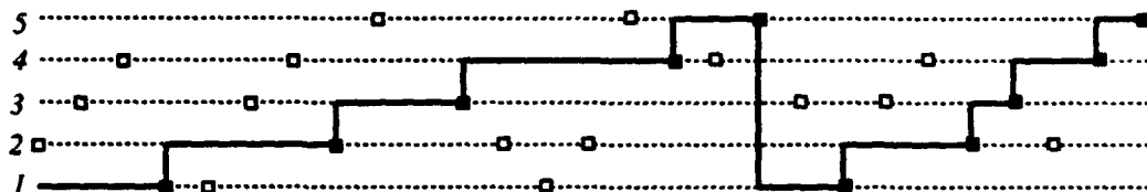
Figure 4.1: A sleepy pager that moves the hole in the cyclical order \langle 1, 2, 3, 4, 5 \rangle . Each dotted horizontal line represents a page. The dark solid line represents the path of the hole (missing page). Each square is a page request; the darkened squares are requests that hit the hole (page faults), and are therefore the only ones the pager is aware of.
