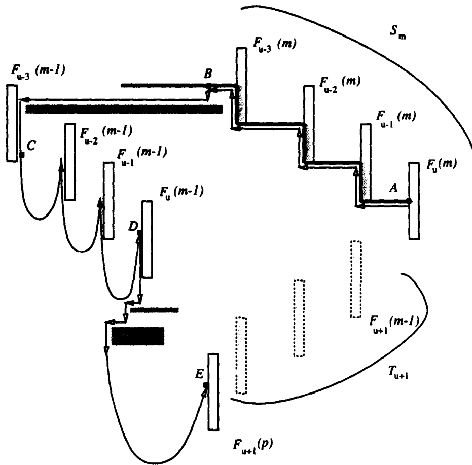
Figure 3.19: A use of procedure \text{JumpDownLeft} to jump from F_u(m) to F_{u+1}(p) , for clarity shown in a scene where the fence posts correspond exactly to obstacles of height 2\tau . Shaded rectangles with no boundaries are obstacles that are not part of any fence. Solid-boundary rectangles are nodes found so far in the tree. Dotted-boundary rectangles are nodes that will be eventually found in the tree. Thick solid lines are tree edges. The thin arrow line is the path followed when executing the procedure. Each curved arrow line shows an execution of procedure \text{JumpDownRight} .
