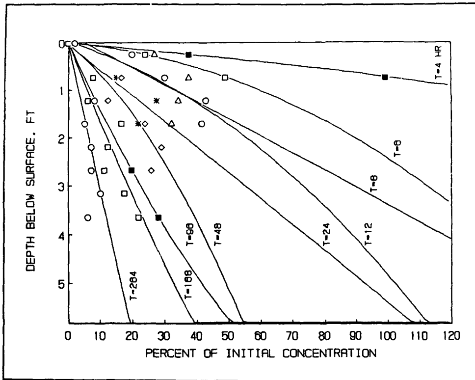
Figure 7. Solids concentration profile curve for Reach 1
