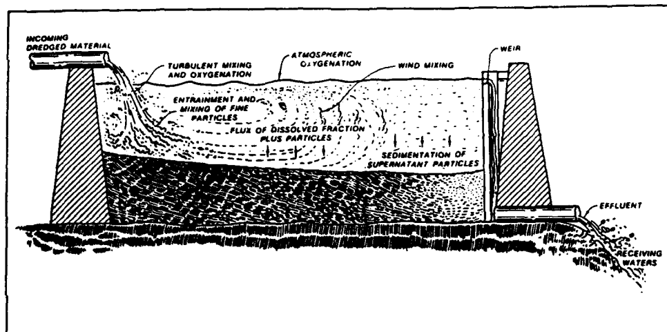
Figure 1. Schematic of an active CDF
