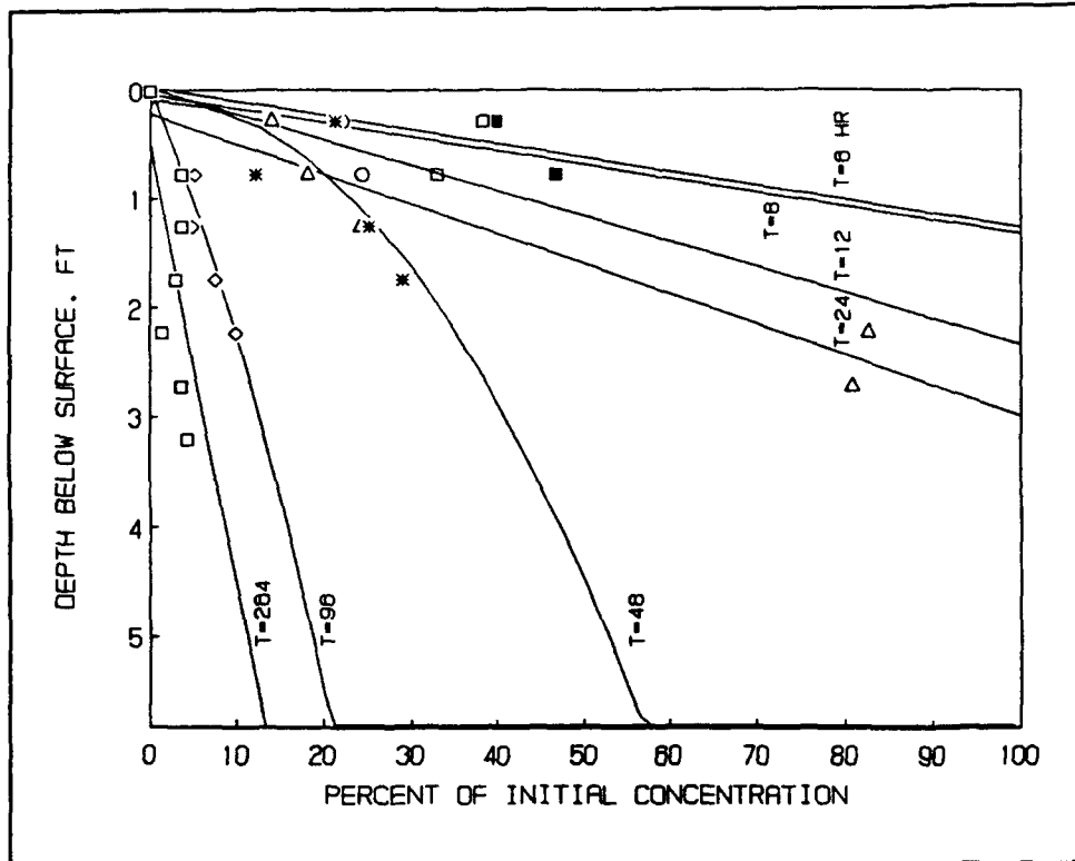
Figure 11. Solids concentration profile curve for Reach 3
