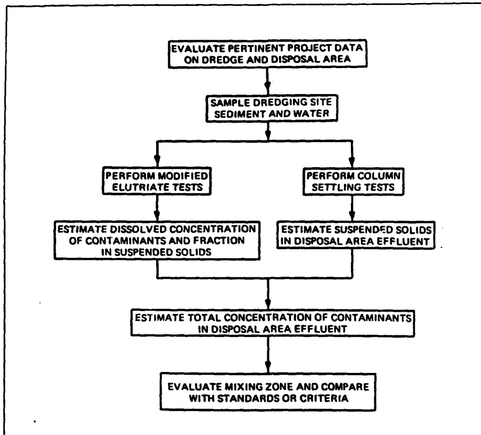
Figure 2. Steps for predicting effluent water quality (Palermo 1984)
