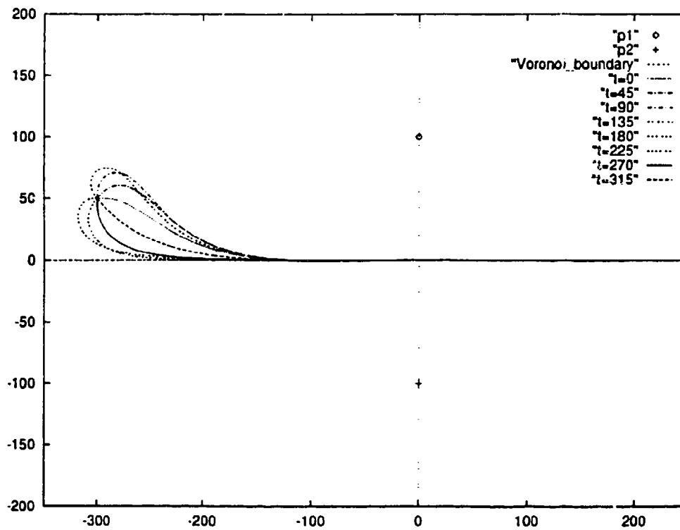
Figure 5.7 : Simulation Result of Two Points, q = ((-300, 50), \theta, 0)
