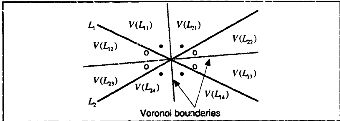
Figure 3.2 : Voronoi Diagram of Two Lines (Not Parallel)
