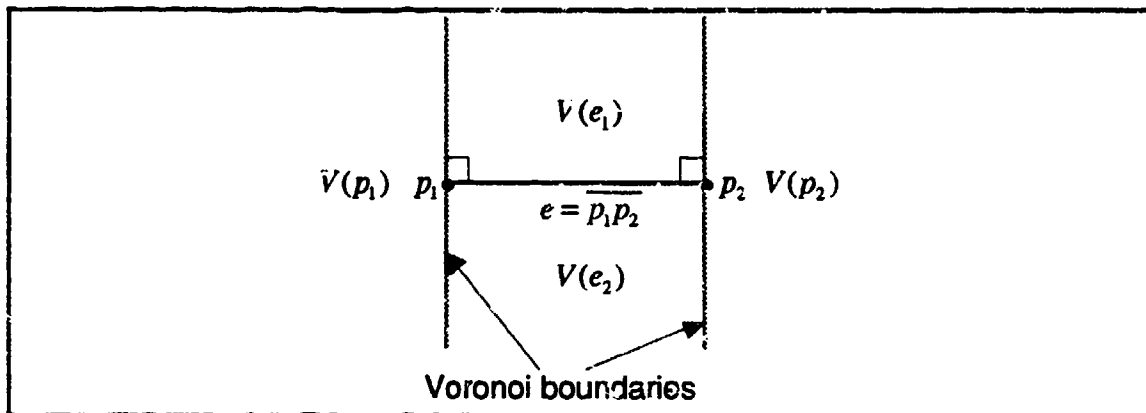
Figure 3.4 Voronoi Diagram of A Line Segment
