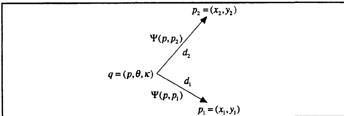
Figure 5.6 : Case \Psi(p, p_1) - \Psi(p, p_2) < 0
