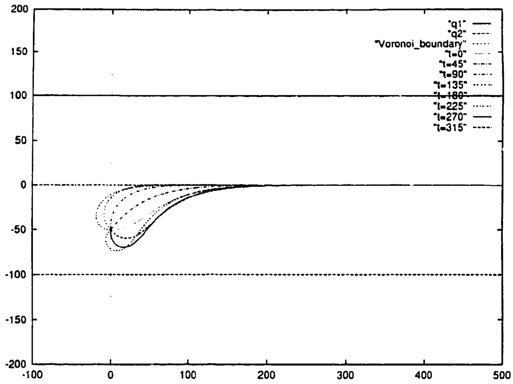
Figure 5.13 : Simulation Result of Parallel Lines, q = ((0, -50), \theta, 0)
