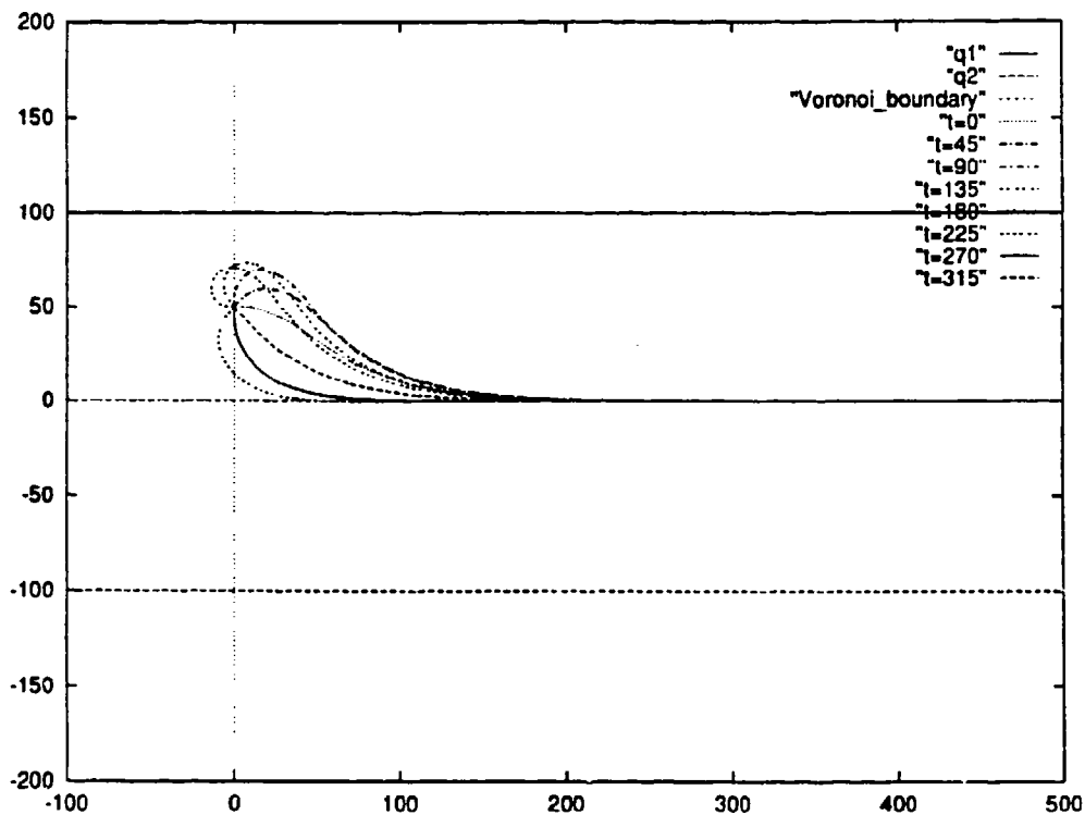
Figure 5.12 : Simulation Result of Parallel lines, q = ((0,50),\theta,0)
