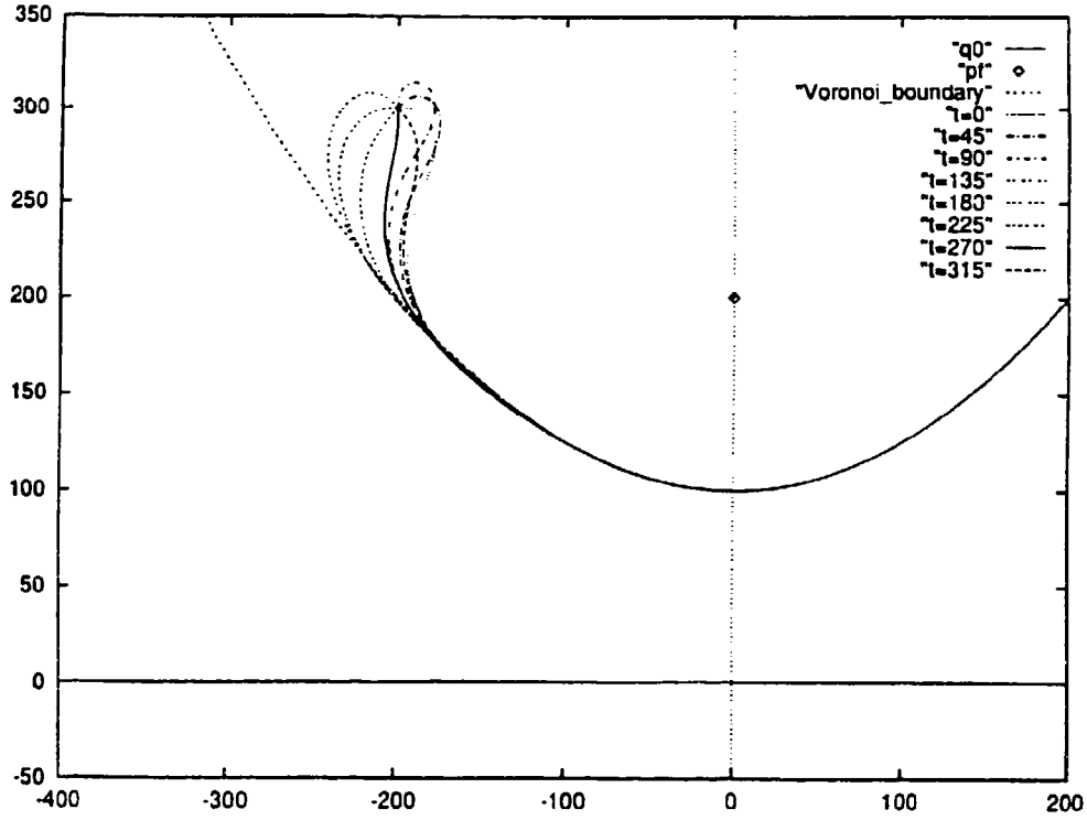
Figure 5.23 : Simulation Result of l > 0 , q = ((-200, 300), \theta, 0)
