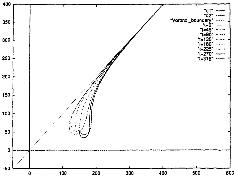
Figure 5.15 : Simulation Result of Not Parallel Lines, q = ((150,50),\theta,0)
