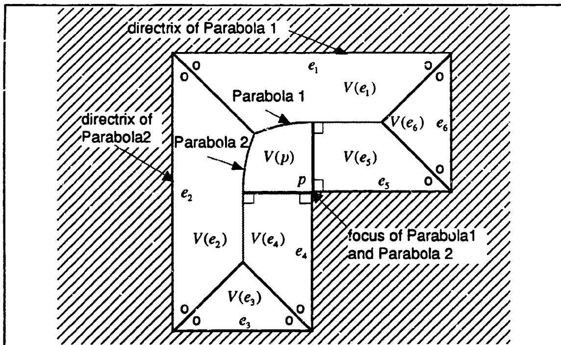
Figure 3.12 : Voronoi Diagram of An Inverted Polygon
