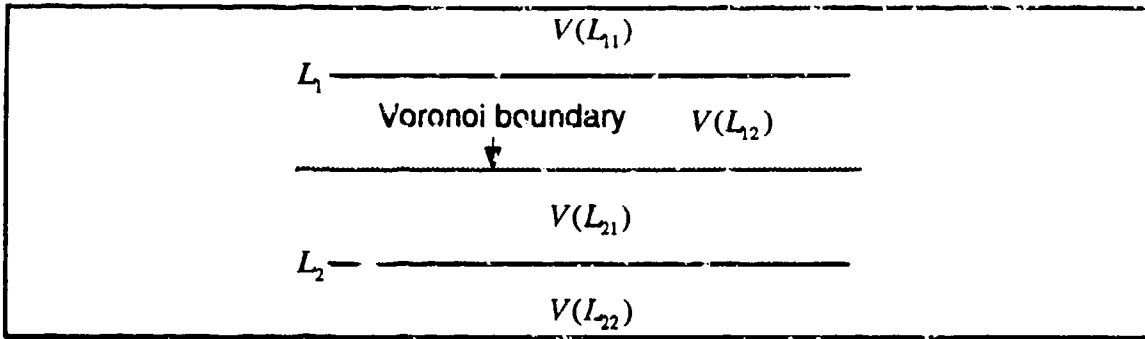
Figure 3.3 : Voronoi Diagram of Two Parallel Lines
