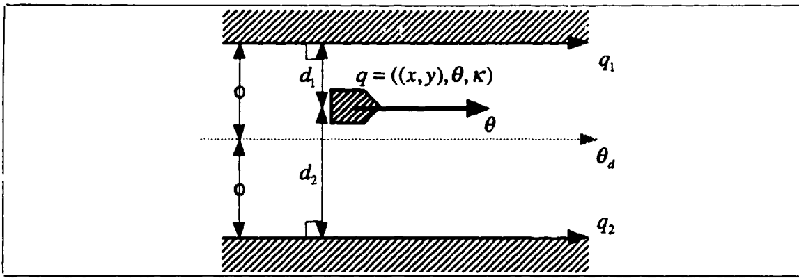
Figure 5.9 : Parallel Directed Lines
