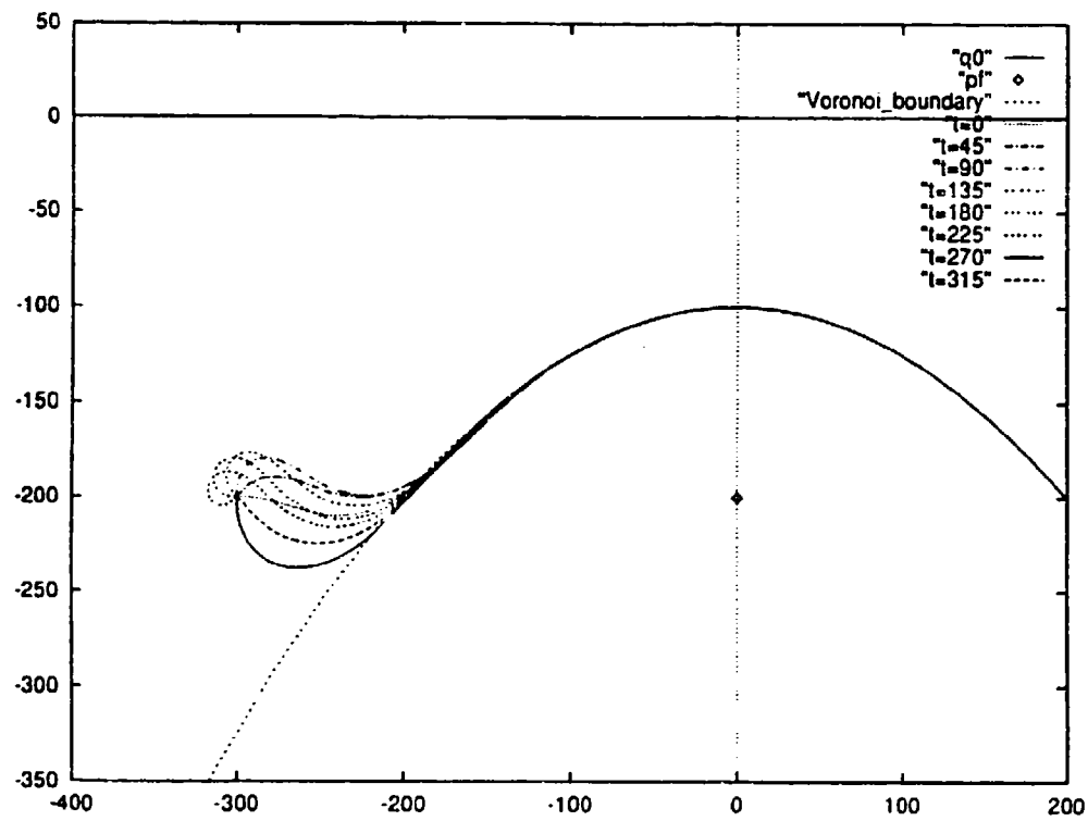
Figure 5.24 : Simulation Result of l < 0 , q = ((-300, -200), \theta, 0)
