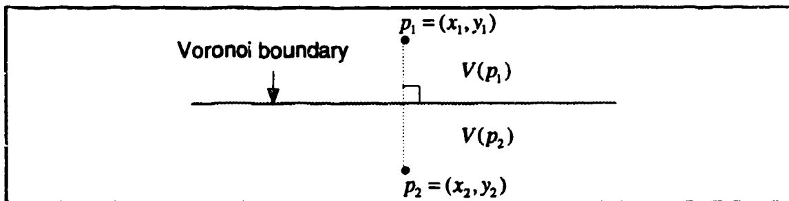
Figure 3.1 : Voronoi Diagram of Two Points
