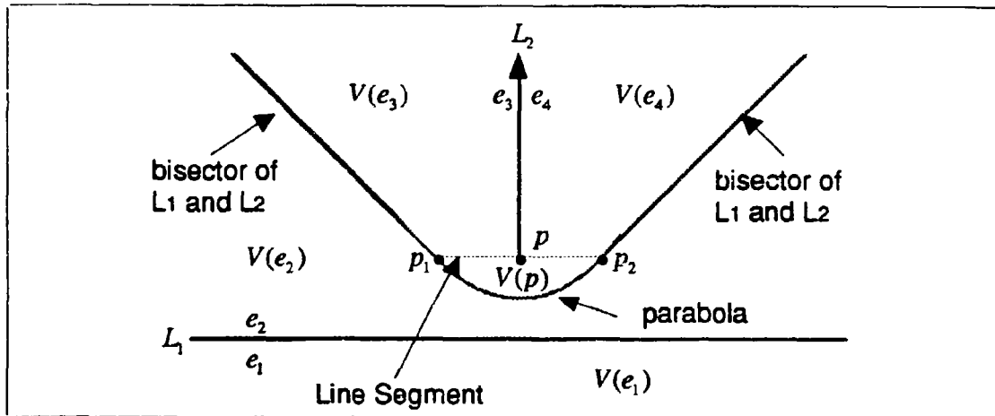
Figure 3.8 : Voronoi Diagram of Line and Ray
