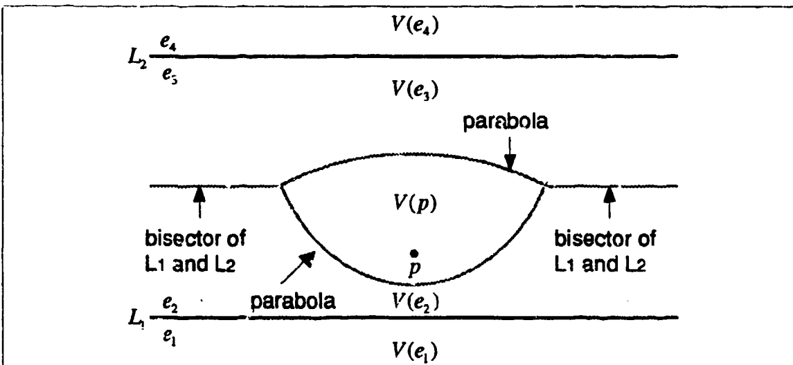
Figure 3.7 : Voronoi Diagram of A Point and Two Lines
