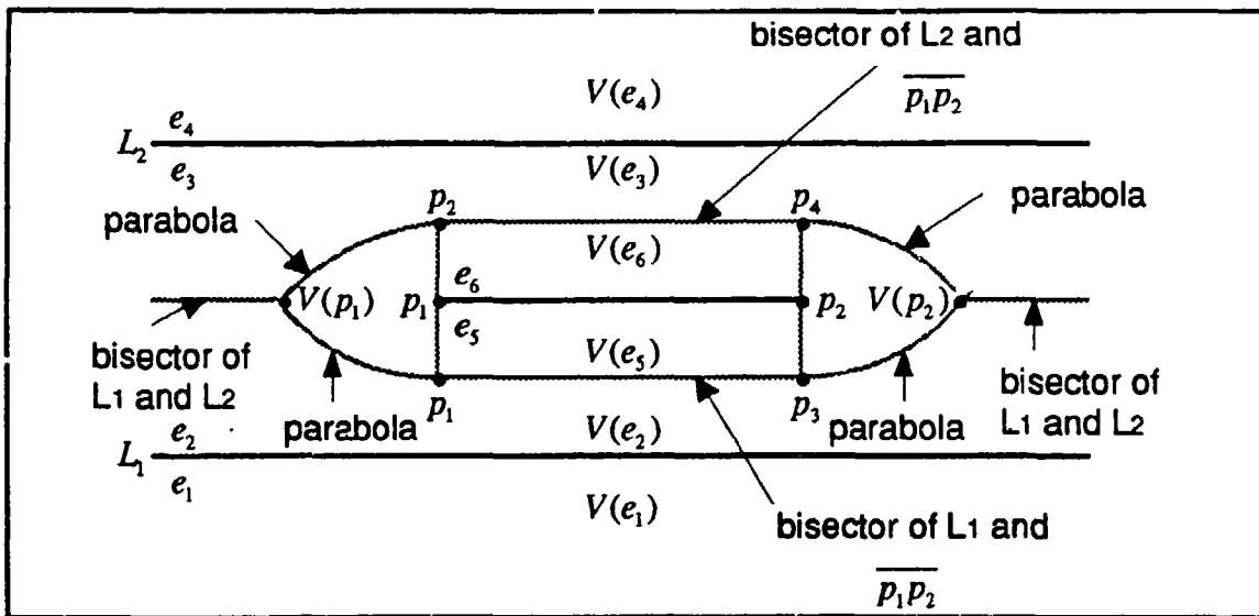
Figure 3.9 : Voronoi Diagram of Two Lines and A Center Line Segment
