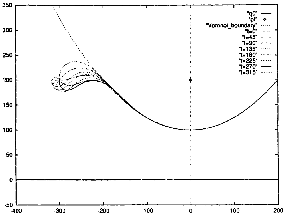
Figure 5.22 : Simulation Result of l > 0 , q = ((-300, 200), \theta, 0)
