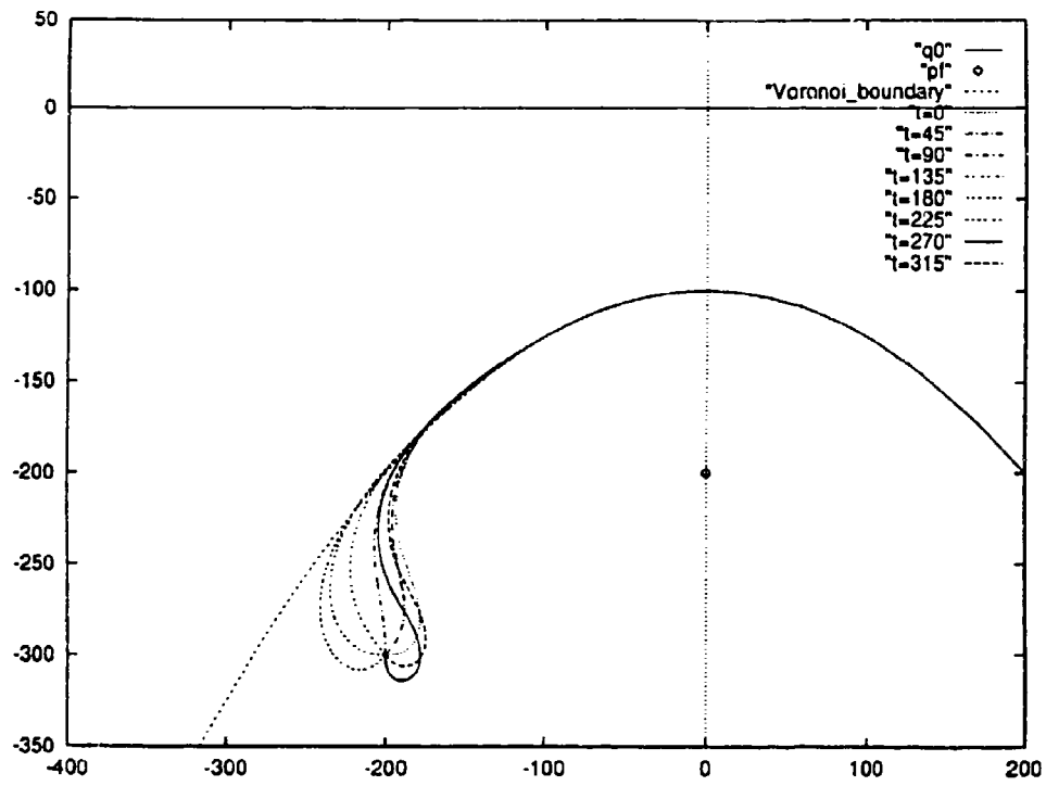
Figure 5.25 : Simulation Result of l < 0 , q = ((-200, -300), \theta, 0)
