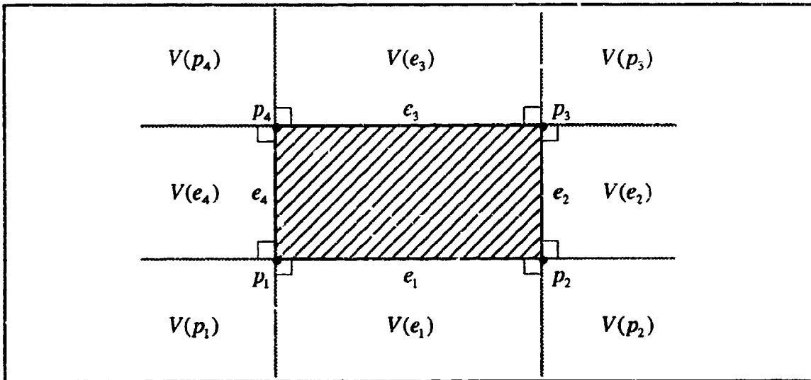
Figure 3.11 : Voronoi Diagram of A Normal Polygon
