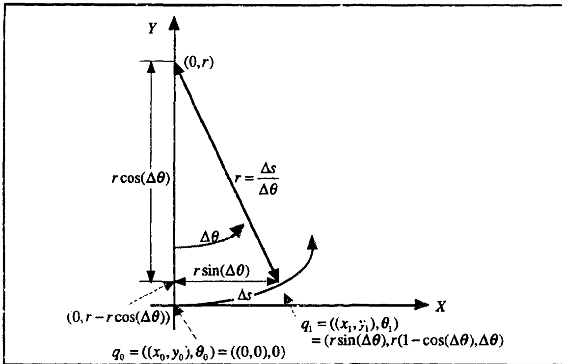
Figure 4.1 : Short Circular Segment
