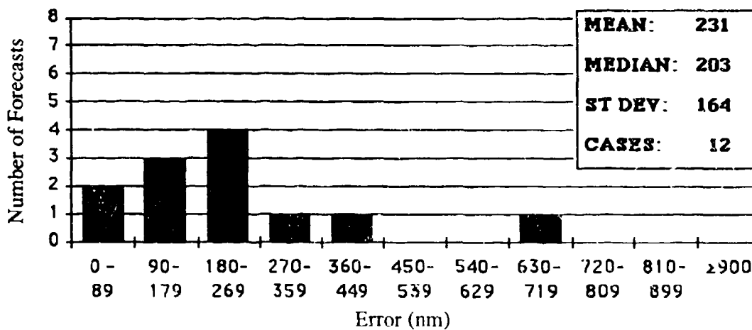
Figure 5-5f Frequency distribution of 72-hour forecast errors (90-nm increments) for the North Indian Ocean in 1993. The largest error, 651 nm, was on TC01A.
