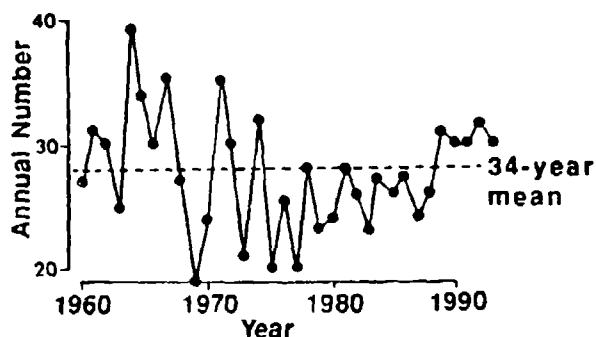
Figure 3-2 Tropical cyclones of tropical storm or greater intensity in the western North Pacific (1960-1993)
