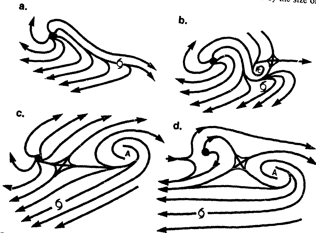
Figure 3-14-2 A model of upper-level streamlines based on composited 200-mb winds and cirrus plume orientations taken from satellite imagery associated with Robyn (13W) and Steve: (a) Composite for 5 through 7 August, (b) Composite for 8 through 10 August, (c) Composite for 10 and 11 August, and (d) Composite for 12 and 13 August. Solid black dot = the location of Robyn and tropical cyclone symbol = Steve.
