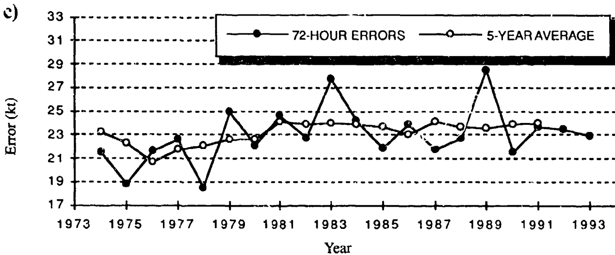
Figure 5-4 Mean intensity forecast errors (kt) and 5-year running mean for a) 24 hours, b) 48 hours and c) 72 hours for the western North Pacific Ocean for the period 1974 to 1993.
