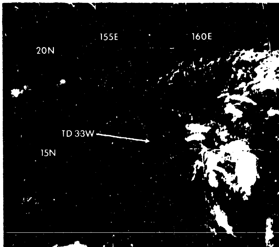
Figure 3-33-1 The only deep convection associated with TD 33W remains to the east of the exposed low-level circulation (182230Z November visual GMS imagery).
