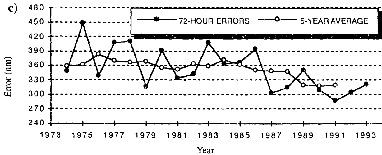
Figure 5-3 Mean track forecast error (nm) and 5-year running mean for a) 24 hours, b) 48 hours and c) 72 hours for the western North Pacific Ocean for the period 1974 to 1993.
