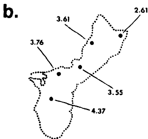
Figure 3-25-3 Total precipitation for Ed's passage over Guam: a) Storm total precipitation estimates from the NEXRAD for the period 282054Z September to 011504Z October. Shaded region = \geq 2 inches (50 mm), black areas \geq 3 inches (75 mm). Star locates the NEXRAD. (b) Storm total precipitation measurements from rain gauges for the same period.
