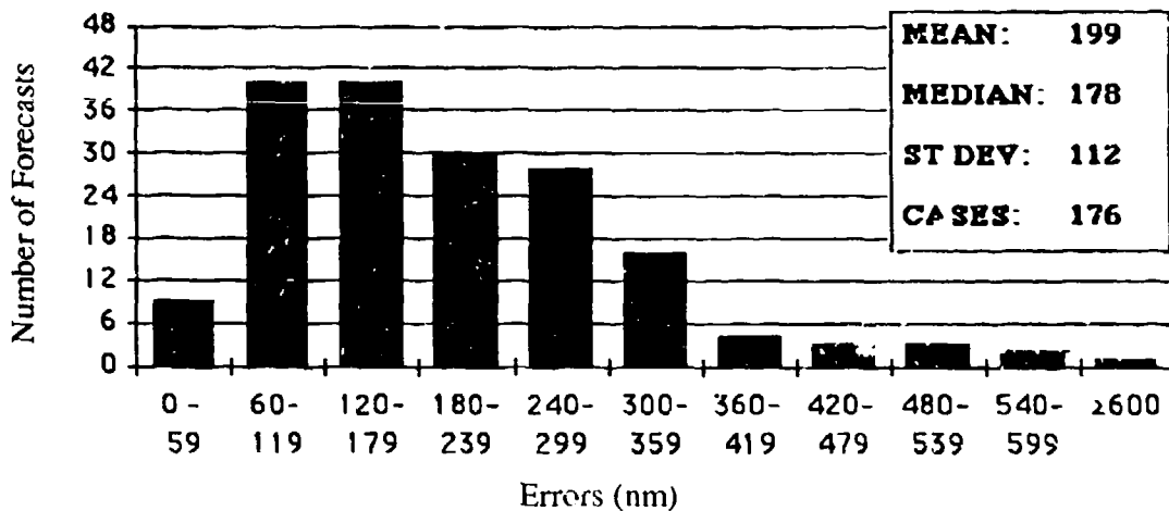
Figure 5-7e Frequency distribution of 48-hour forecast errors (60-nm increments) for the South Pacific and South Indian Oceans in 1993. The largest error, 618 nm, occurred on Tropical Cyclone 23P (Piema).
