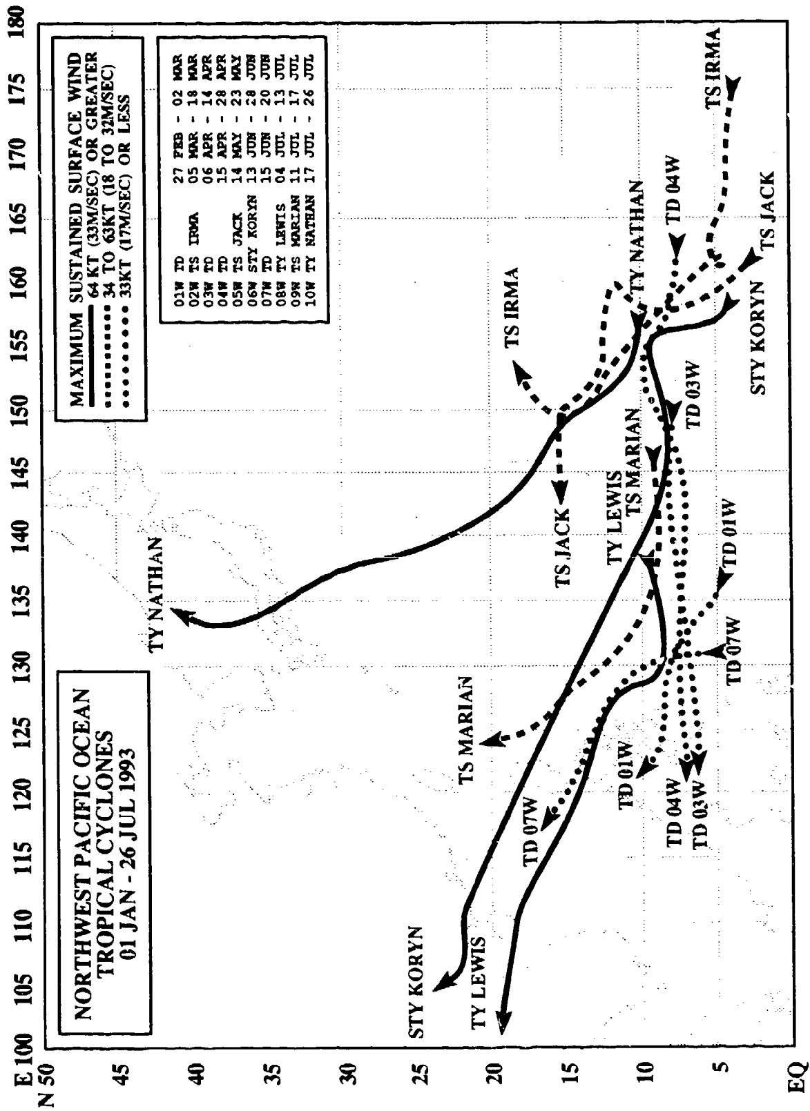
Figure 3-10 Composite best tracks for the North West Pacific Ocean: tropical cyclones for the period 1 January to 26 July 1993.
