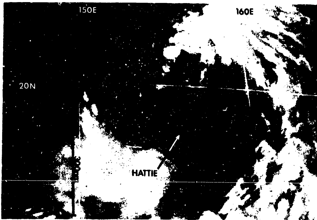
Figure 3-29-3 Hattie's exposed low-level circulation center (LLCC) appears between two areas of extensive convective cloudiness (220031Z October multispectral visual/infrared GMS imagery).
