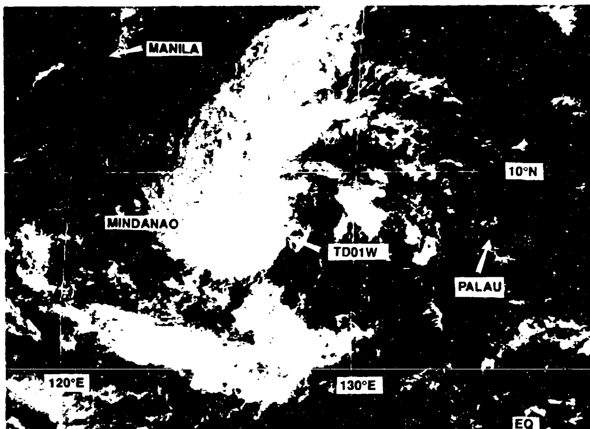
Figure 3-01-1 TD 01W approaches the island of Mindanao (010030Z March visual GMS imagery).
