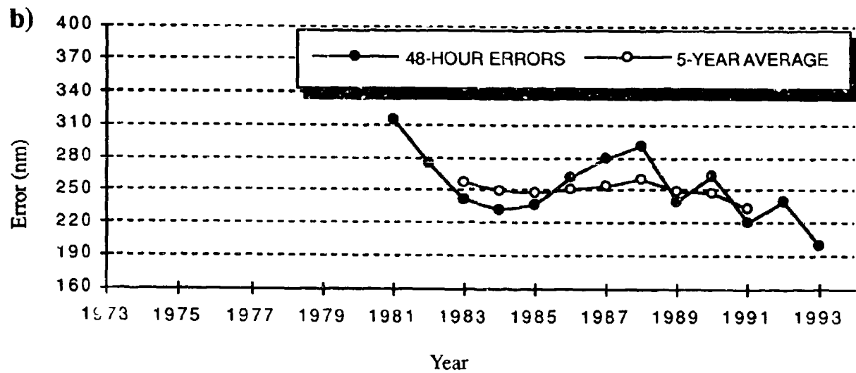
Figure 5-8 Mean track forecast errors (nm) and 5-year running mean for a) 24 hours and b) 48 hours for the South Pacific and South Indian Oceans for the period 1981 to 1993.
