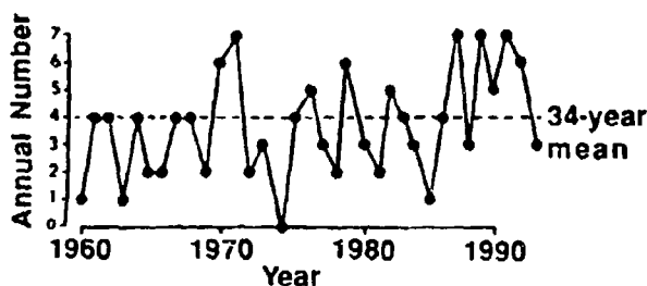
Figure 3-1 Number of western North Pacific super typhoons (1960-1993)
