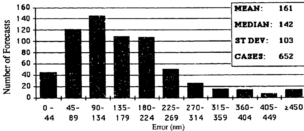
Figure 5-2d Frequency distribution of 36-hour forecast errors (45-nm increments) for the western North Pacific Ocean in 1993. The largest error, 574 nm, occurred on Typhoon Flo (26W).
