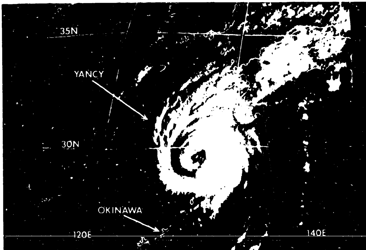
Figure 3-19-1 Visual image of Super Typhoon Yancy with a large, elongated eye, approximately seven hours prior to landfall in southern Kyushu. At this time, Yancy's maximum sustained winds were estimated to be 120 kt (62 m/sec) (022330Z, September visual GMS imagery.)
