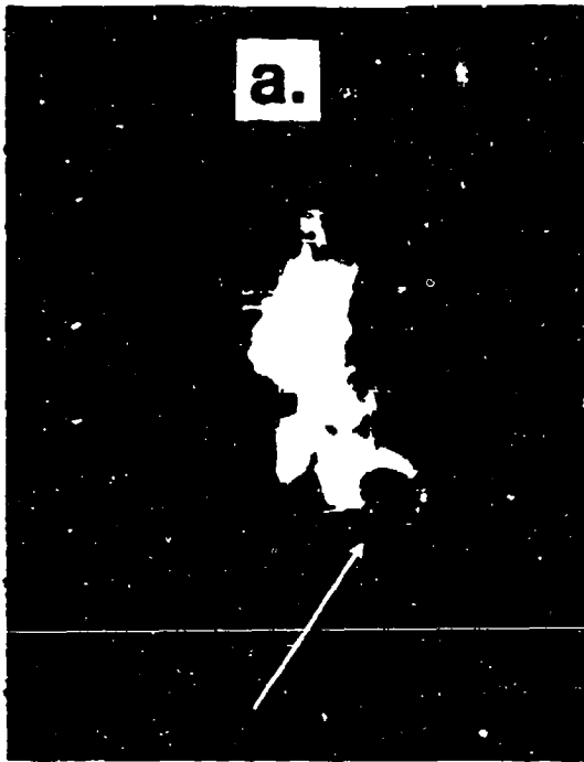
Figure 3-21-1 Radar images from Kaohsiung (WMO 46744): a) at 112200Z, and b) 121800Z September show the dramatic decrease in Abe's eye diameter from 25 to 8 nm (45 to 15 km) as intensification takes place (Radar photos courtesy of the Central Weather Bureau, Taipei, Taiwan).
