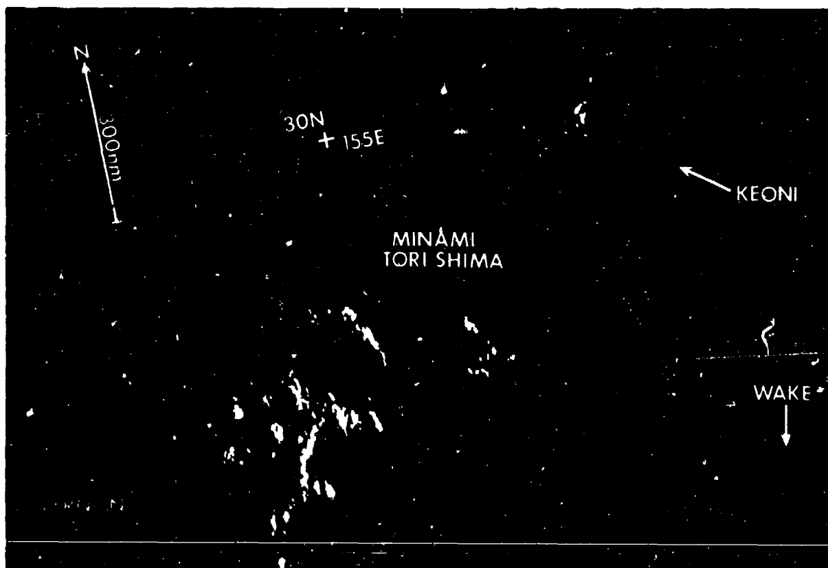
Figure 3-01C-1 Keoni tracks in tandem with Vernon (17W) (242313Z August visual NOAA imagery.)
