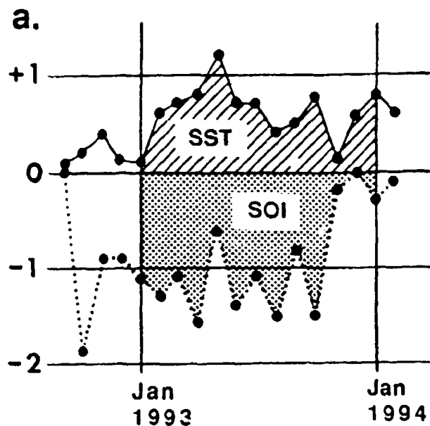
Figure 3-3a Anomalies from the monthly mean for eastern equatorial Pacific Ocean sea surface temperature (SST) (hatched) in degrees Celsius and the Southern Oscillation Index (SOI) (shaded) for 1993. (adapted from Climate Analysis Center, 1993 and Australian Bureau of Meteorology, 1993)
