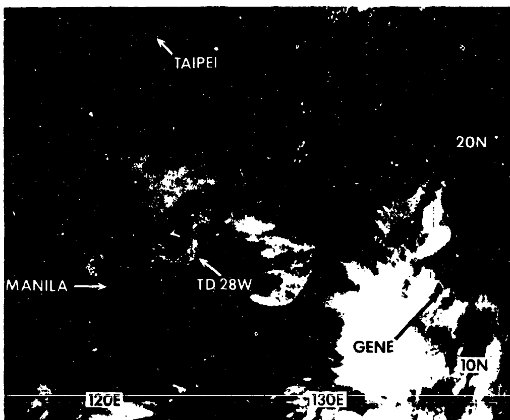
Figure 3-28-1 The exposed low-level circulation center of TD 28W is visible to the east of the deep convection associated with the depression subsided after crossing Luzon 12 October (080424Z October visual DMSP imagery).
