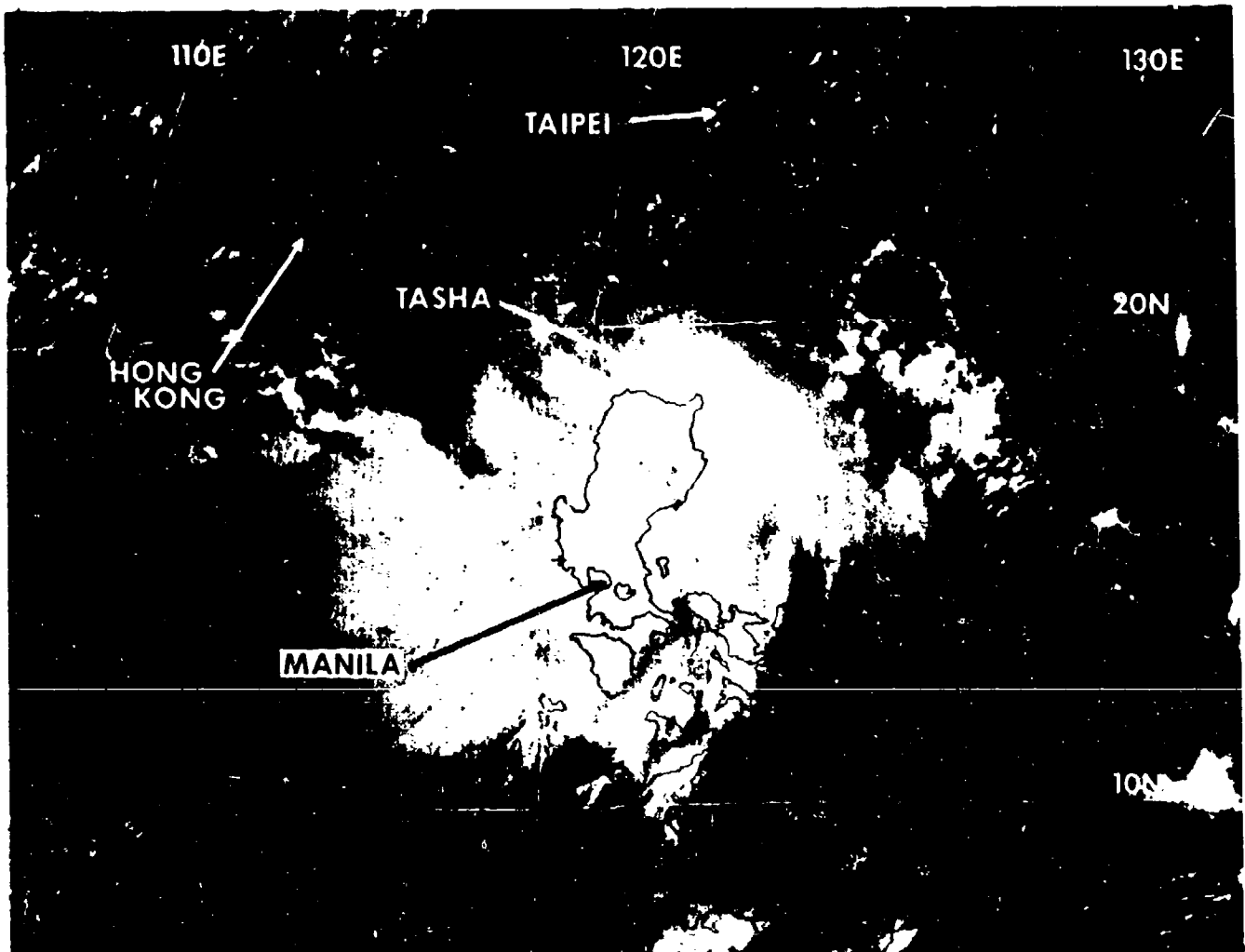
Figure 3-16-1 As Tasha passes north of Manila, bands of deep convection cover the island of Luzon (172331Z Augus: visual GMS imagery.)
