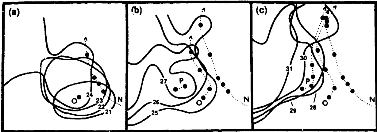
Figure 3-10-2 Illustration of the west-northwestward movement of the monsoon gyre of July 1993. a) The 1008, 1006, 1004 and 1004 mb contour of sea-level pressure (SLP) at 06Z July 21, 22, 23 and 24 respectively. b) The 1006 mb contour of SLP at 06Z July 25, 26 and 27. c) The 1006 mb contour of SLP at 06Z July 28, 29, 30 and 31. Dots show 06Z position of Nathan (N), Ofelia (O) and Percy (P) which show on each panel.
