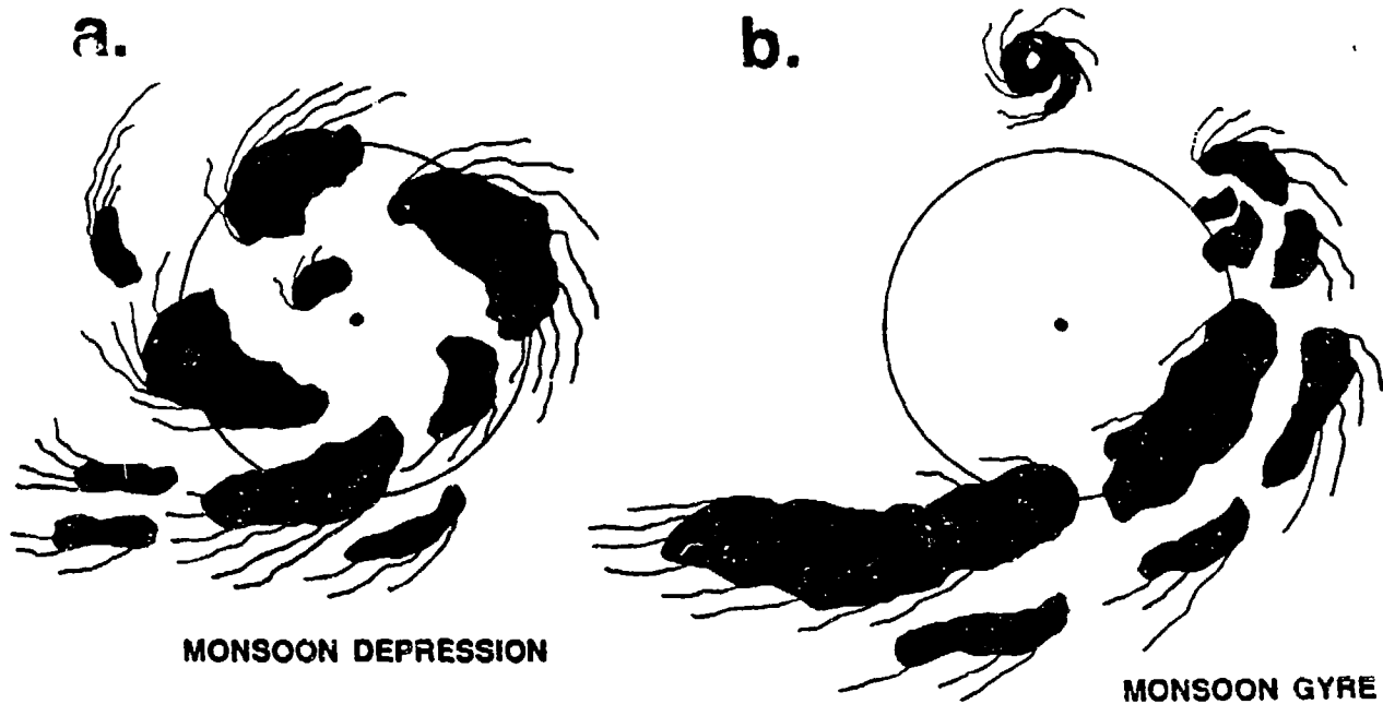
Figure 3-29-4 Schematic illustration of the distribution of deep convective cloud and cirrus in: a) a monsoon depression, and b) a monsoon gyre. Black areas represent deep convection, and filaments indicate orientation of cirrus plumes. Circle enclosed area of lowest sea-level pressure and has a diameter of approximately 600 nm (1110 km). The black dot is the low-level circulation center.
