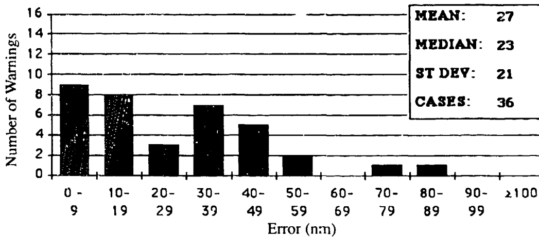
Figure 5-5a Frequency distribution of initial warning position errors (10-nm increments) for the North Indian Ocean in 1993. The largest error, 85 nm, was on TC02B.
