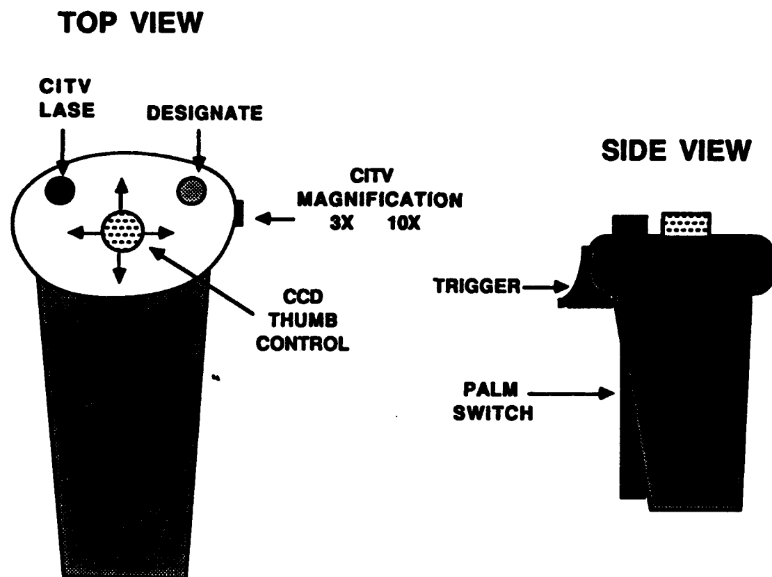
Figure 9. Drawing of the commander's control handle with functions labeled
