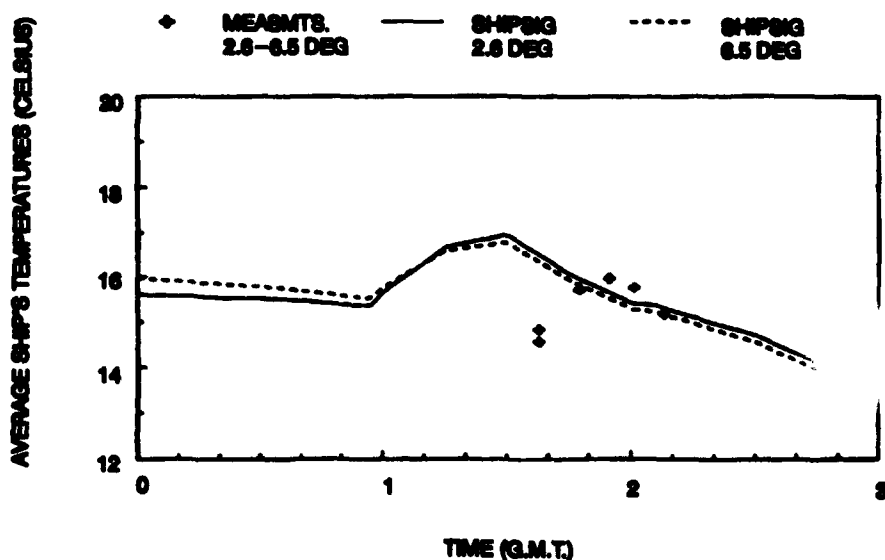
Figure 10. Comparison of measured average ship's temperatures (starboard side) and those calculated by SHIPSIG for the time period 0000 to 0300 G.M.T. on 4 August 1992 for different viewing angles.
