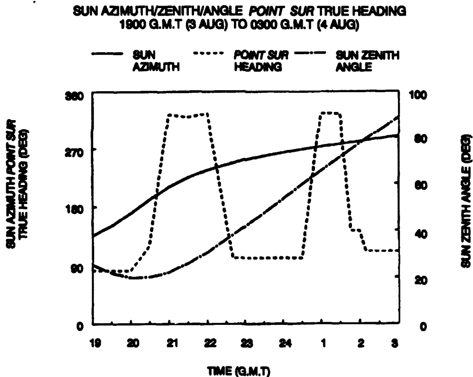
Figure 4. Heading of the R/V Point Sur and the sun's azimuth and zenith angle as functions of time on 3 and 4 August 1992.
