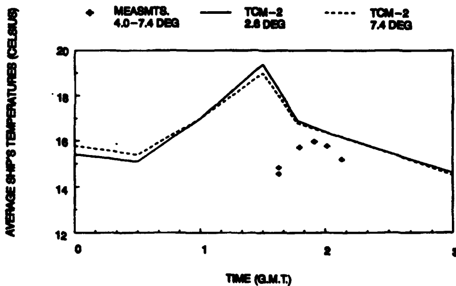
Figure 9. Comparison of measured average ship's temperatures (port side) and those calculated by TCM2 for the time period 0000 to 0300 G.M.T. on 4 August 1992 for different viewing angles.
