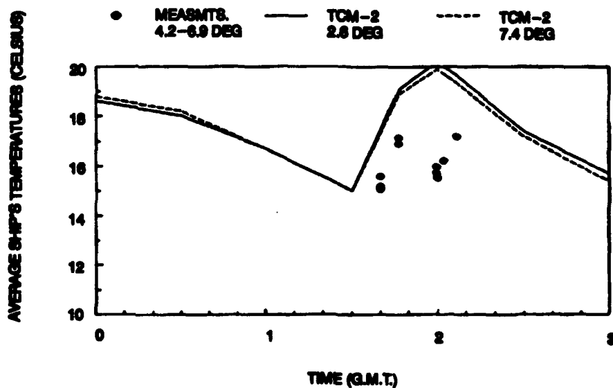
Figure 11. Comparison of measured average ship's temperatures (starboard side) and those calculated by TCM2 for the time period 0000 to 0300 G.M.T. on 4 August 1992 for different viewing angles.
