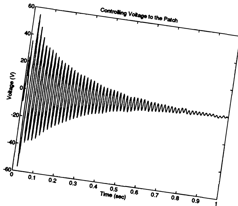
Fig. 5. The controlling voltage determined from (7).
