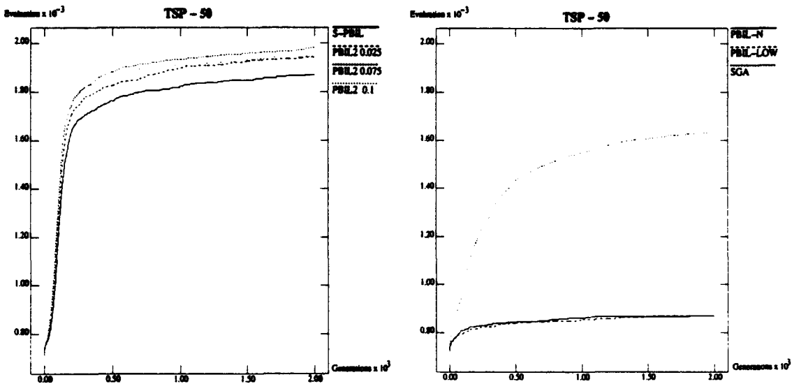
Figure 10: TSP, 50 City.
