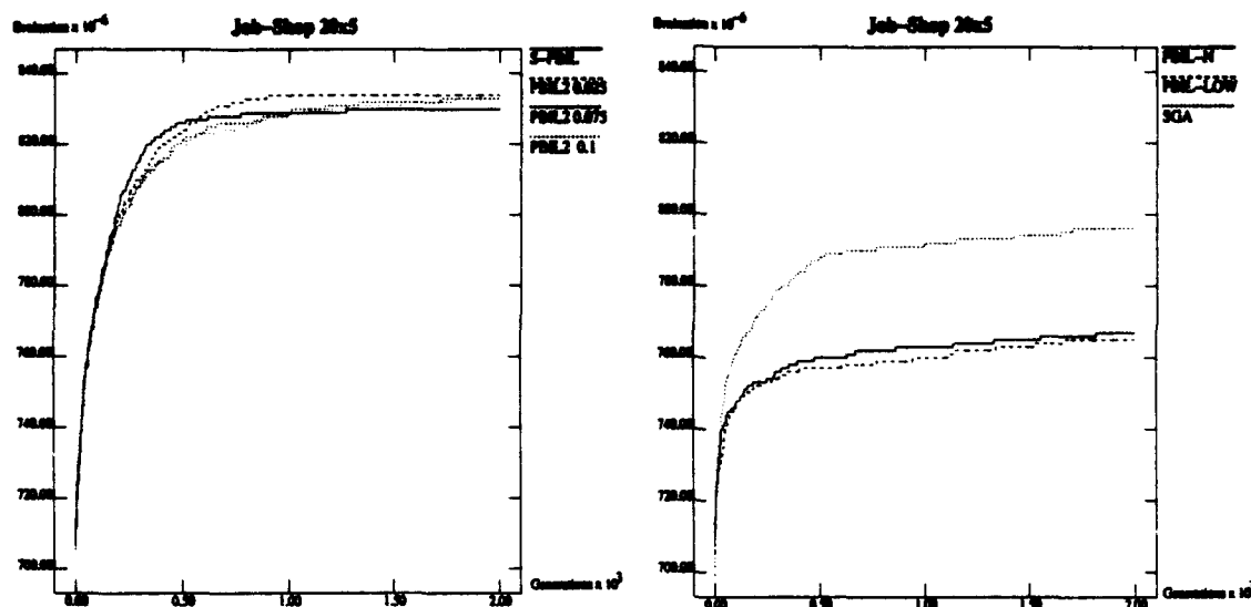
Figure 8: Job-Shop, 20x5
