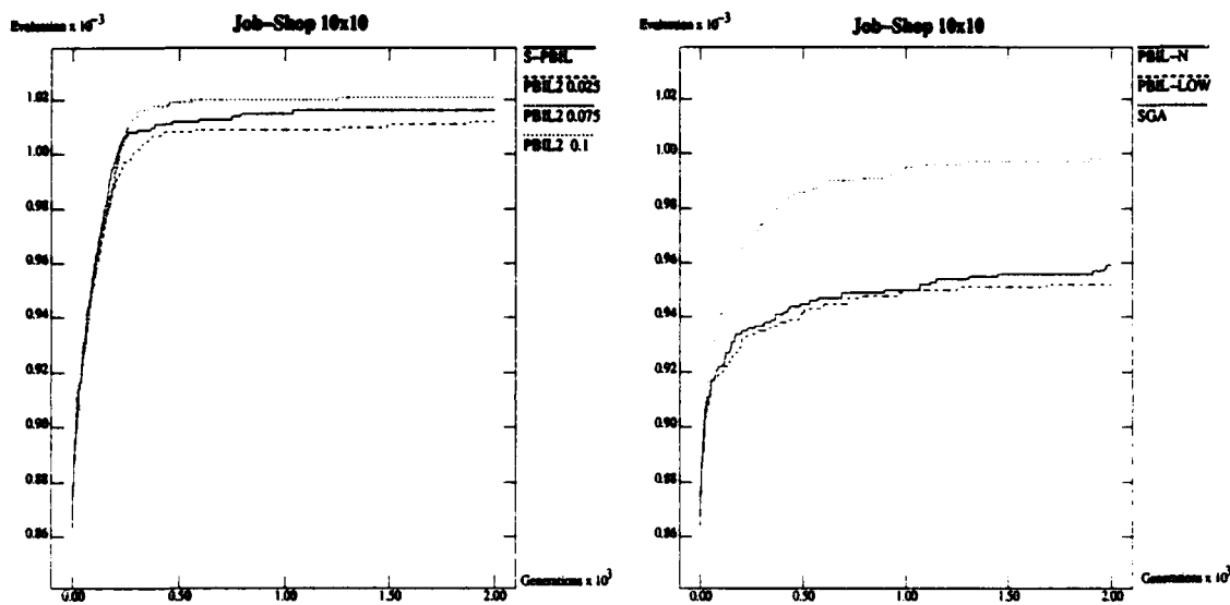
Figure 7: Job-Shop, 10x10
