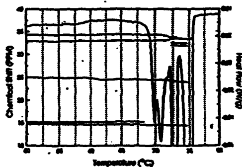
Figure 5 Correlation of peak chemical shift values from variable-temperature 13 C CP/MAS with DSC thermal transitions of the same sample treatment.
