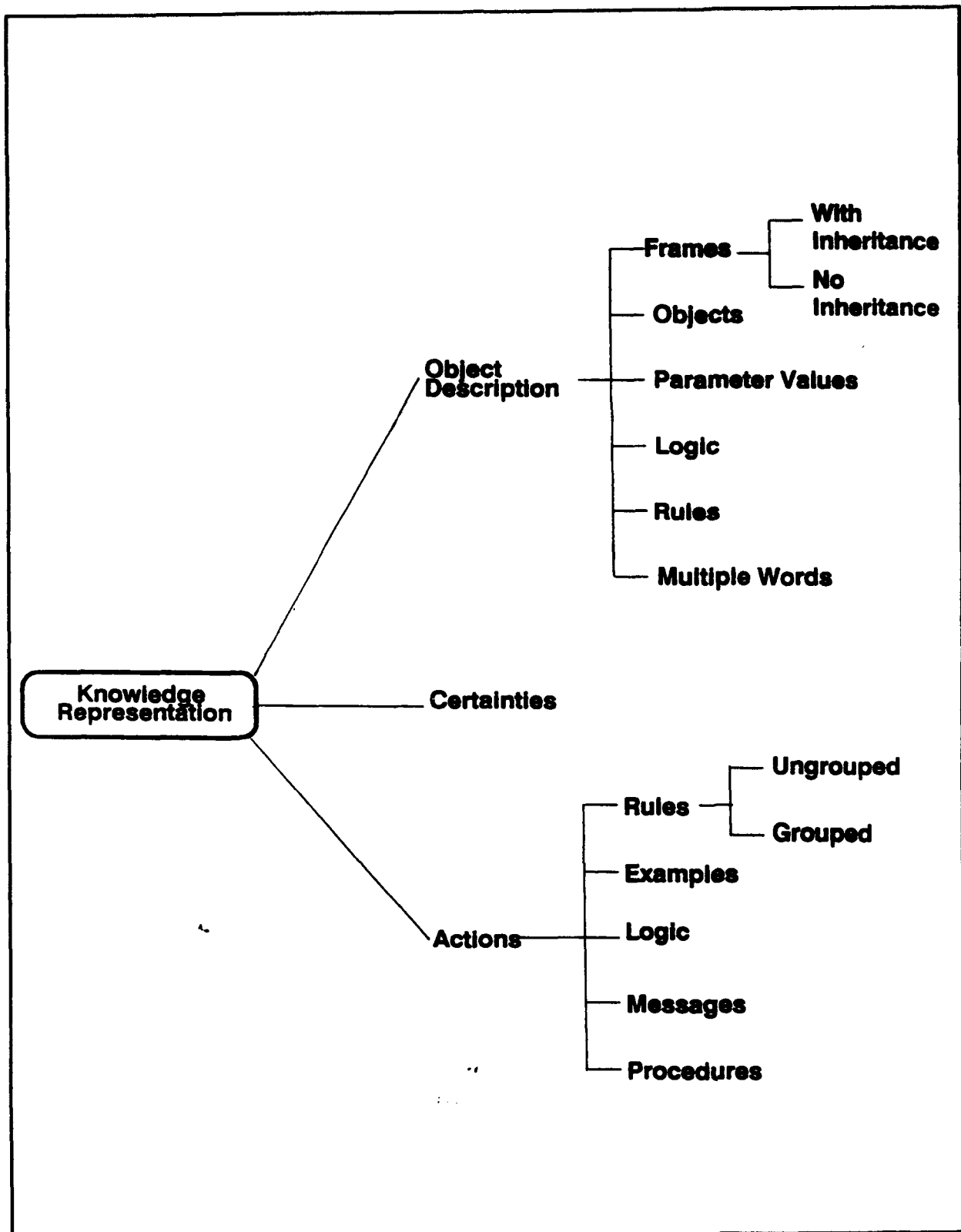
FIGURE 5.1.2-1. KNOWLEDGE REPRESENTATION
