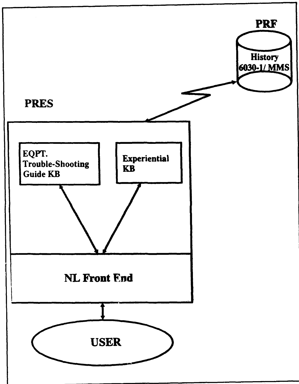
FIGURE 4.3.6.1.2-1. PROBLEM RESOLUTION EXPERT SYSTEM
