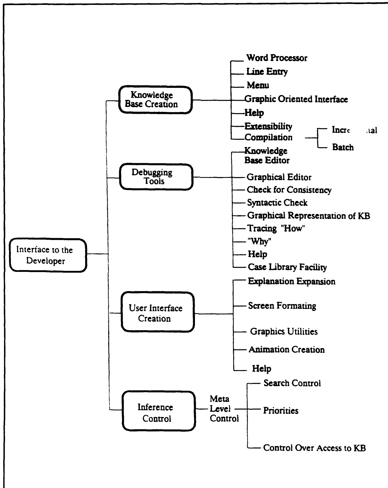
FIGURE 5.2.3.2-2. FEATURES OF A DEVELOPER'S INTERFACE TO AN EXPERT SYSTEM TOOL
