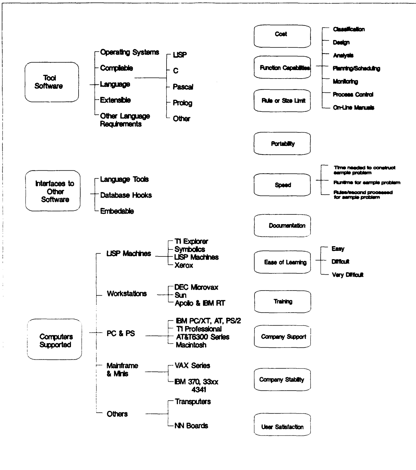
FIGURE 5.2.3.2-1. FACTORS FOR EXPERT SYSTEM TOOL SELECTION
