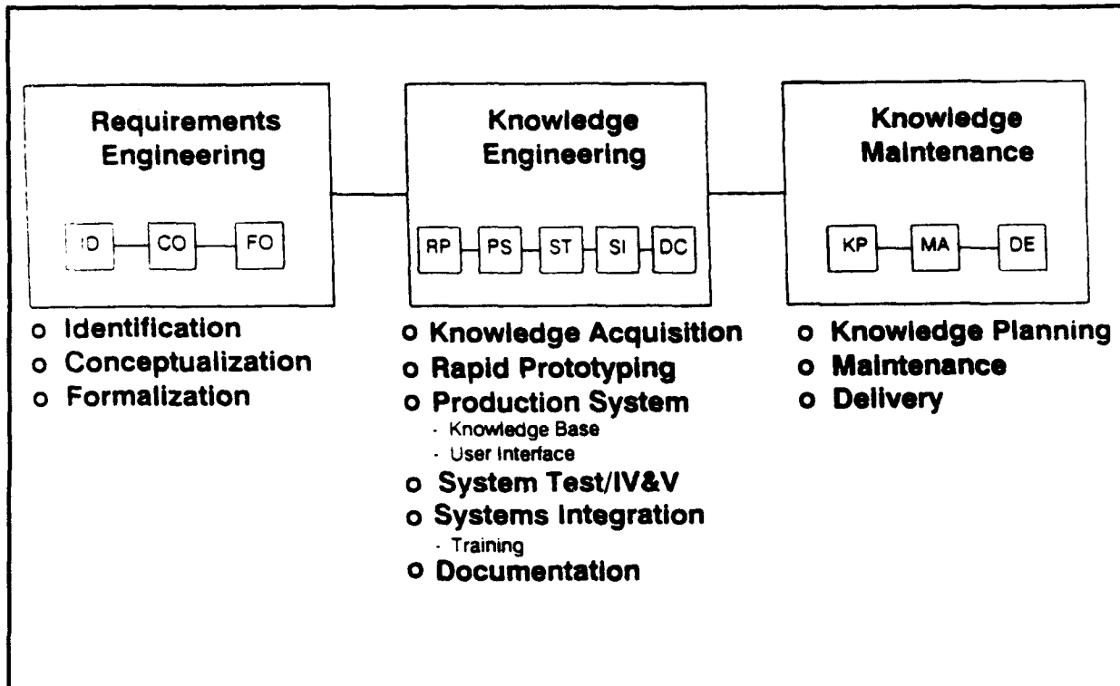
FIGURE 5.3.1-1. THREE MAJOR PHASES OF EXPERT SYSTEM DEVELOPMENT
