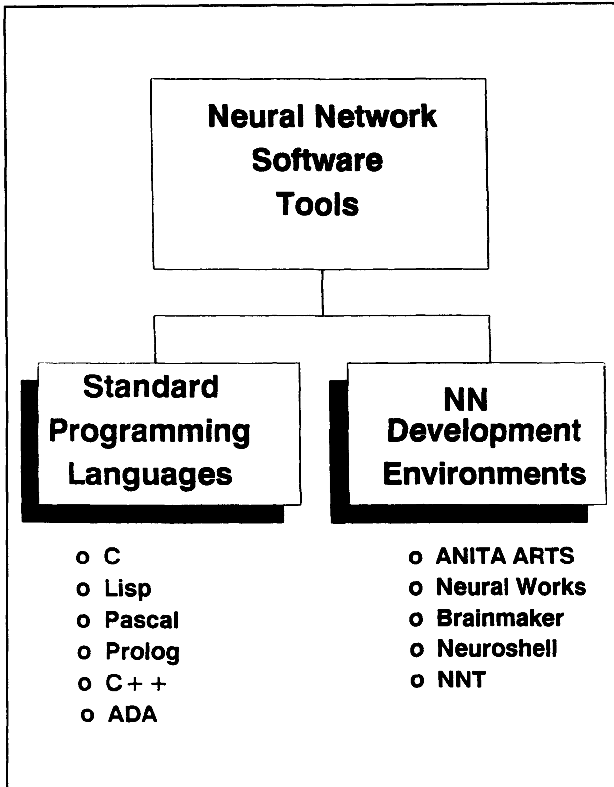
FIGURE 6.2.3.2-1. NN SOFTWARE
