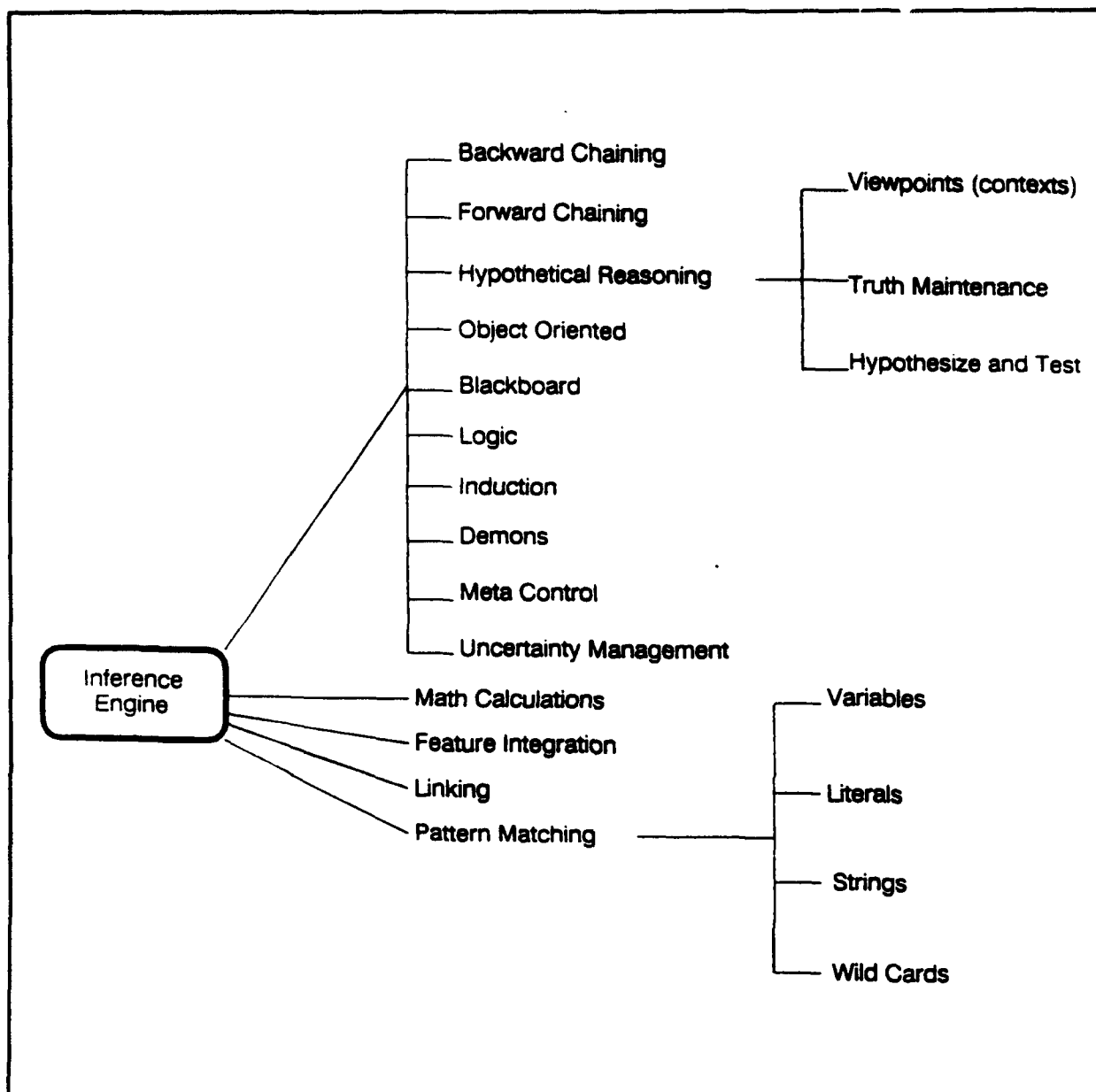
FIGURE 5.1.3-1. INFERENCE TECHNIQUES
