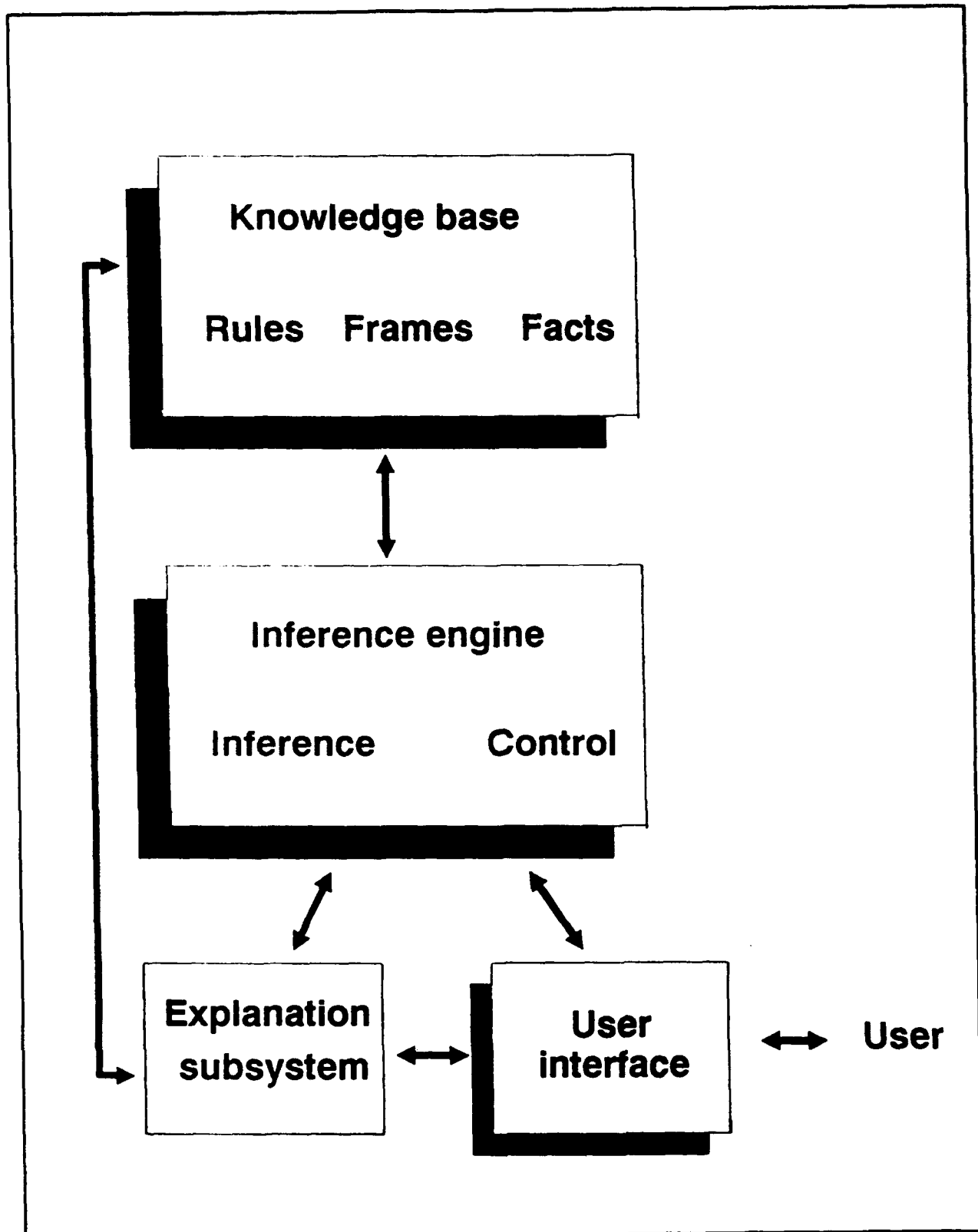
FIGURE 4.1.2-1 KNOWLEDGE-BASED EXPERT SYSTEM ARCHITECTURE
