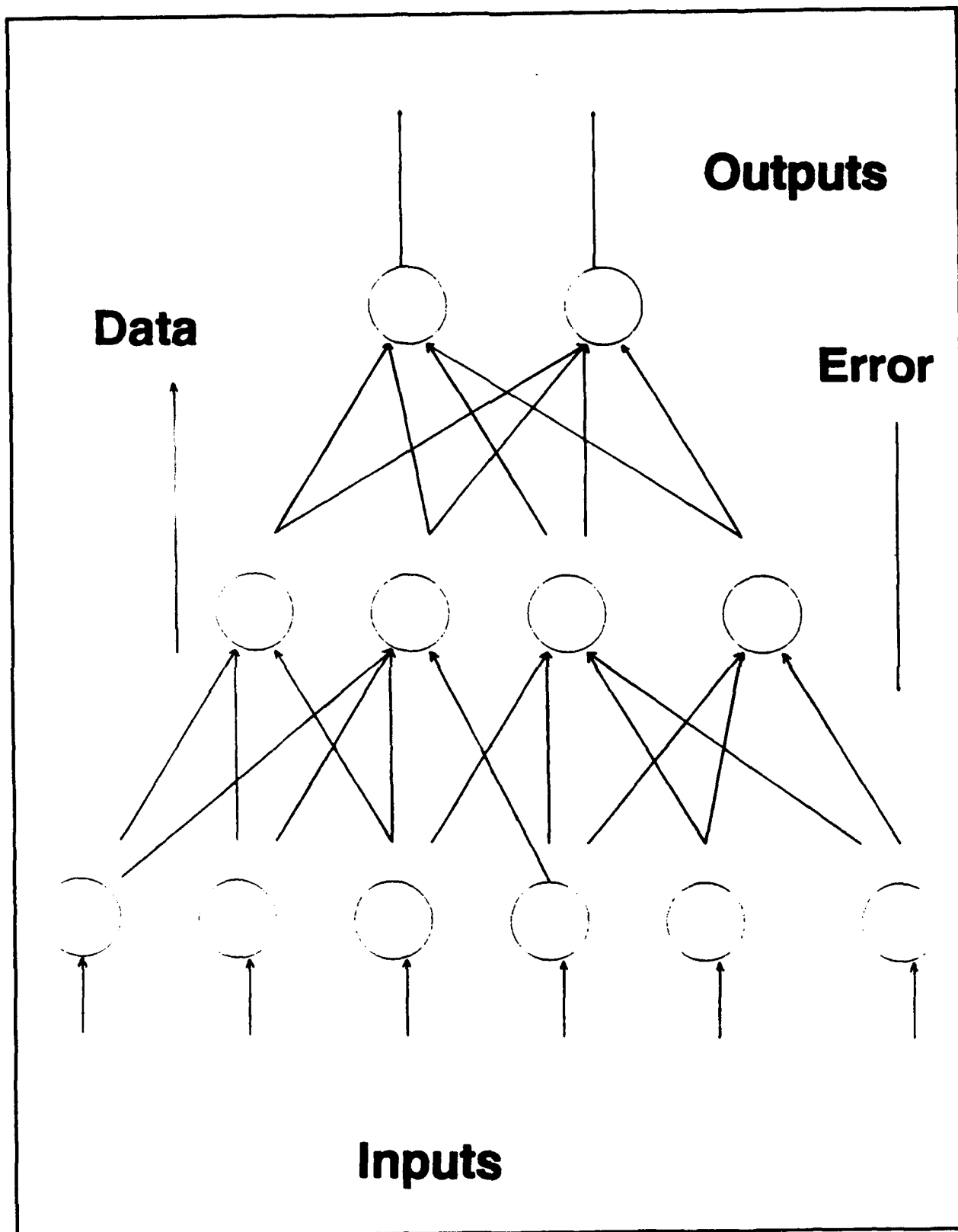
FIGURE 4.1.4-1. ANN ARCHITECTURE
