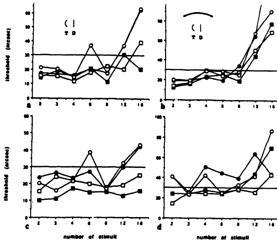
Fig. 17 Thresholds for the detection of a single curved target among straight distractors at eccentricities of 0.2^\circ (a,b) and 0.4^\circ (c,d). The stimuli were either oriented vertically (left column; a,c) or orientation varied by \pm 20^\circ (HW; circles) or 30^\circ (AH; squares) relative to the vertical (right column; b,d). For each condition, thresholds were measured both with (line symbols) and without subsequent mask (solid symbols). Results of two observers.
