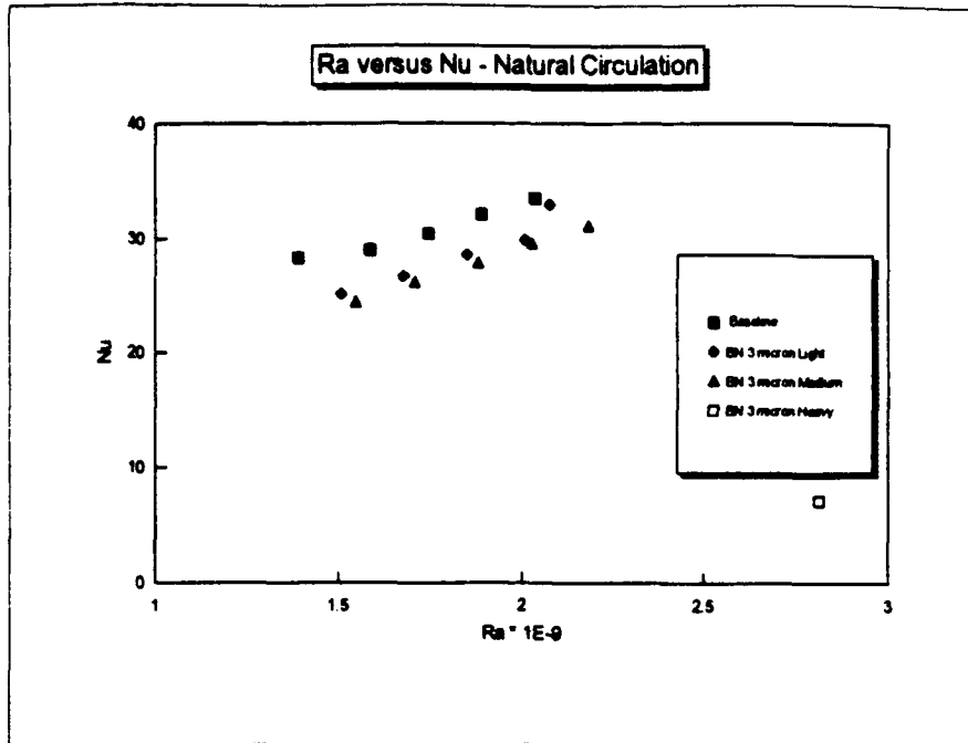
Figure 3-17: Ra versus Nu for 3 micron BN
