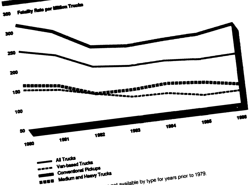
Figure IV.8: Truck Fatality Rates by Type of Truck a
