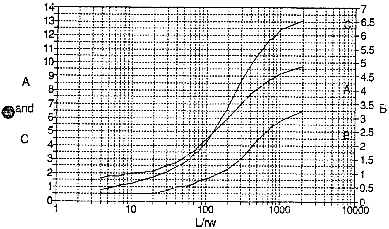
CECRL09 Curves Relating Coefficients A, B, and C to L/rw
