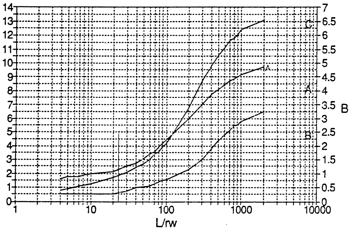
CECRL07 Curves Relating Coefficients A, B, and C to L/rw
