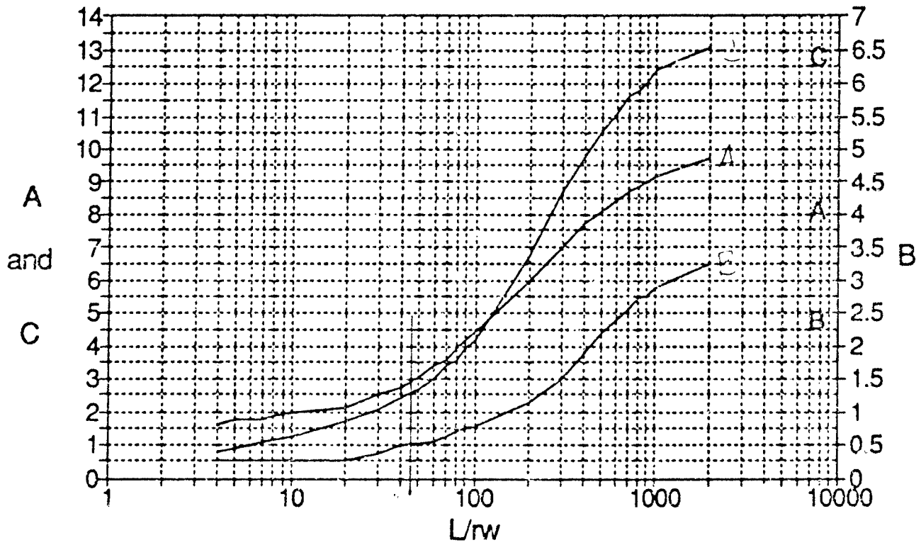
CECRL12 Curves Relating Coefficients A, B, and C to L/rw
