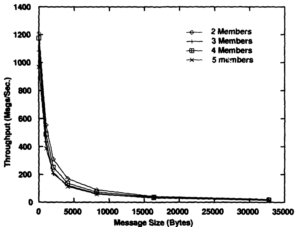
Figure 16: IP Multicast Asynchronous Cbcast Throughput in Msgs/Sec.
