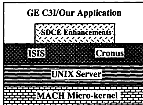
Figure 4. SDCE Architecture 2.
