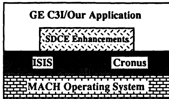
Figure 3. SDCE Architecture 1.
