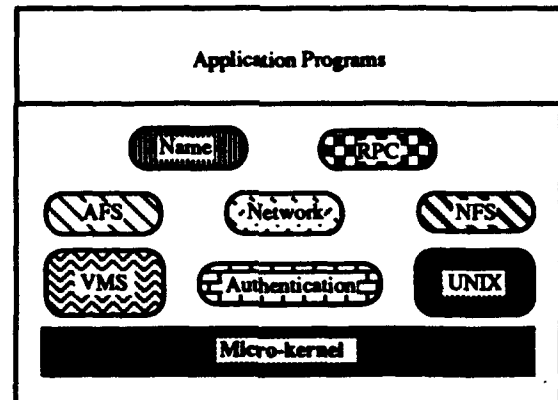
Figure 1. Micro-kernel Architecture.
