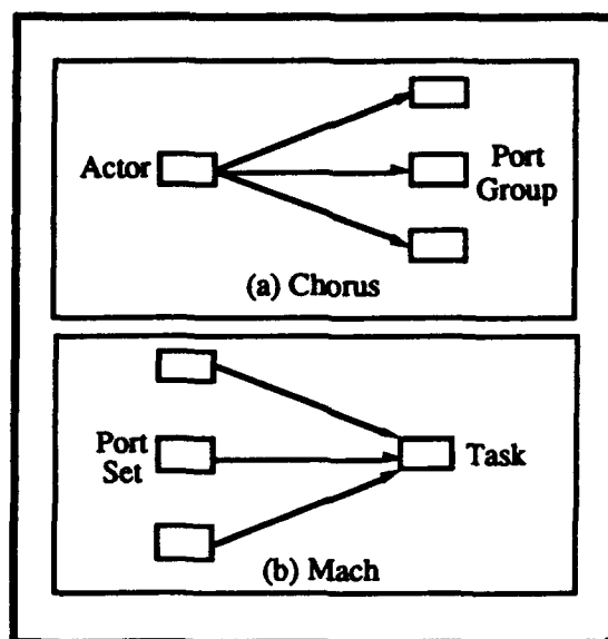
Figure 2. Send/Receive Semantics.
