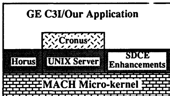
Figure 5. SDCE Architecture 3.
