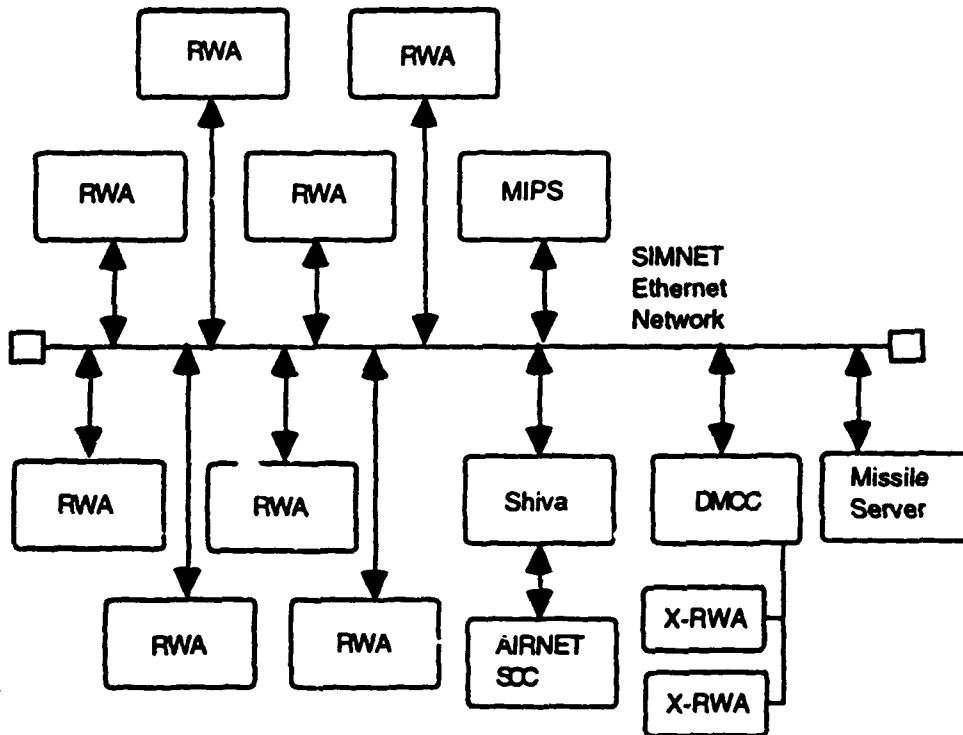
Figure 4.0 - 1 Required System Components
