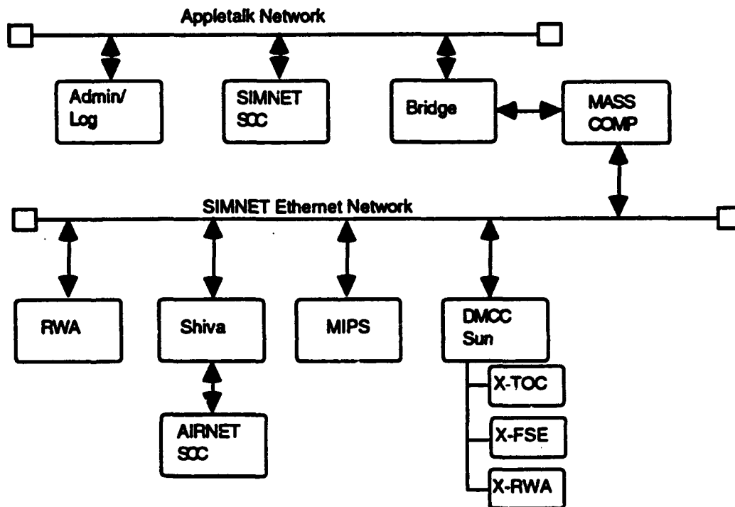
Figure 4.1 - 1 Required System Components
