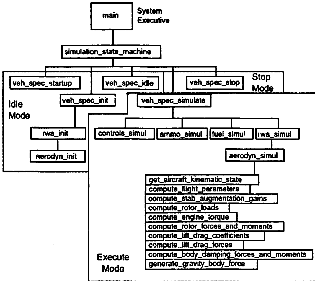
Figure 1: Flight Model Execution Software Path
