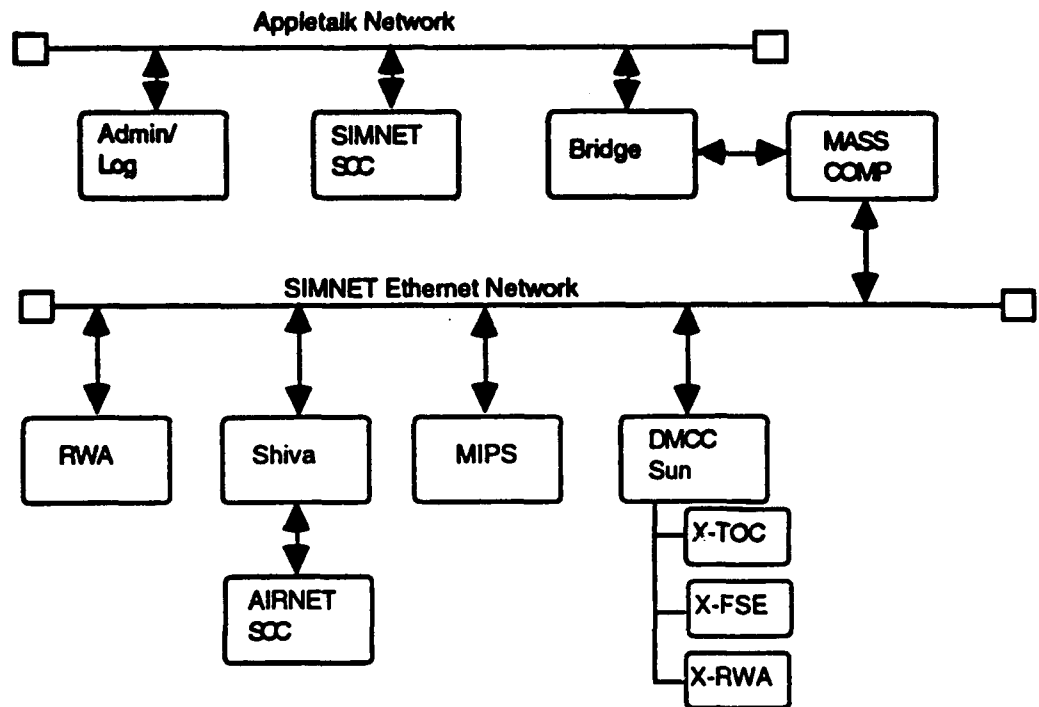
Figure 1 - 1 AIRNET Functional Configuration
