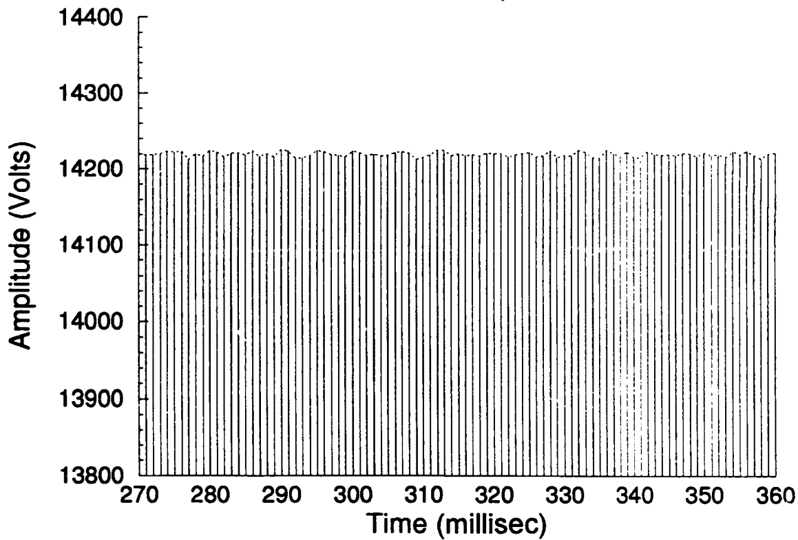
Figure 6b. Amp vs. Time for Staggered PRF MTS (no Doppler).
