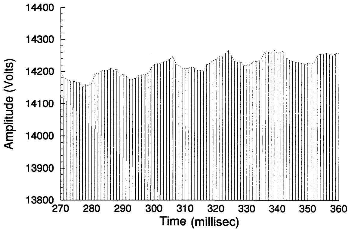
Figure 6a. Amp. vs. Time for Staggered PRF MTS (no Doppler).
