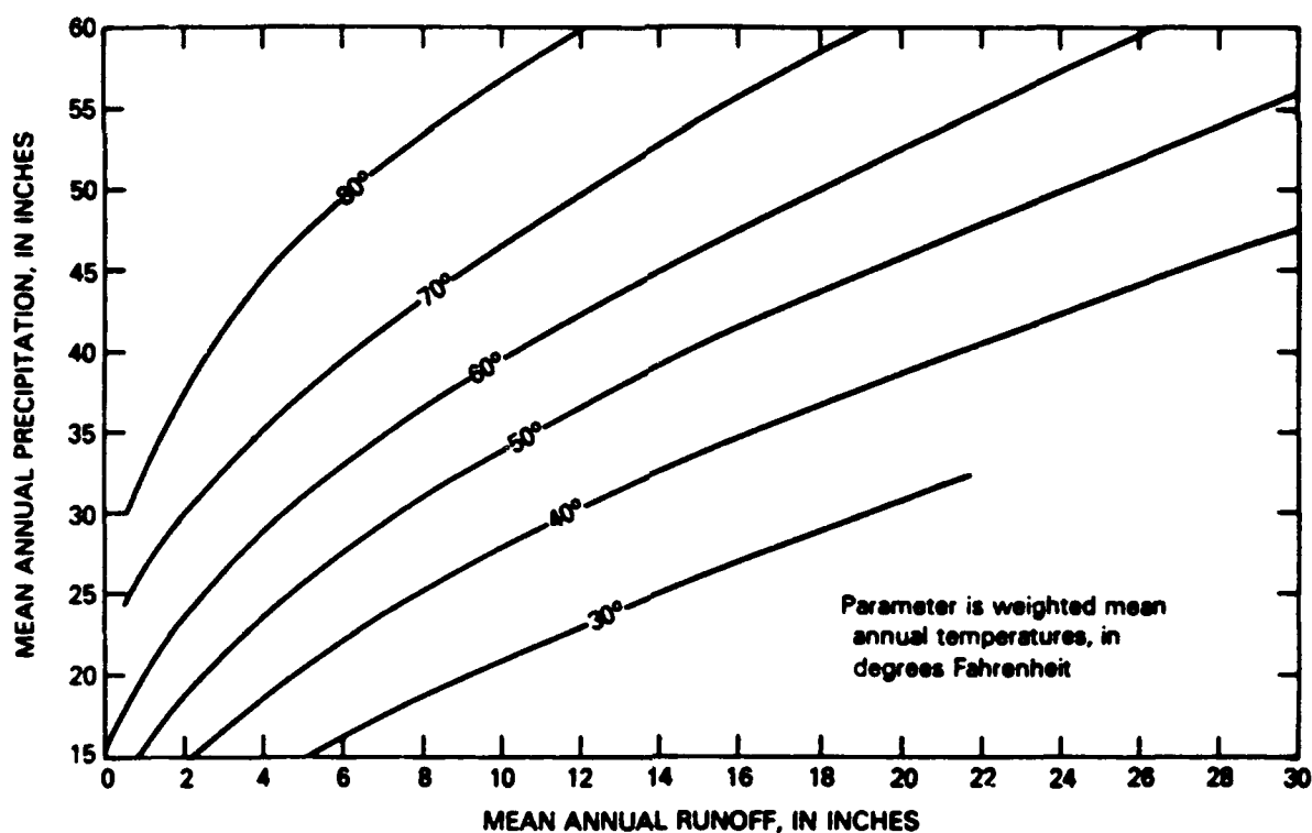
Figure 1. Relationship of annual runoff to precipitation and temperature.
