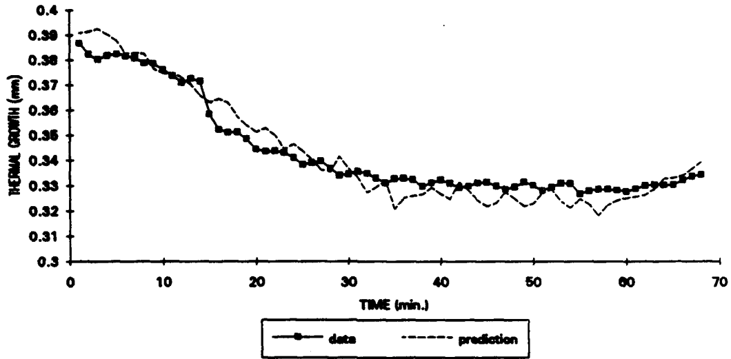
THERMAL GROWTH PREDICTION IN Z-AXIS (9000 rpm, cool-start)
