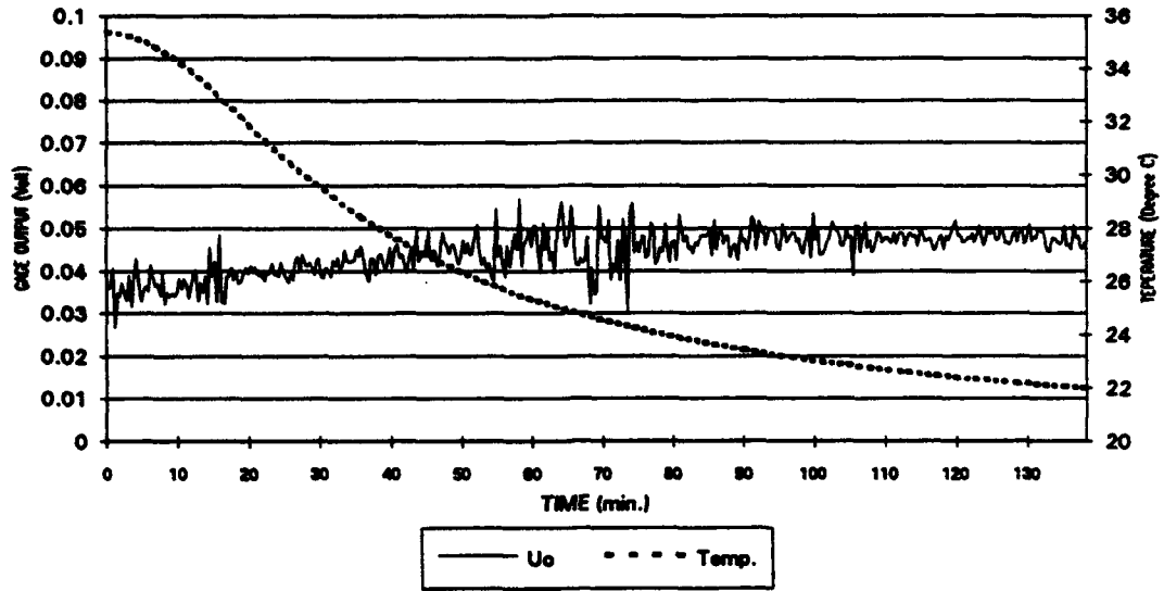
Figure 7. Thermal Drift Test Results of an API Capacitance Gauge
