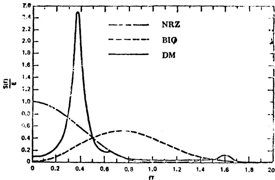
Figure C-1. Spectral Density of Random NRZ, BIØ, and DM Coding
