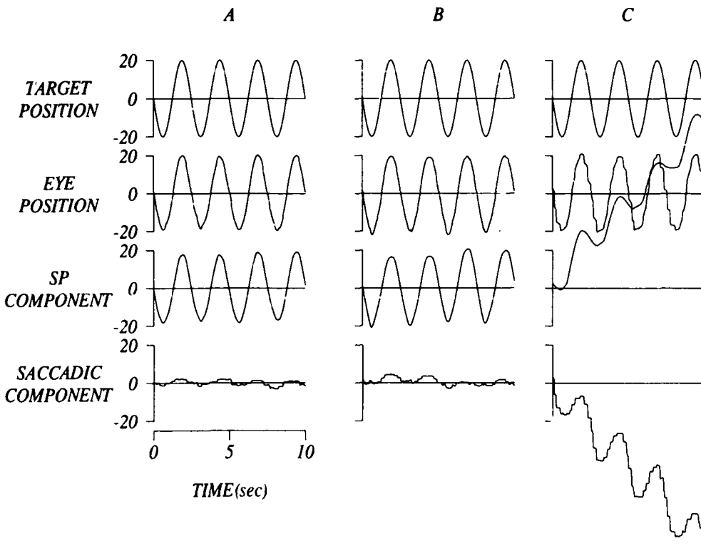
Fig. 3. Tracking record of a normal subject is shown in (A); tracking records for the patients discussed in Case Reports 1 and 2 are presented in (B) and (C), respectively. The eye position trace represents the combined tracking response and is the sum of the SP and saccadic components. Units of measurement are degrees of movement.
