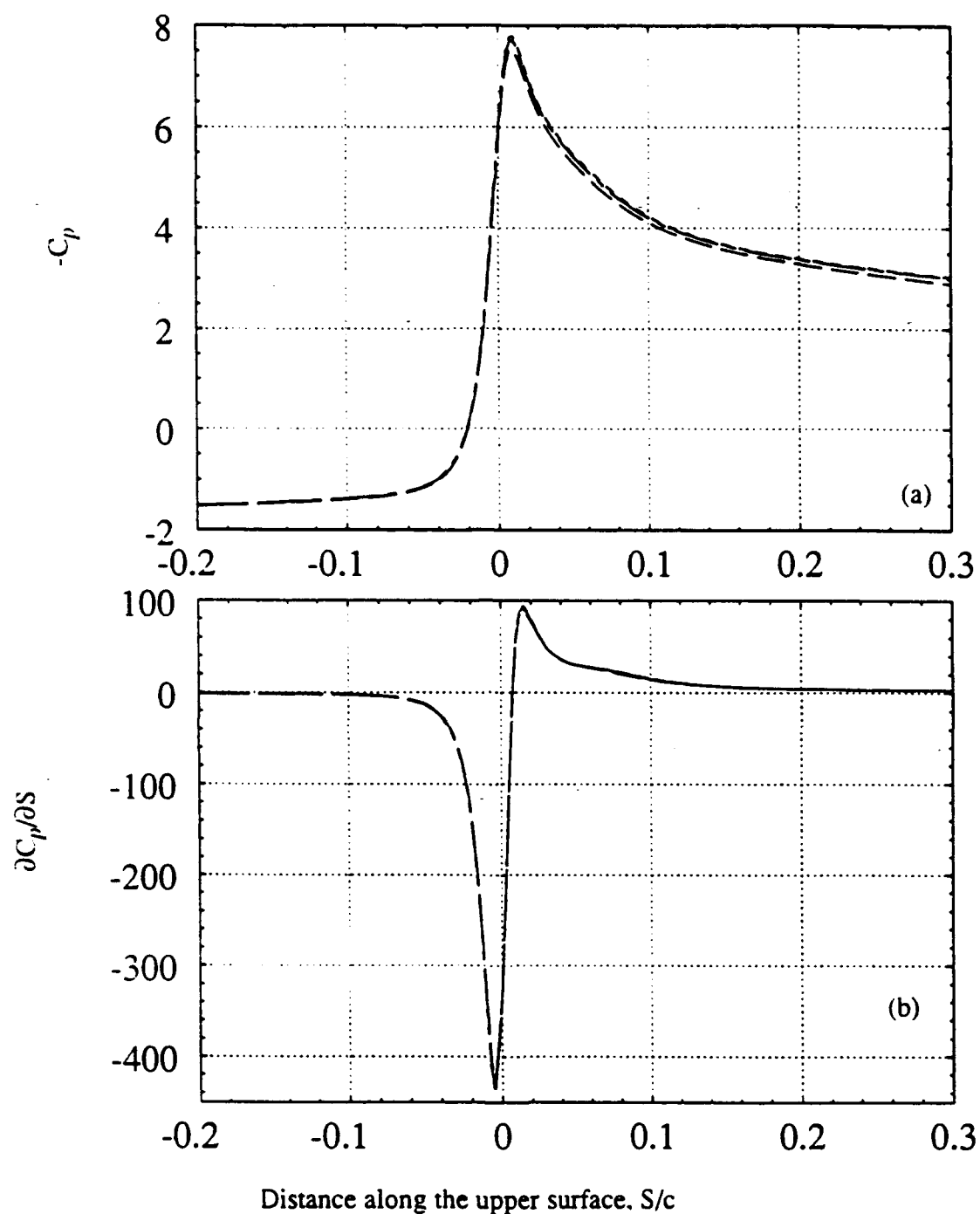
Figure 11. a) Surface pressure and b) surface pressure gradient profiles just before the onset of leading edge separation ( 22^\circ ), \Omega^* = 0.4 . ..... e = 0.039 , ..... e = 0.15 , and ---- e = 0.60 .
