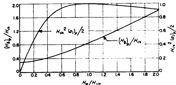
FIG. 1. Dependence of the location (H_s)_p and height (a_1)_p of the observed peaks on modulation amplitude.
