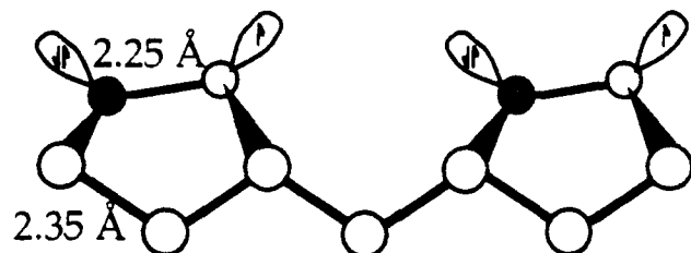
Si-P dimer
