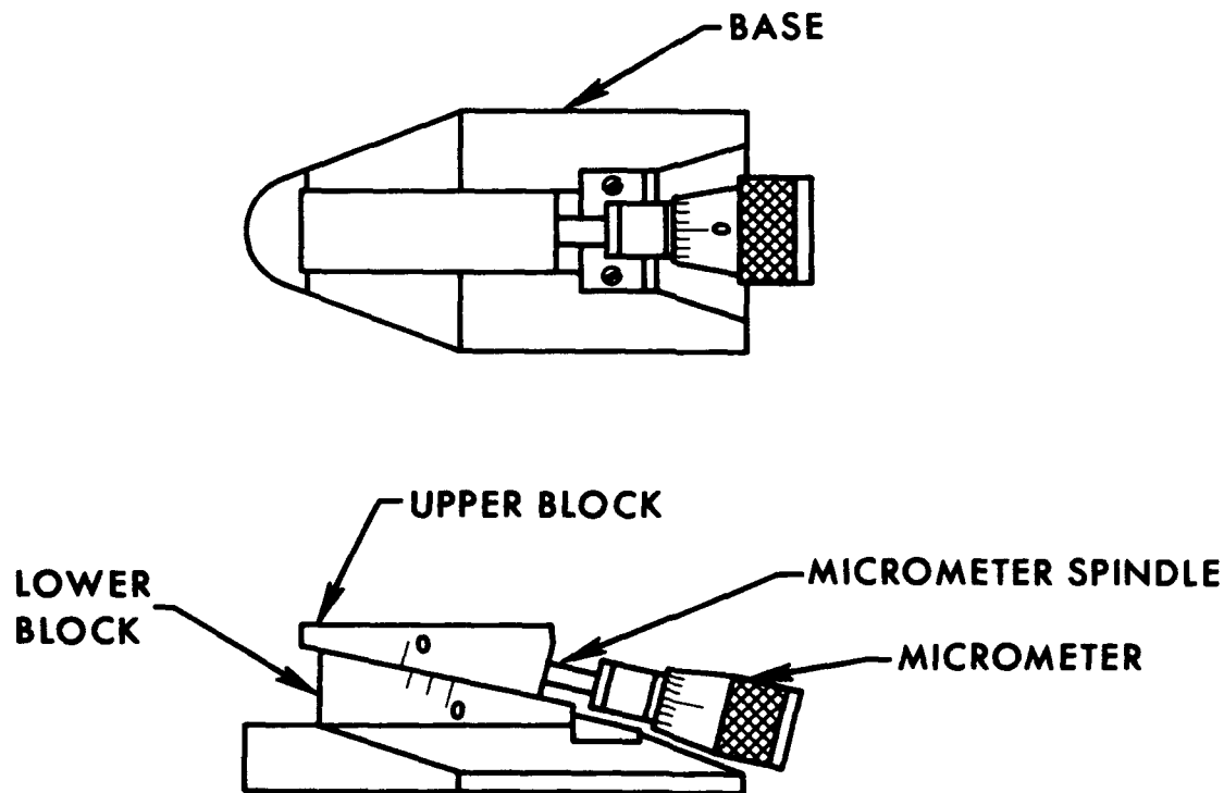
Figure 2. Two-view sketch of gage.
