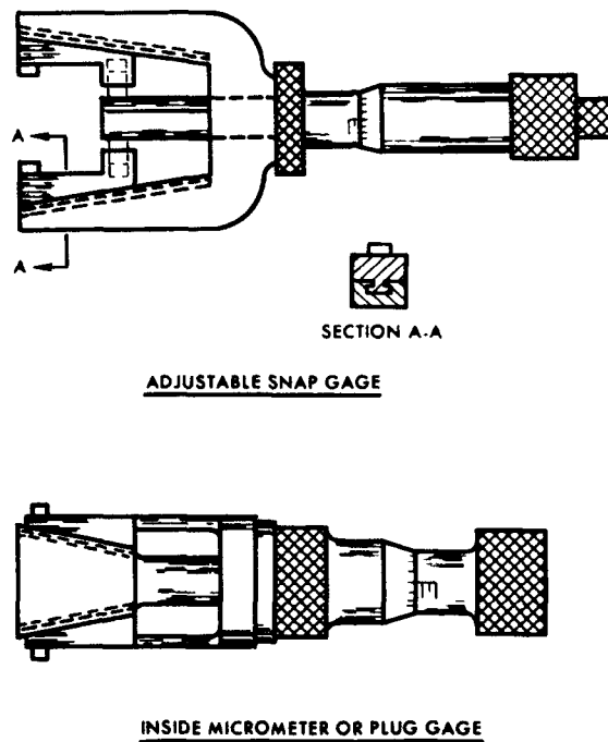
Figure 3. Possible variations of sliding-wedge principle.
