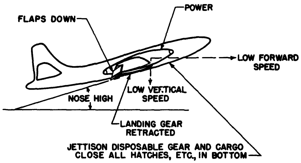
Figure 1. - Landing configuration.
