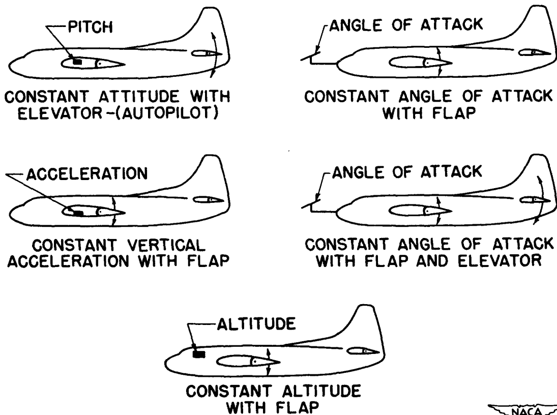
Figure 2. - Possible detector-servo systems for reducing gust loads.
