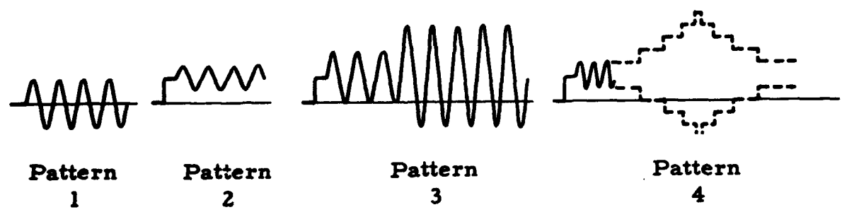
Figure 2. - Typical load patterns on airplane and on fatigue machines.
