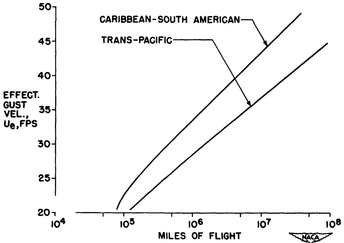
Figure 6. - Effect of route on gust frequency.
