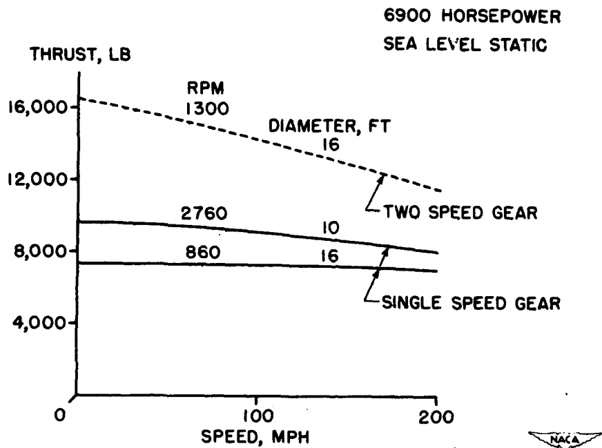
Figure 4. - Variation of thrust with airspeed in take-off.
