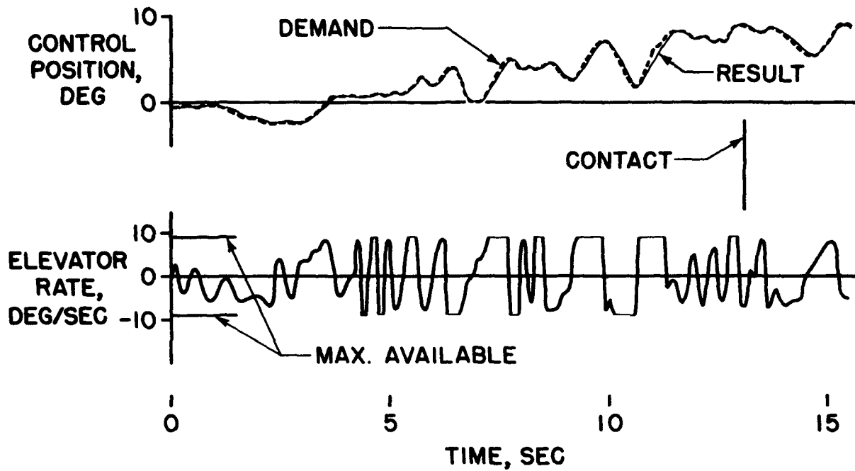
Figure 3. - Time history of a landing made with restricted elevator rate.
