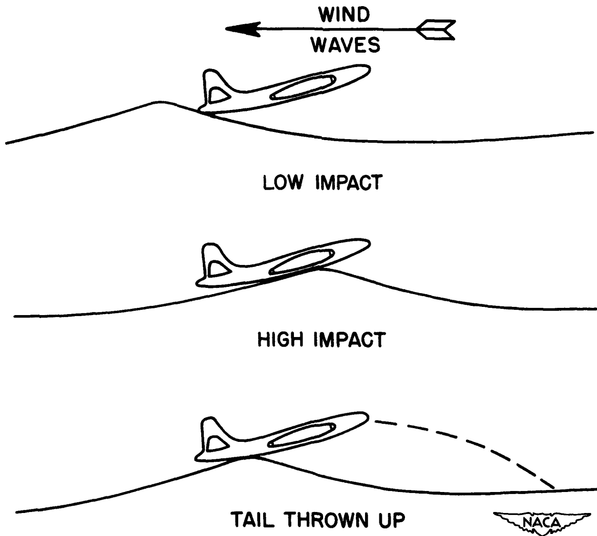
Figure 4. - Across waves.
