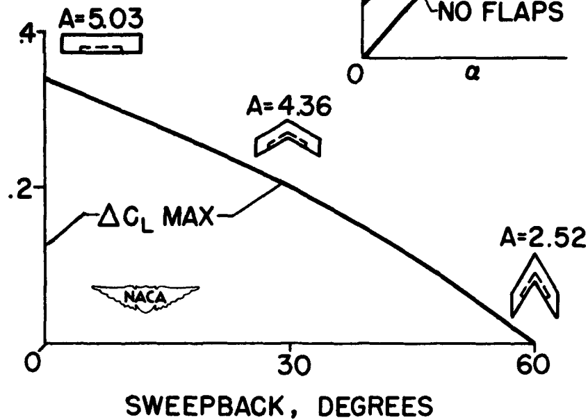
Figure 9. - Increment at various angles of sweepback of maximum lift due to flaps.
