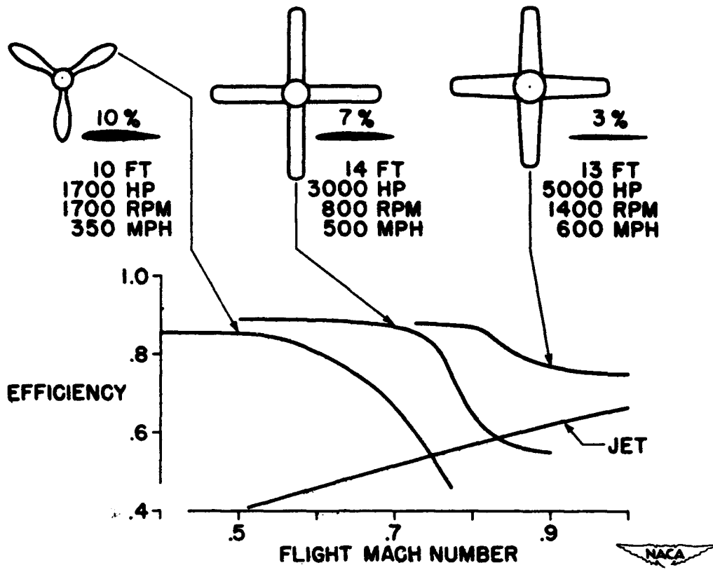
Figure 1. - Variation of efficiency with flight Mach number for three different propeller types.
