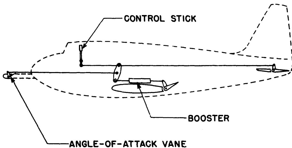
Figure 5. - Diagram of mechanism for vane-type acceleration alleviator.
