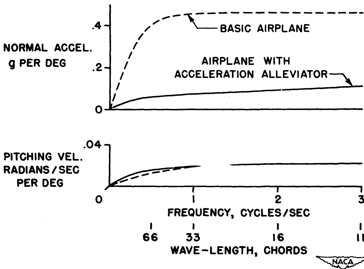
Figure 6. - Response of an airplane equipped with acceleration alleviator to sinusoidal gusts of various frequencies. Characteristics of basic airplane shown for comparison.
