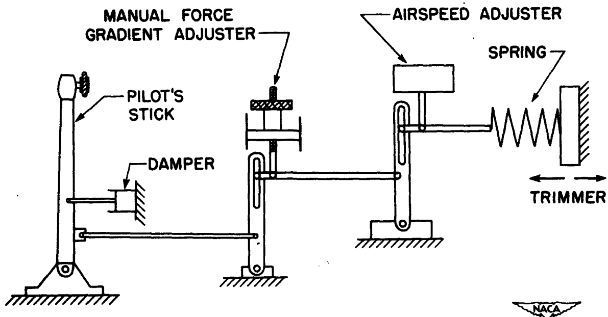
Figure 6. - Schematic drawing of feel device.
