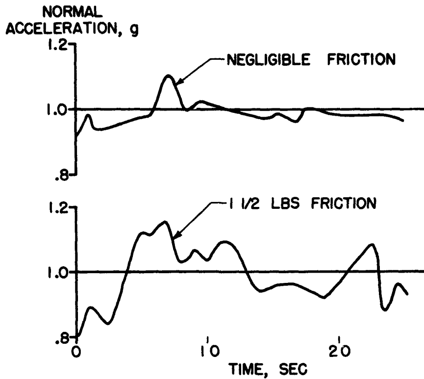
Figure 5. - Time histories of normal acceleration for two values of booster valve friction.
