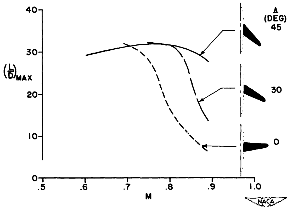
Figure 5. - Effect of sweep on the maximum lift-to-drag ratio.
