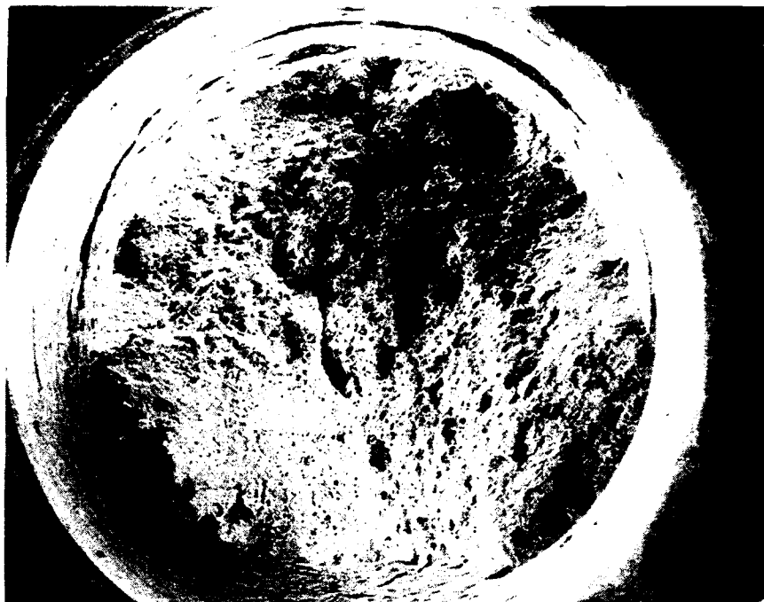
Figure 18 Low magnification scanning electron micrograph of the HY-100 heat affected zone showing the mixed mode behavior observed in failures contained in Region II of Figure 6. 100 \mu\text{m}
