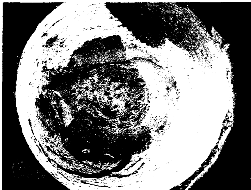
Figure 19 Low magnification scanning electron micrograph of the HSLA-100 heat affected zone showing the mixed mode behavior observed in failures contained in Region II of Figure 6. 100 \mu\text{m}
