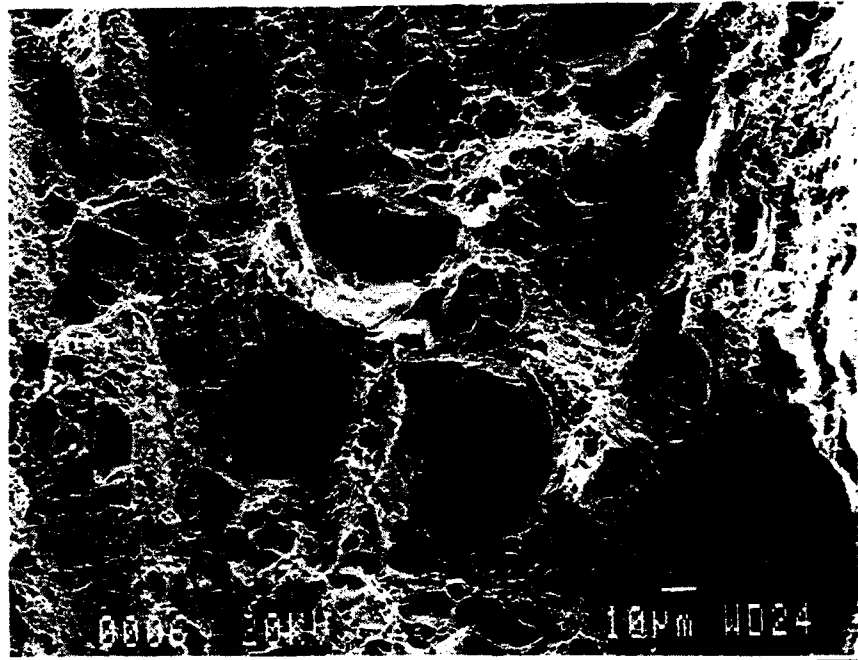
Figure 15b High magnification scanning electron micrograph from Figure 15a showing the general size and distribution of the observed microvoids.
