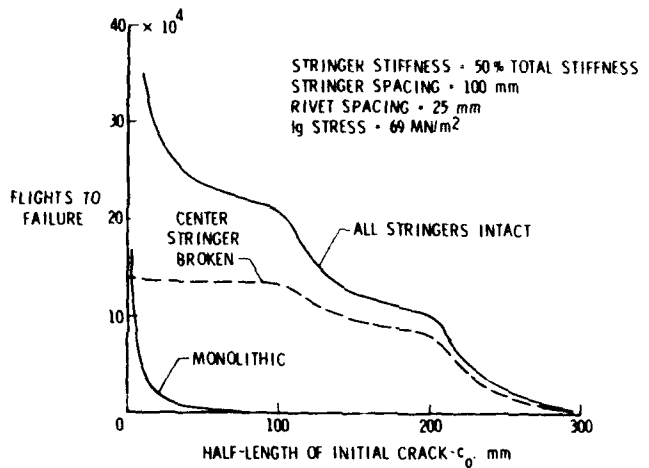
Figure 13. Crack propagation life for 7075-T6 aluminum alloy panels.
