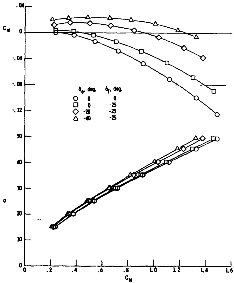
(a) Body axis.
