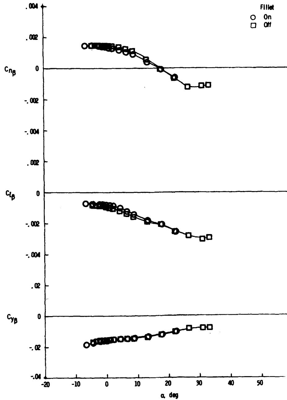
Figure 13. - Effect of planform fillet on lateral-directional stability characteristics of single fin version, center fin on (flared rudder), \delta_e = \delta_r = 0^\circ
