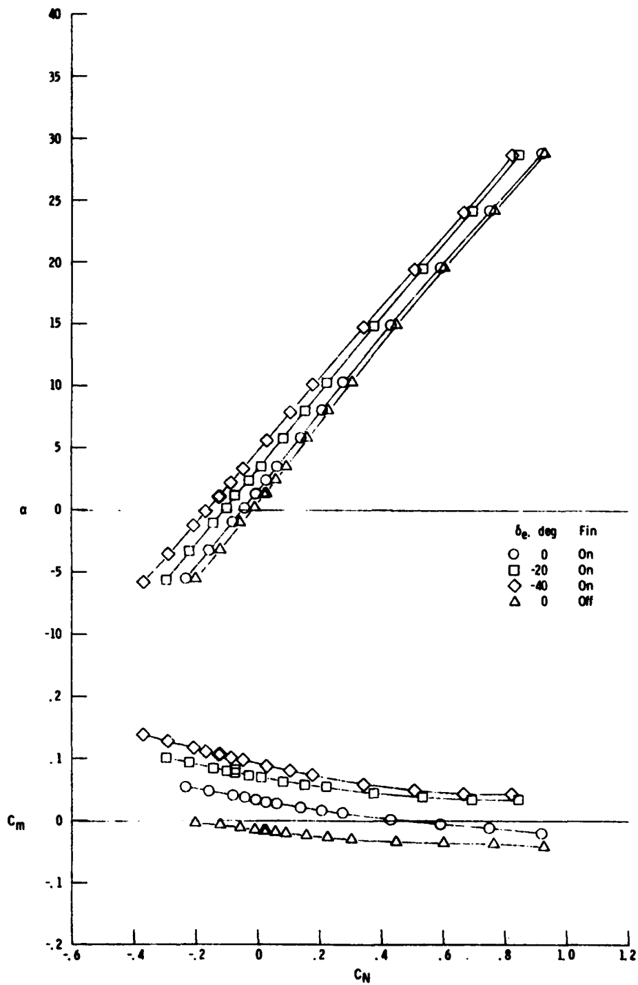
(c) M = 2.36 Figure 8 - Continued.
