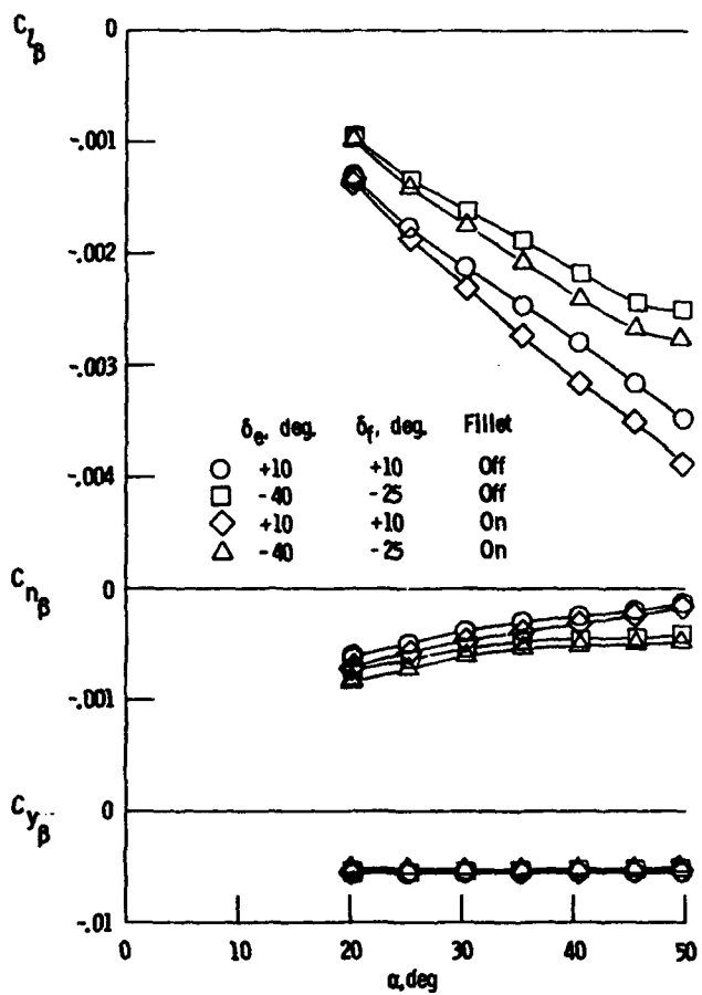
(b) Bent sting, center fin off.
