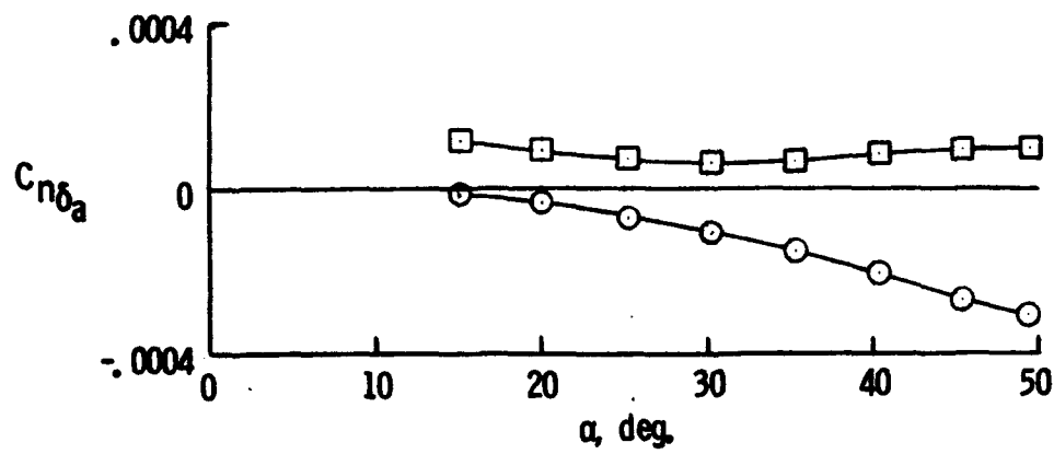
Figure 7. - Roll control effectiveness on twin fin version, \delta_a = 10^\circ . M = 10.3 .
