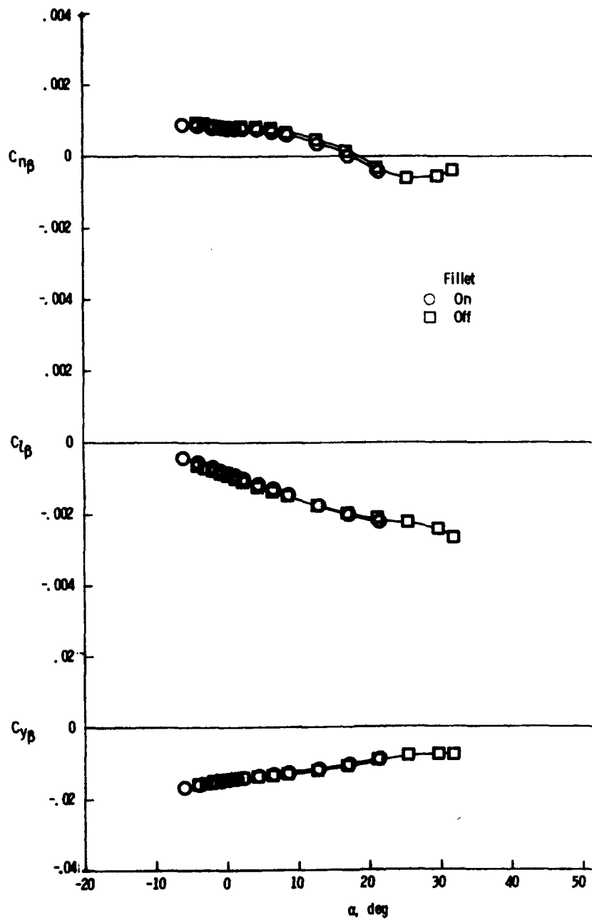
(c) M = 3.96 Figure 13. - Continued.
