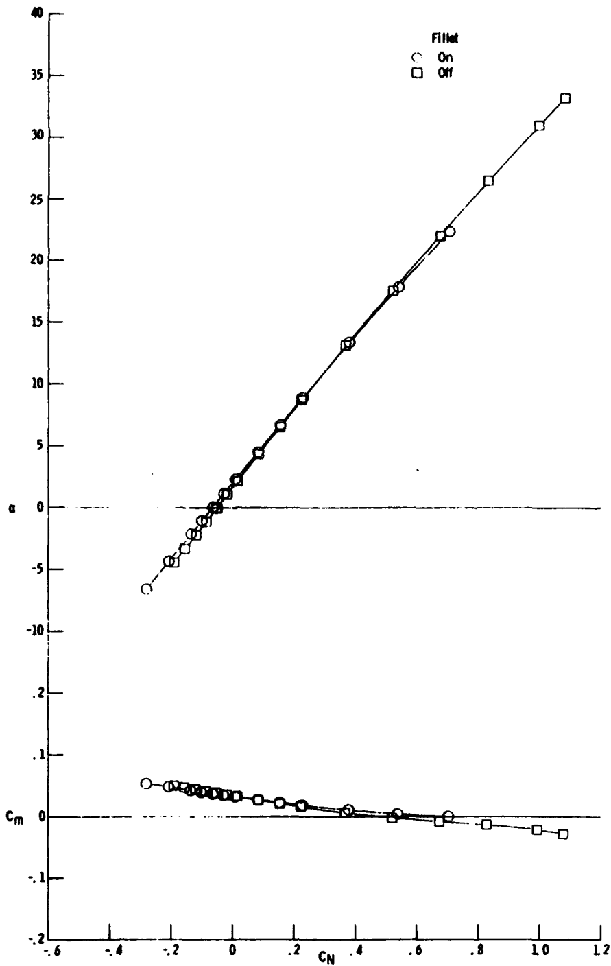
Figure 9. - Planform fillet effect on longitudinal stability characteristics of single fin version, rudder flared 30^\circ , \delta_\alpha = \delta_\gamma = 0^\circ .
